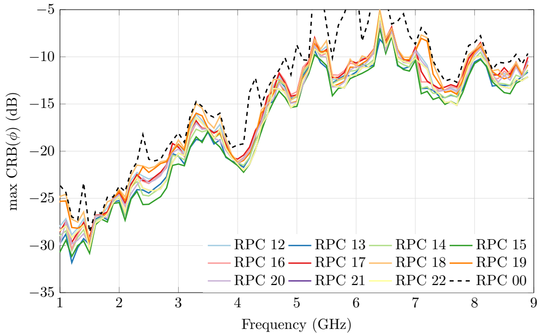
Figure H.13: Highest simulated CRLB( \phi ) of the Four Season VA using different RPCs [12 to 22] added to the RPC 00, and under the scenario conditions defined in Table 3.15 ( \gamma = 45^\circ † \eta = 0^\circ )
