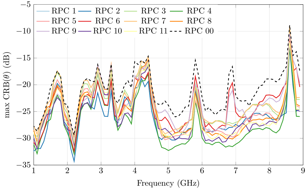
Figure H.6: Highest simulated \text{CRLB}(\theta) of the Four Season VA using different RPCs [1 to 11] added to the RPC 0, and under the scenario conditions defined in Table 3.15 ( \gamma = 90^\circ \uparrow \eta = 0^\circ , i.e. vertical polarization)
