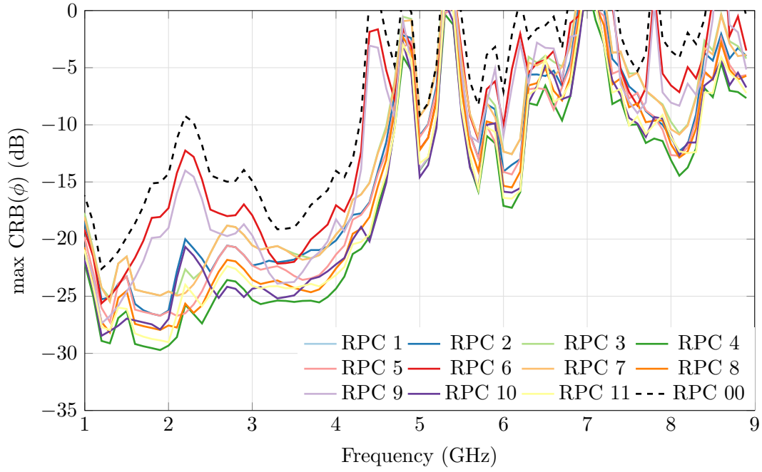
Figure H.4: Highest simulated \text{CRLB}(\phi) of the Four Season VA using different RPCs [1 to 11] added to the RPC 00, and under the scenario conditions defined in Table 3.15 ( \gamma = 90^\circ \dagger \eta = 0^\circ , i.e. vertical polarization)
