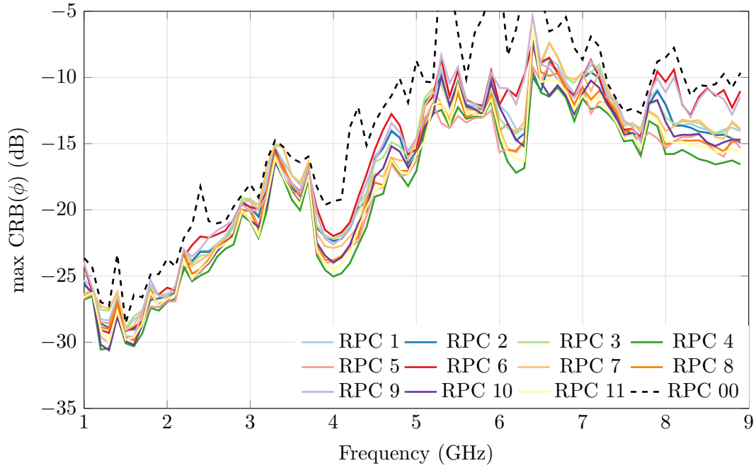
Figure H.12: Highest simulated CRLB( \phi ) of the Four Season VA using different RPCs [1 to 11] added to the RPC 00, and under the scenario conditions defined in Table 3.15 ( \gamma = 45^\circ † \eta = 0^\circ )
