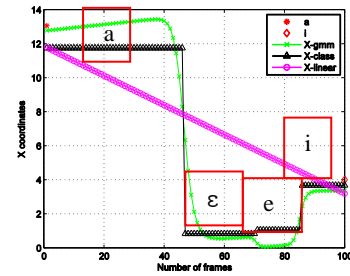
Figure 7: The dynamic transition of X coordinates of hand position by interpolation between the vowel [a] and [i]. Results with the multi-linear mapping (X-linear), the GMM mapping (X-gmm), and the gaussian classifier applied to the spectral space (X-class).
