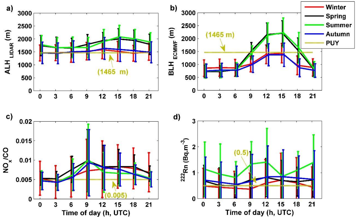
Figure 4.1. 2. The diurnal variation of the 3-h averaged parameters used to segregate between BL/AL and FT air masses as a function of the season: (a) ALH LIDAR ; (b) BLH ECMWF ; (c) NO x /CO, and (d) 222 Rn. Variability within each season indicates the standard deviation.
