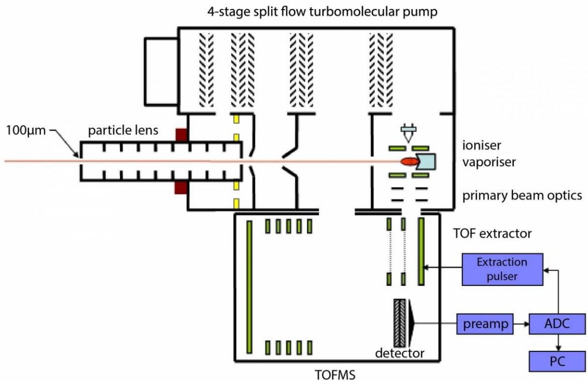
Figure 3. 3. ToF-ACSM schematic.
