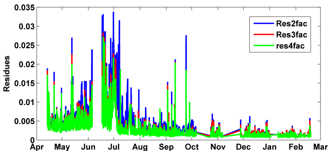
Figure 4.2. 8. Residues for: 2-, 3- and 4- factorial ME-2.
