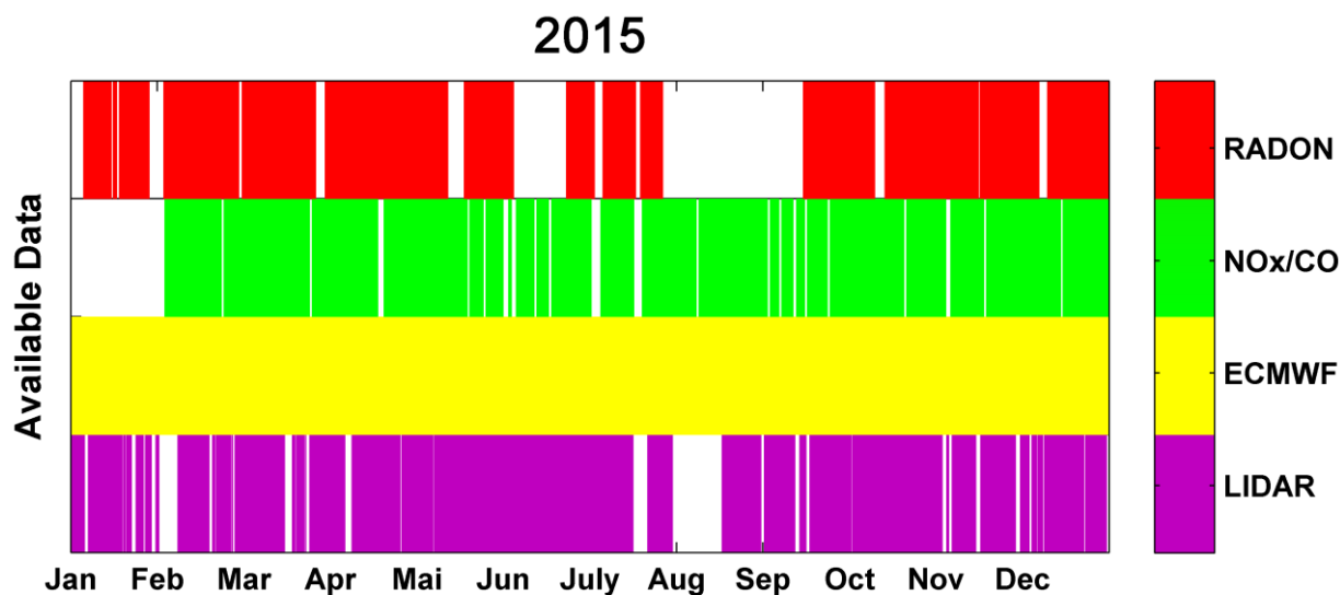
Figure 4.1. 1. Available data from the main instruments used in the determination of the boundary layer height. Red: Radon-222, Green: NO x /CO, Yellow: ECMWF, and Violet: LIDAR.
