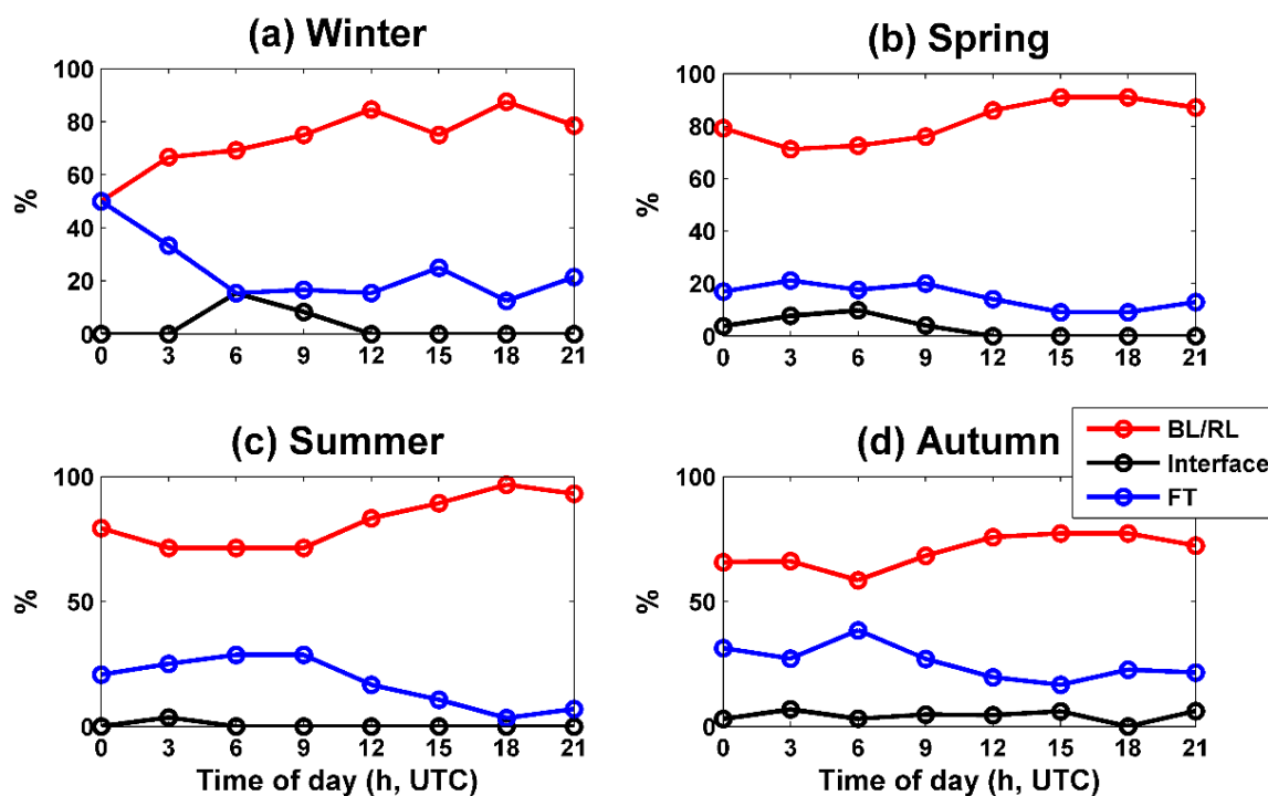
Figure 4.1. 7. The diurnal variation of percentage that the PUY station is in FT/Interface/(BL/RL) conditions for the four seasons: (a) Winter; (b) Spring; (c) Summer; (d) Autumn. red: Boundary Layer (BL) (daytime)/Residual Layer (RL) (nighttime), black: Interface, blue: Free Troposphere (FT).
