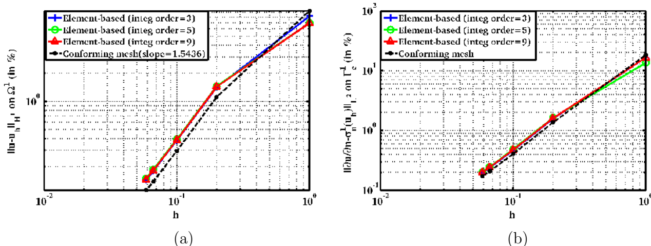
Figure 5.15: Convergence curves with P_2 elements and non-symmetric integration for different integration orders
