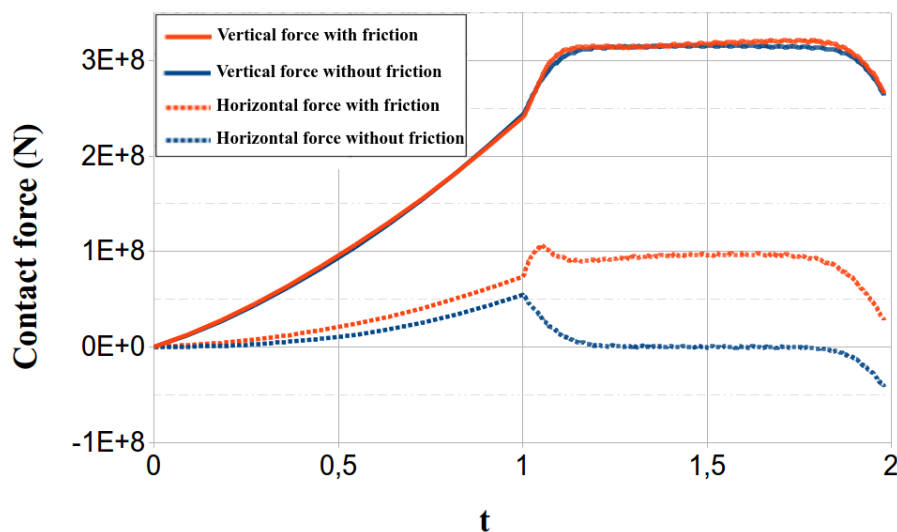
Figure 4.9: Evolution of the vertical and horizontal components of the contact forces for shallow ironing.
