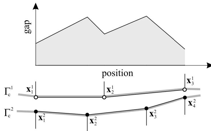
Figure 5.1: Illustration of gap’s variation between two surfaces with non-matching mesh.
