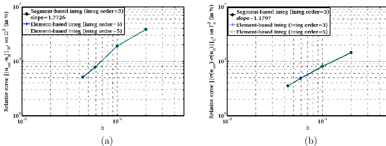
Figure 5.16: Convergence curves with P_1 elements and different integration rules for Hertz problem
