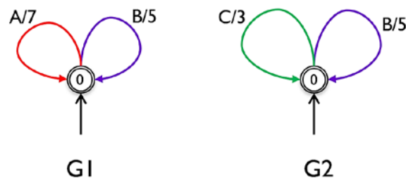
Figure 2.2. Corresponding ME automata for Example 1
