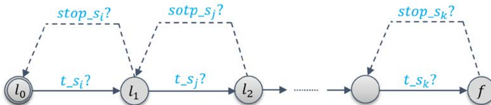
Figure 4.17. Modeling pattern of a triggering PR automata with tasks subject to failure
