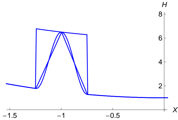
Figure 3.5: Groove shapes: Triangular- Rectangular - Sinusoidal
