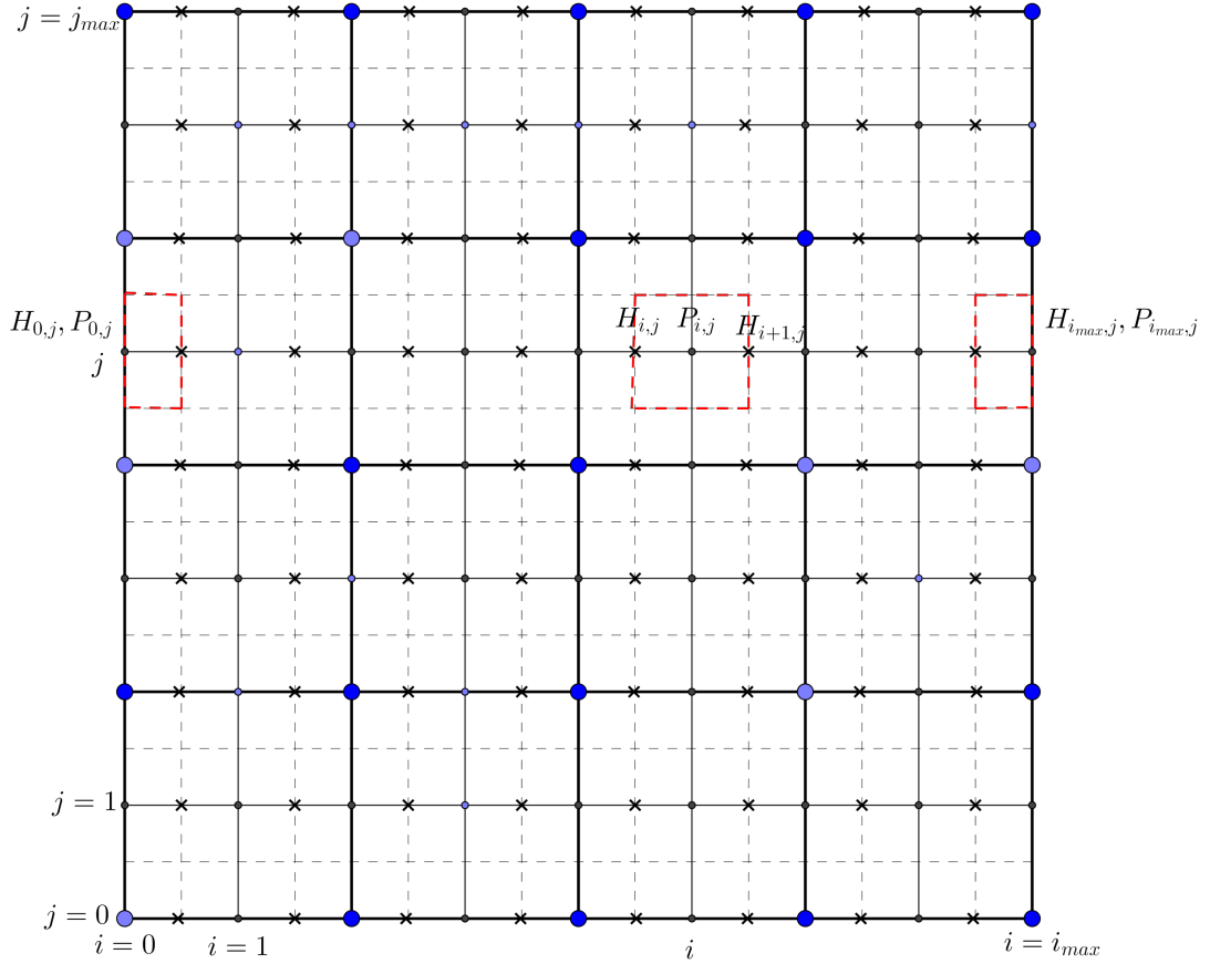
Figure 4.1: 2 grids
