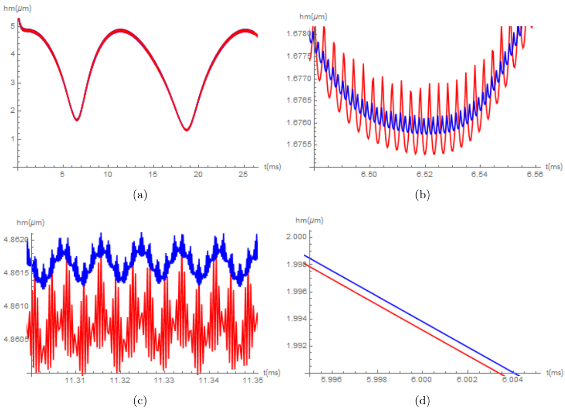
Figure 6.8: In red 7 levels, in blue 8 levels; A = 0.3 , D_1 = 0.25 , \Lambda = 0.2 , h_t = 0.02h_x (a) over an engine cycle (b) zoom around the first minimum (c) zoom around the first maximum (d) velocity close to 0.
