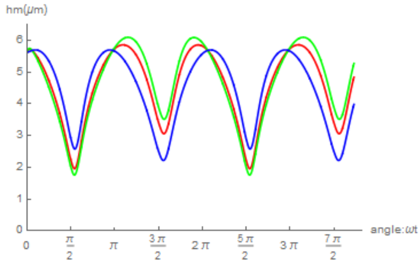
Figure 6.11: Smooth case, in blue constant temperature 125^\circ\text{C} , in red BDC 100^\circ\text{C} and TDC 150^\circ\text{C} , in green BDC 90^\circ\text{C} and TDC 160^\circ\text{C} .
