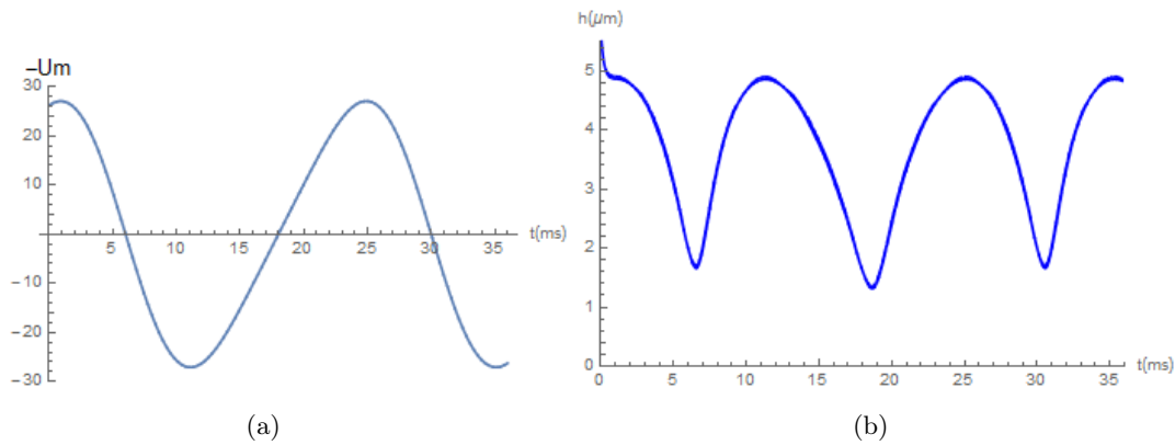
Figure 6.6: On 7 levels, for A = 0.3 , D_1 = 0.25 and \Lambda = 0.2 (a) Mean velocity, (b) Minimum film thickness.
