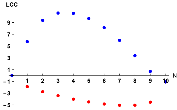
Figure 5.7: Load carrying capacity in terms of the number N of rows of three dimples of depth 1 spaced by D = 4 on \Omega = [-20, 20] \times [-20, 20] . In blue the first row is located at (-18, 0) , in red the last row is located at (18, 0) .
