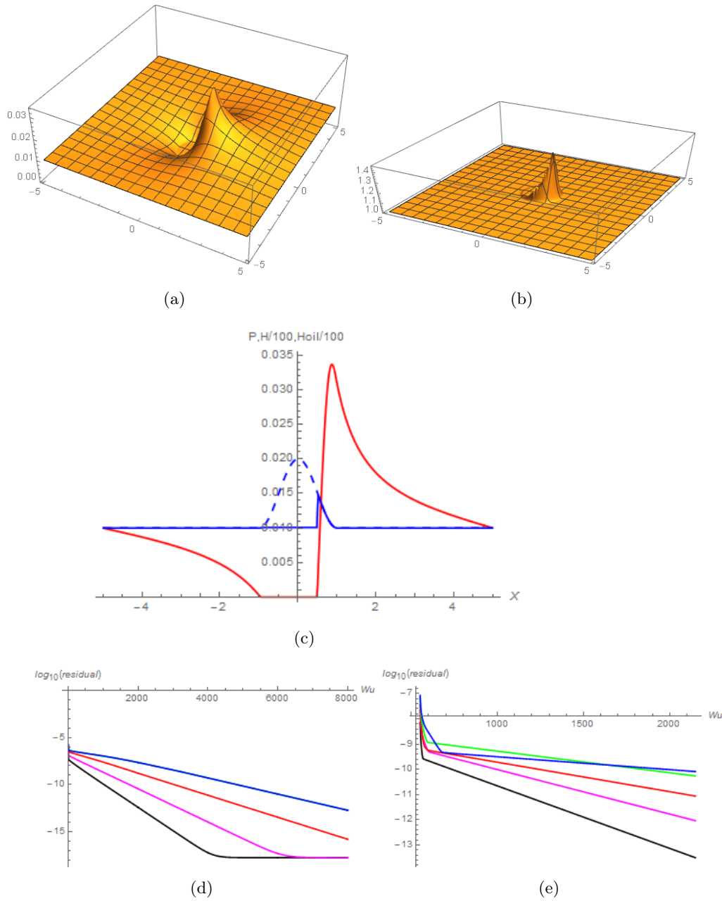
Figure 4.10: Dimple of depth A = 1 - Dirichlet conditions .
