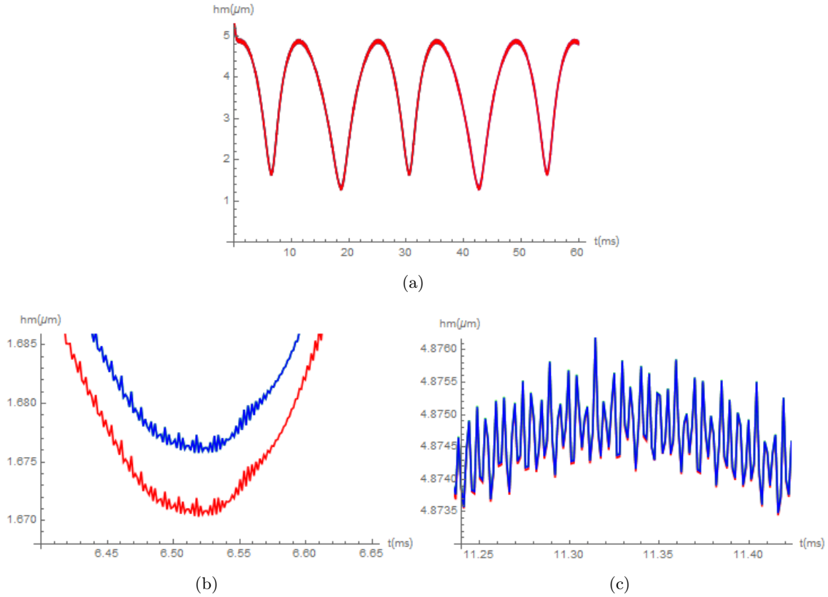
Figure 6.10: 7 levels, A = 0.3 , D_1 = 0.25 , \Lambda = 0.2 , h_t = 0.05h_x , in red ncy=5, in green ncy=20, in blue ncy=10, (a) over two engine cycles (b) zoom around the first minimum (TDC), (c) zoom around the first maximum.
