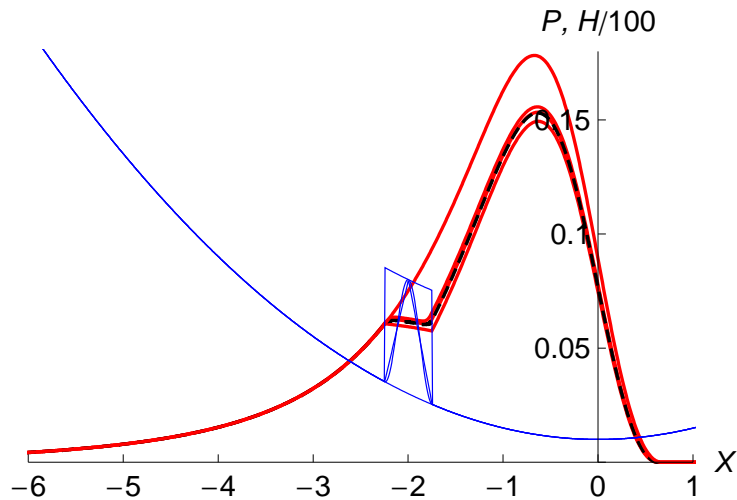
Figure 3.6: Textured pressure distribution and geometry for one groove perpendicular to the sliding direction located at X_g = -2 - A = 5 , E = 10 , \Lambda = 0.5 for various groove shapes: rectangular, triangular, sinusoidal, smooth from bottom to top with the 1D analytical model (dashed line).
