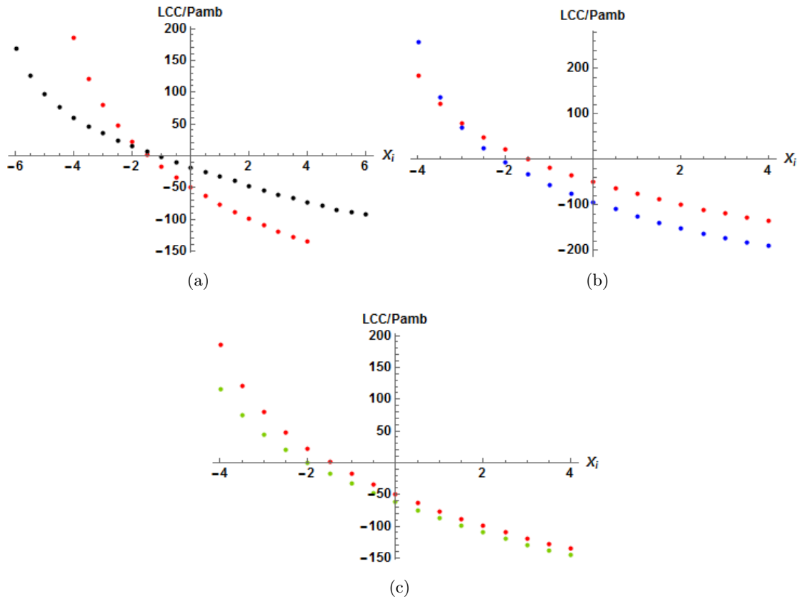
Figure 5.14: Load carrying capacity of a single dimple of identical volume as the nine indent pattern compared with the load carrying capacity (in red) of the pattern of nine dimples of depth 1 spaced by 4 on \Omega = [-10, 10] \times [-10, 10] , (a) a single dimple of radius 3 and depth 1, (b) a square dimple of size 10, (c) a square dimple of size 8.
