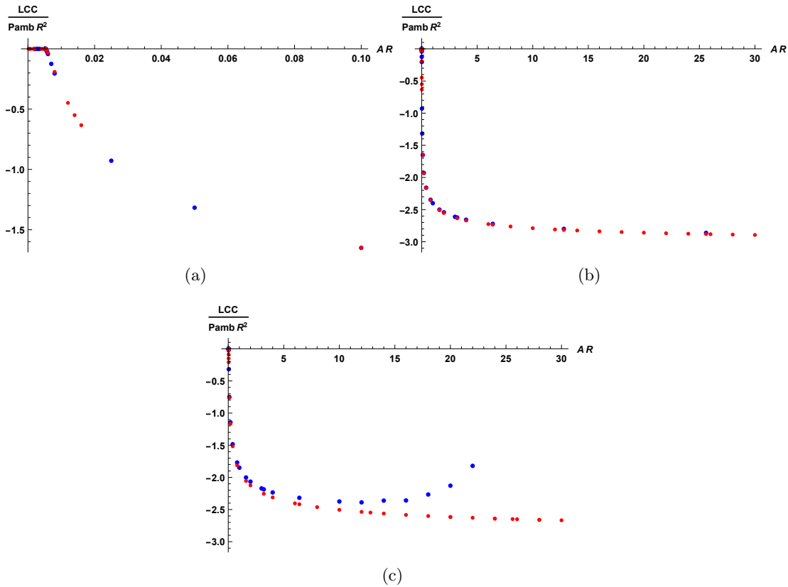
Figure 5.18: Evolution of LCC/(P_{amb}R^2) as a function of AR for two dimple radii: R = 1 in blue, R = 2 in red in the case of a single dimple at the center of \Omega = [-8, 8] \times [-8, 8] . (a) P_{amb} = 0.001 (b) P_{amb} = 0.002 (c) P_{amb} = 0.005 .
