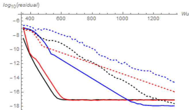
Figure C.16: Residual in terms of work units -No Y -flow- Full lines periodic parabolic geometry: fully flooded in black, H_0 = 1.5 in red and H_0 = 1.1 in blue - Dashed lines periodic wave : fully flooded in black, H_0 = 1.1 in red and H_0 = 1.05 in blue
