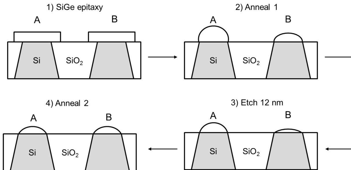
Fig. IV-14: Schematic representation of the experiment. It represents a cross-section perpendicular to the lines ( A = \text{maximum} and B = \text{minimum} of undulations in Fig. IV-13 ). (1) First, a 20 nm thick SiGe epitaxy is done. (2) Second, the layer is annealed at 725°C for 960 sec under 20 Torr of H_2 atmosphere (anneal 1). (3) Third, the lines are thinned by 12 nm (10 nm is left in average). (4) Finally, the layer is again annealed (anneal 2). To note: anneal 1 = anneal 2.
