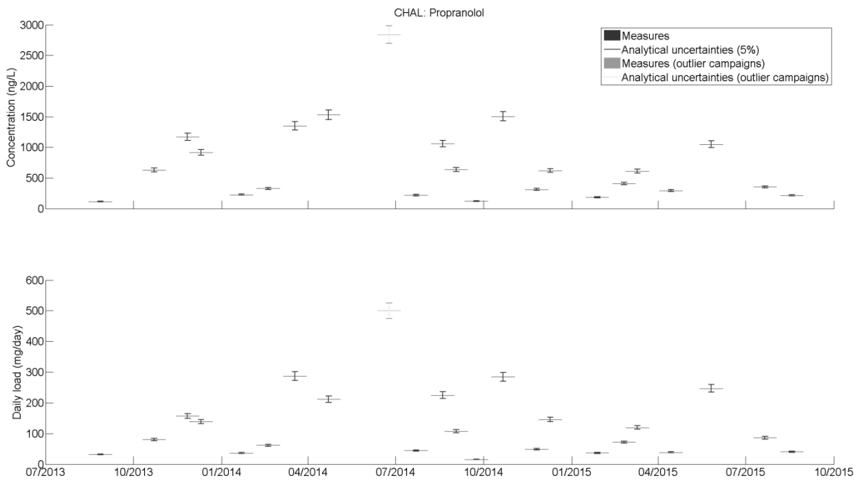
Figure 136: Time series of the daily concentrations and loads of the CHAL hospital for Propranolol.
