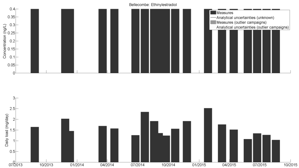
Figure 91: Time series of the daily concentrations and loads of the urban catchment for Ethinylestadiol.
