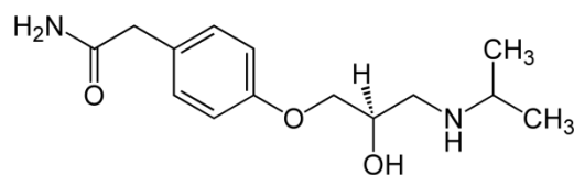
Figure 11: Atenolol molecular structure
