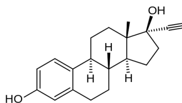
Figure 17: Ethinylestradiol molecular structure
