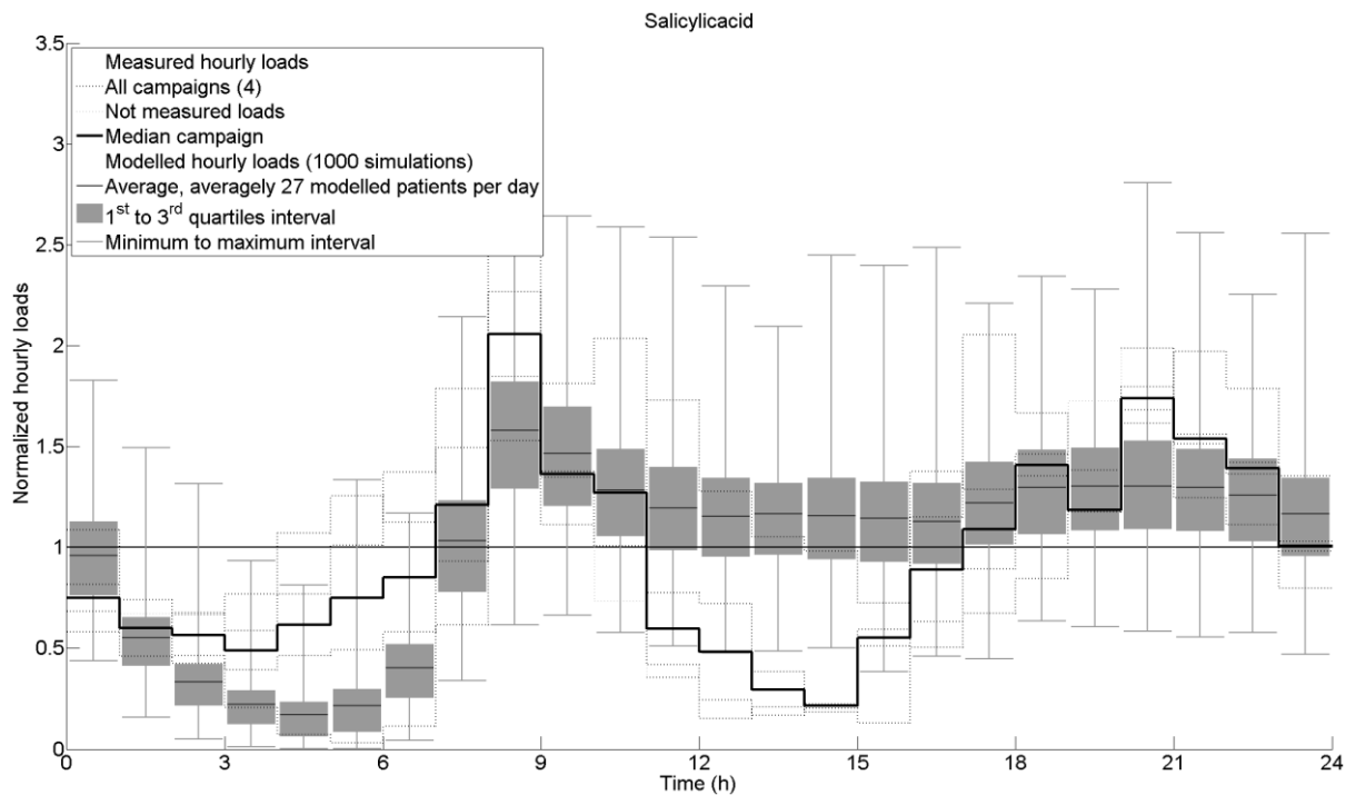
Figure 194: Comparison of the dynamics of the measured and modelled hourly loads of Salicylic acid in the urban catchment.
