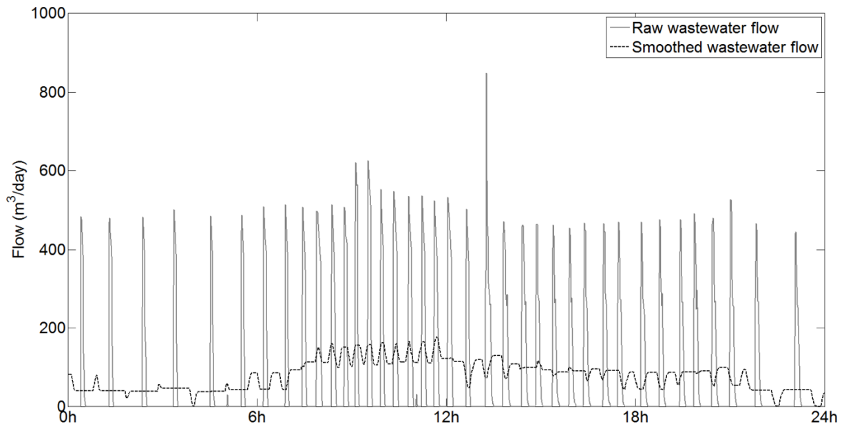
Figure 50: One day of the CHAL raw wastewater flow time series.
