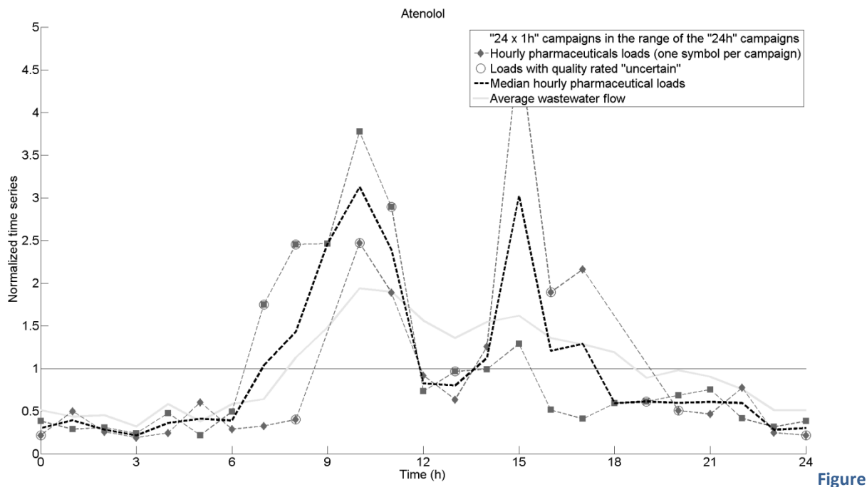
Figure 141: Time series of the hourly loads of the CHAL hospital for Atenolol.
