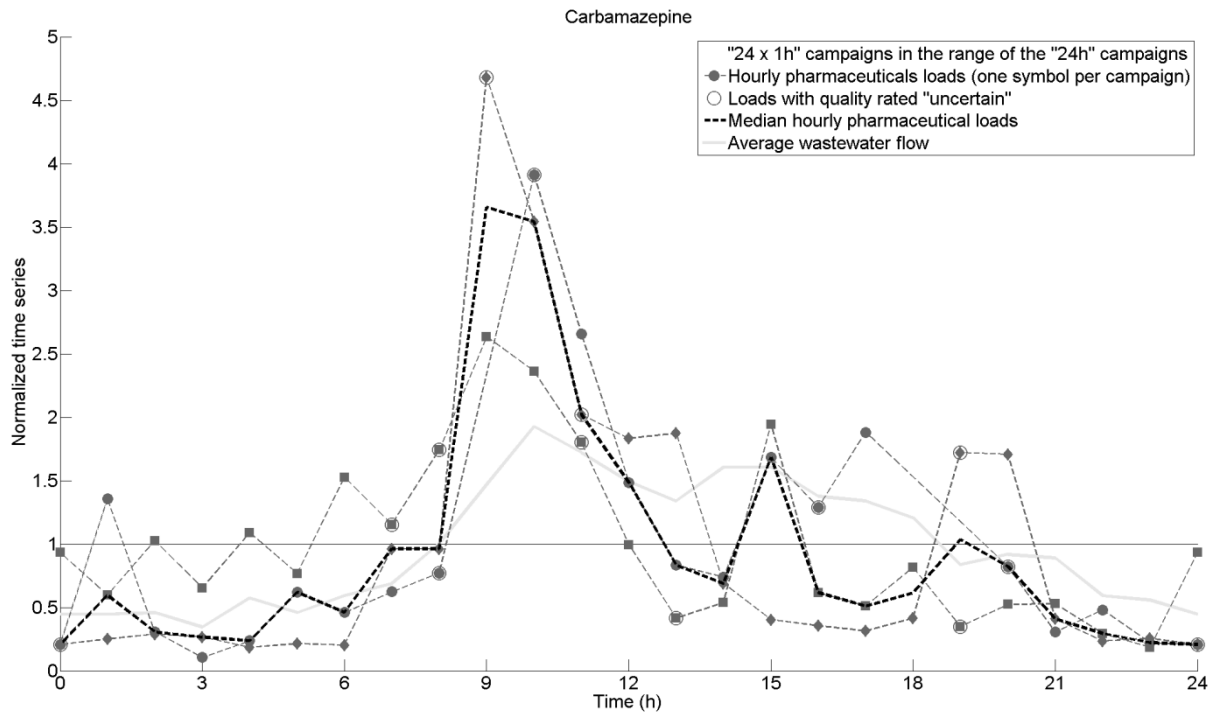
Figure 61: Hourly loads time series of Carbamazepine in the CHAL hospital (average reconstructed daily load equal to 110 mg/day).
