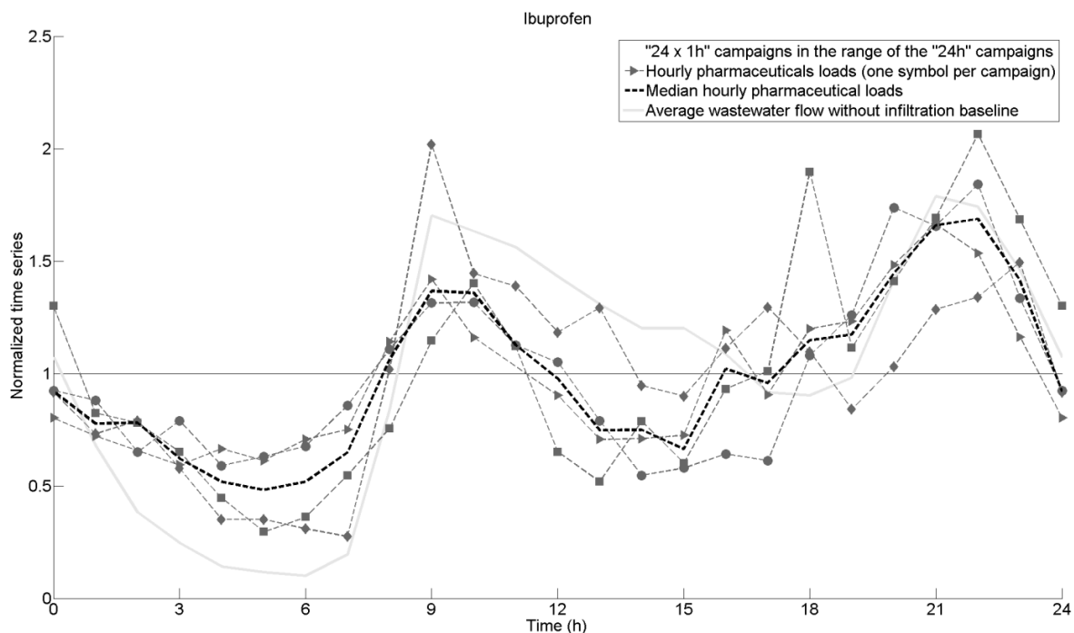
Figure 55: Hourly loads time series of Ibuprofen in the urban catchment.
