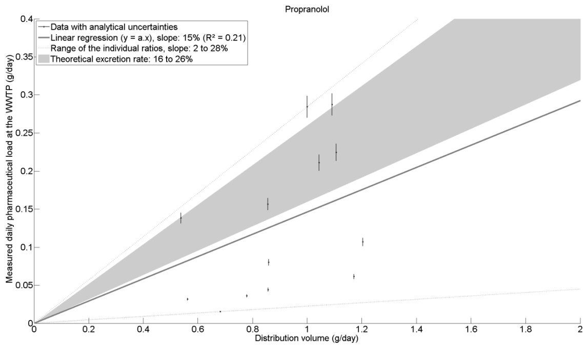
Figure 183: Correlation between distributions and daily loads of Propranolol for the CHAL hospital.
