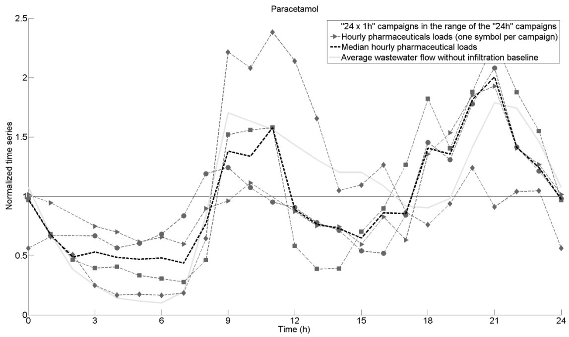
Figure 106: Time series of the hourly loads of the urban catchment for Paracetamol.
