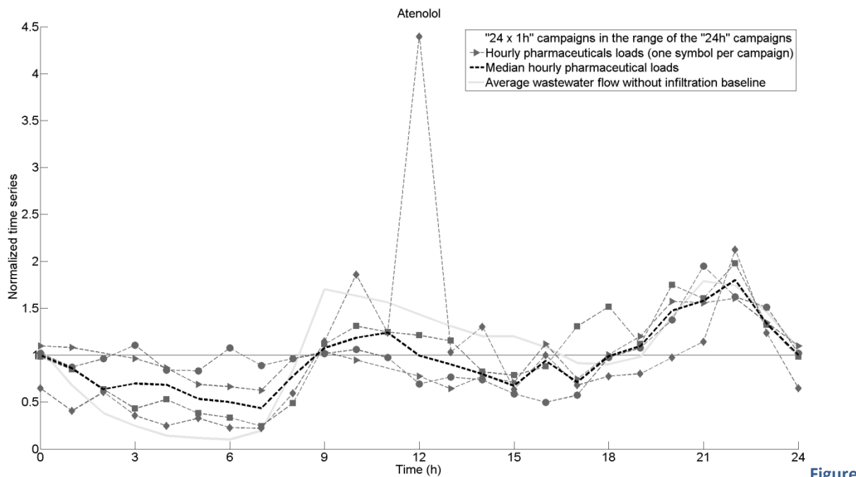
Figure 101: Time series of the hourly loads of the urban catchment for Atenolol.
