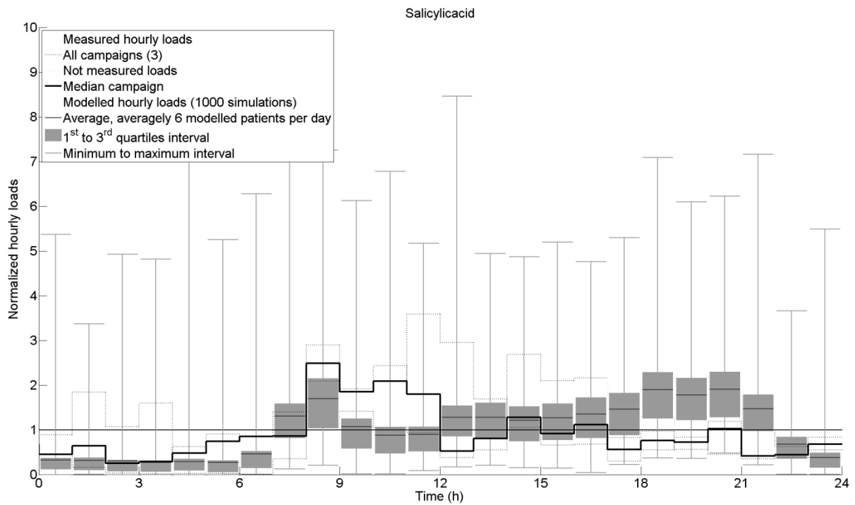
Figure 204: Comparison of the dynamics of the measured and modelled hourly loads of Salicylic acid in the CHAL hospital.
