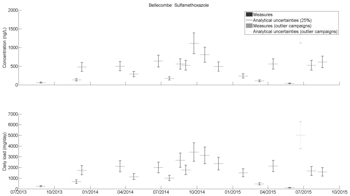
Figure 98: Time series of the daily concentrations and loads of the urban catchment for Sulfamethoxazole.
