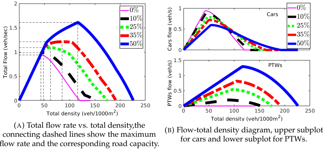
FIGURE 5.1: Flow-density diagram, for different penetration rates of PTWs.
