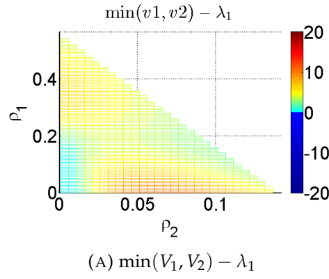
FIGURE 4.2: Evaluation of minimum characteristics speed over a point in S = \{\rho_1, \rho_2\} , Here V_1 = 22m/s and V_2 = 27m/s
