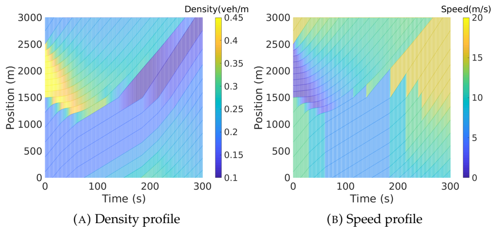
FIGURE 5.17: Evolution of the traffic densities and speed for cars under 2-VSLs
