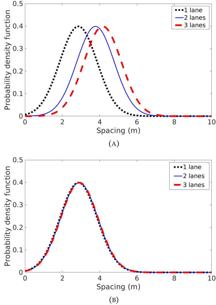
FIGURE B.3: Example of the variation in probability density function with road width (number of lanes)(A) Lower traffic densities ( \rho_1 = 0.01 \text{ veh/m}^2 , \rho_2 = 0.04 \text{ veh/m}^2 ) (B) Higher traffic densities ( \rho_1 = 0.05 \text{ veh/m}^2 , \rho_2 = 0.1 \text{ veh/m}^2 )
