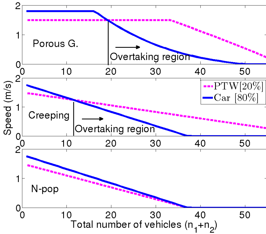
FIGURE 4.13: Speed vs. total number of vehicles plot, when free flow speed of PTWs less than cars and cars account to 80% of the total traffic, upper subplot Porous G , middle subplot Creeping , lower subplot N-pop .
