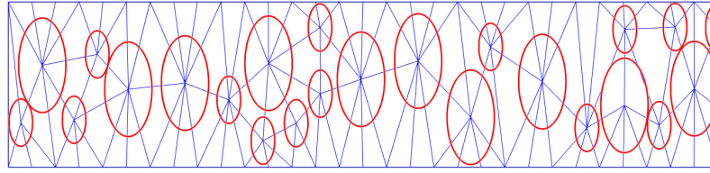
FIGURE 3.3: The implementation of Delaunay triangulation to define pore size
