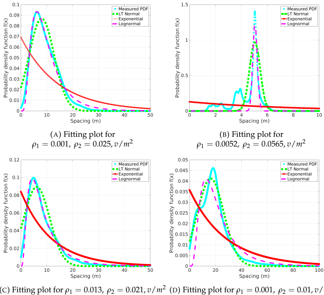
FIGURE 4.19: Fitting of theoretical distributions with the observed distribution, for different vehicles composition
