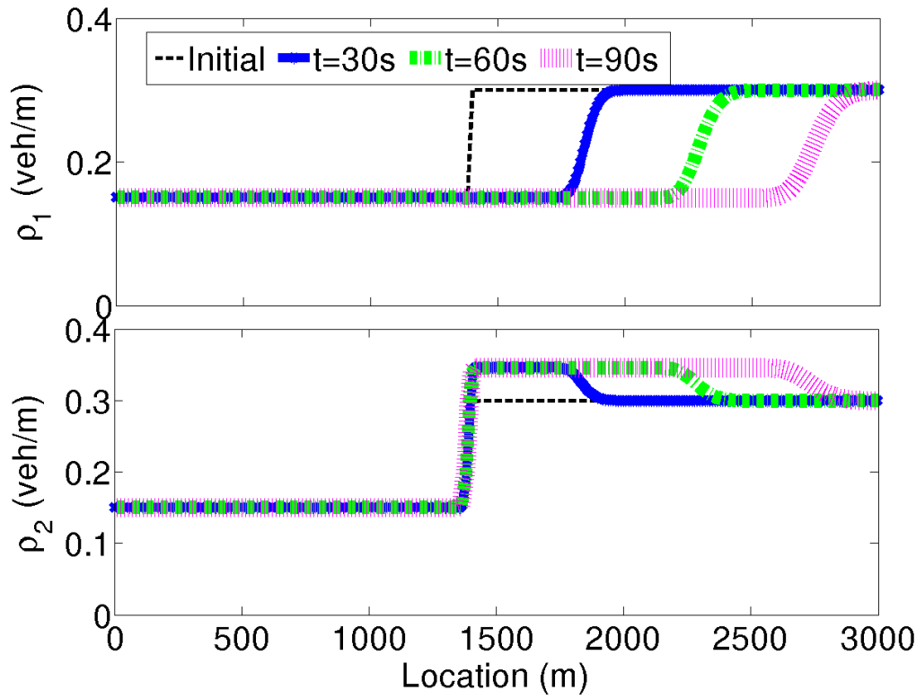
FIGURE 3.19: The density waves of PTWs (upper subplot) and cars (lower subplot), result produced using the general discretization scheme for 1-LRF approach
