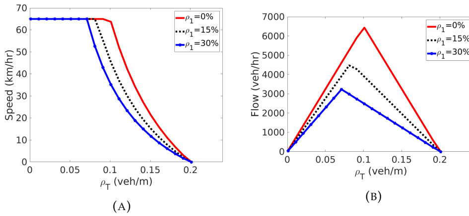
FIGURE 2.8: The variation of (A) speed-density and (B) flow-density relation with traffic composition in (S Logghe and L. H. Immers, 2008; Qian et al., 2017) model
