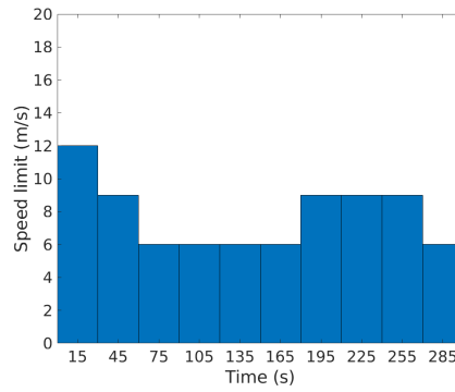
FIGURE 5.16: Time evolution of the speed limit for cars (1-VSL)
