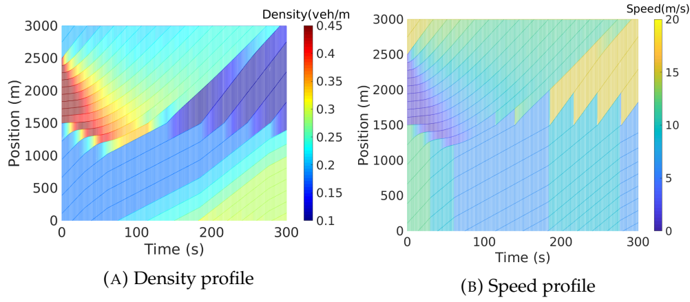
FIGURE 5.15: Evolution of the traffic densities and speed for cars under 1-VSLs
