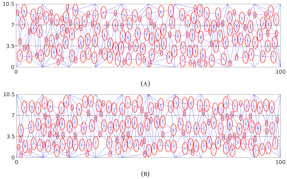
FIGURE B.1: Vehicle distribution in two different settings (A) Disordered flows (B) Semi-ordered flows, \rho_1 = 0.05 \text{ veh/m}^2 , \rho_2 = 0.1 \text{ veh/m}^2
