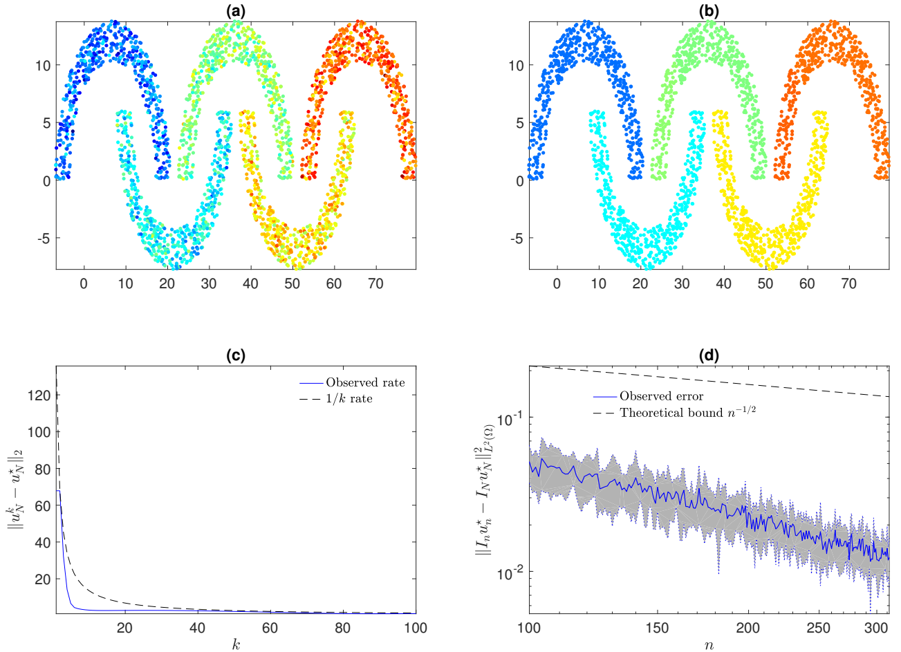
Figure 7.2: Results for point cloud denoising with p = 1 . (a) Noisy point cloud. (b) Recovered point cloud by solving (7.4.1). (c) Primal convergence criterion \|u_n^k - u_n^*\|_2 as a function of the iteration counter k . (d) Mean error \|I_n u_n^* - I_N u_N^*\|_{L^2(\Omega)}^2 across replications as a function of n .
