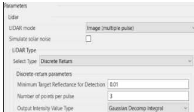
Figure 1-22: Configuration de LiDAR "Multiple pulse" en mode retour discret.
