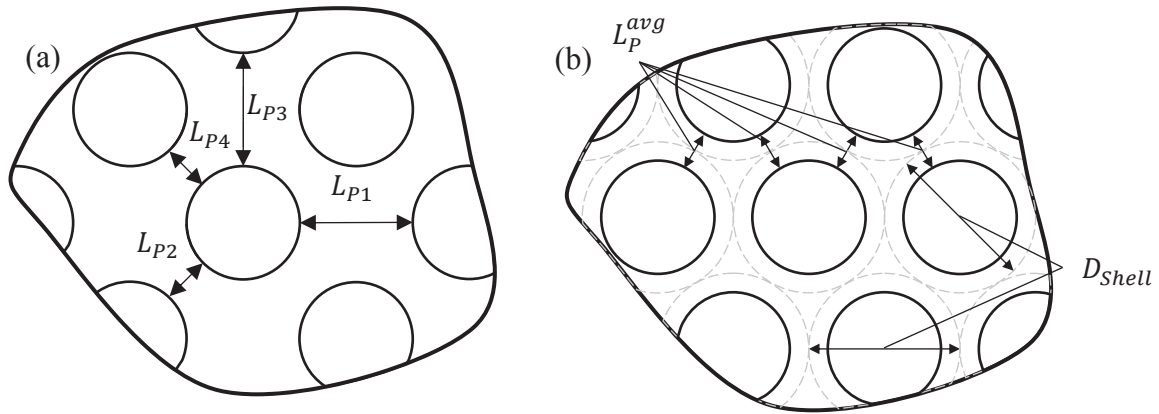
Figure 2.3: Segments of the cross-sectional area of (a) the real hollow fibre module and (b) the modelled hollow fibre module.
