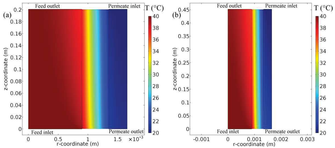
Figure 5.13: Membrane length study. The simulated temperature distributions in the hollow fibre module for the membrane length equal to (a) 0.2 and (b) 0.45 m, respectively ( T_F = 40\text{ }^{\circ}\text{C} , v_F = 0.14\text{ m/s} , T_P = 20\text{ }^{\circ}\text{C} , v_P = 0.5\text{ m/s} ).
