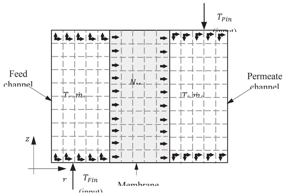
Figure 1.11: Schematic representation of calculated variables in the Hayer's model.
