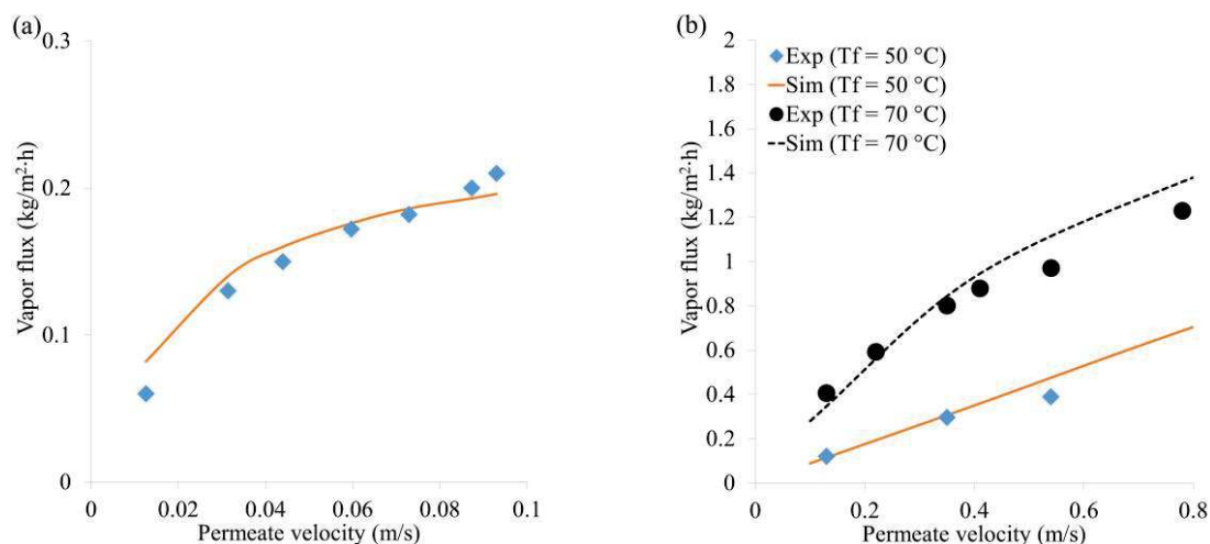
Figure 5.21: Validation of the model and effect of the SG velocity on the water vapour flux at (a) the flat sheet module ( T_F = 25\text{ °C} , T_P = 20\text{ °C} , v_F = 5.6 \times 10^{-3}\text{ m/s} ) and at (b) the hollow fibre module ( T_P = 24\text{ °C} , v_F = 0.02\text{ m/s} ).
