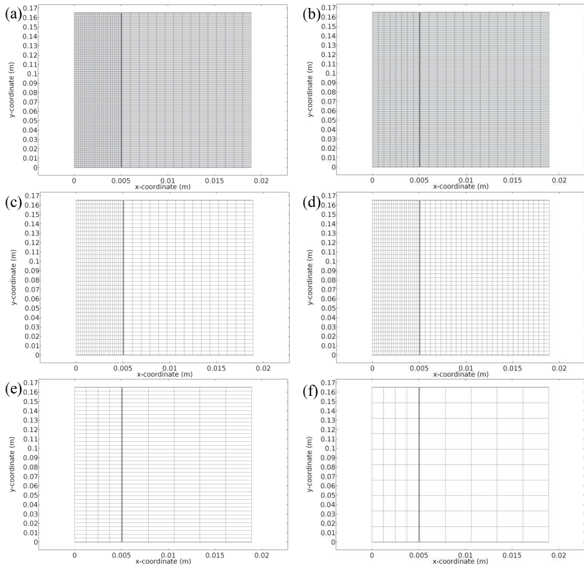
Figure 5.15: Graphical representation of the applied meshes in the mesh study for the flat sheet SGMD module.
