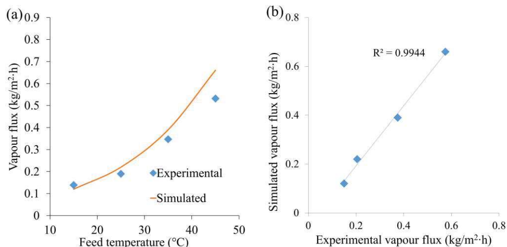
Figure 5.16: Validation of the SGMD model. (a) The effect of the feed temperature on the performance of the flat sheet SGMD module and (b) the corresponding goodness of fit ( v_F=5.6 \times 10^{-3} m/s, v_P=9.3 \times 10^{-2} m/s, T_P=20 °C).
