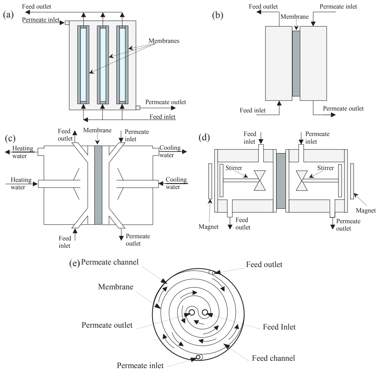
Figure 1.2: Configurations of MD modules: (a) plate and frame module; (b) flat sheet module; (c) thin channel module [52]; (d) Lewis cell [53-56]; (e) spiral-wound module (cross-section) [60].
