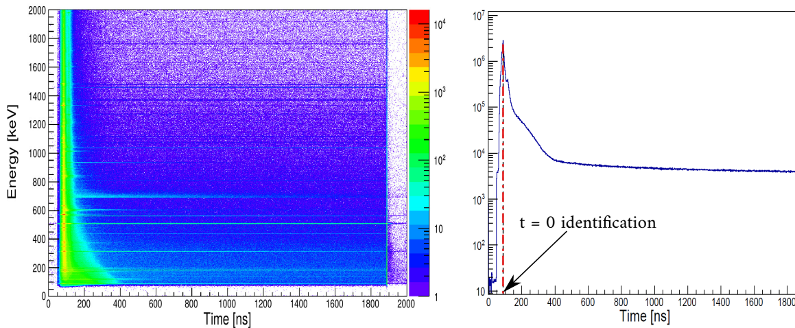
Figure 4.6 – On left two-dimensional histogram of energy vs. time. On right projection of Energy-time matrix on time axis which is used to make t = 0 identification.
