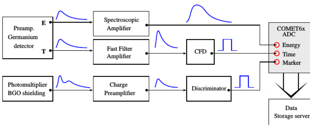
Figure 3.13 – Readout electronics.
