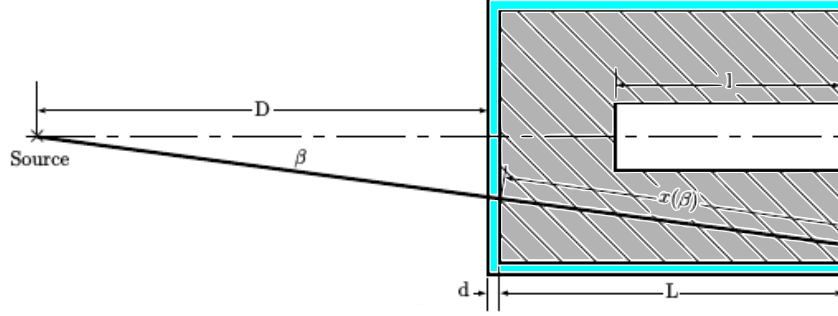
Figure A.1 – Geometry of source-detector configuration for calculation of solid angle correction for coaxial detectors.
