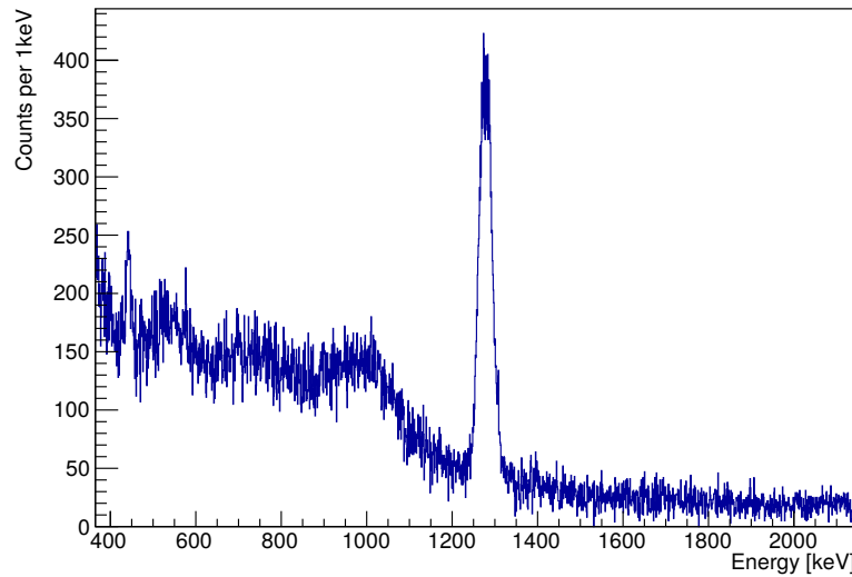
Figure 4.21 – Random-subtracted \gamma -ray spectrum collected at 1 \mu\text{m} plunger separation, showing the ^{22}\text{Ne } 2^+ \rightarrow 0^+ 1274 keV photopeak. Doppler corrected data for all \gamma -ray detectors in coincidence with particle detector is shown.
