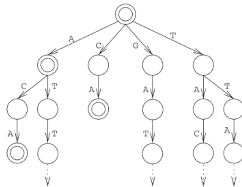
Figure 2.4: The suffix tree of GATTACA.
