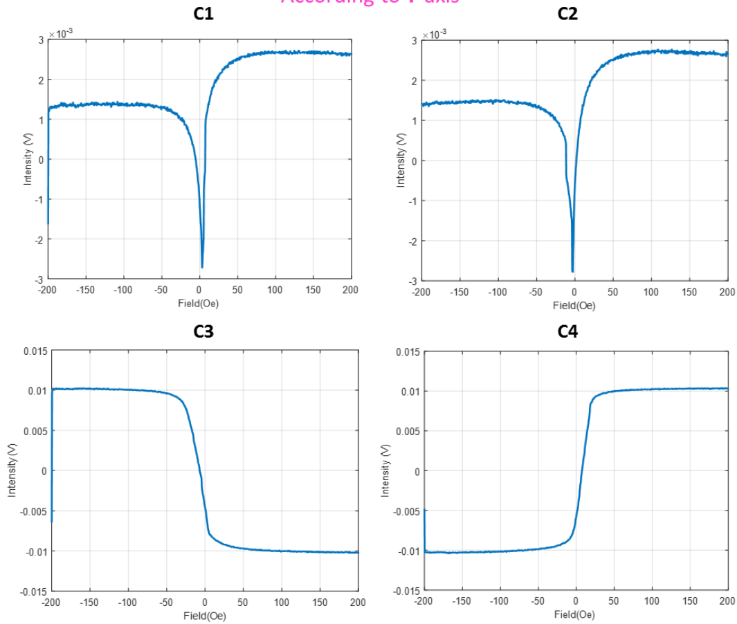
Figure 4.14- The response of four type 1 GMR sensors as function of magnetic field applied along their y-axis.
