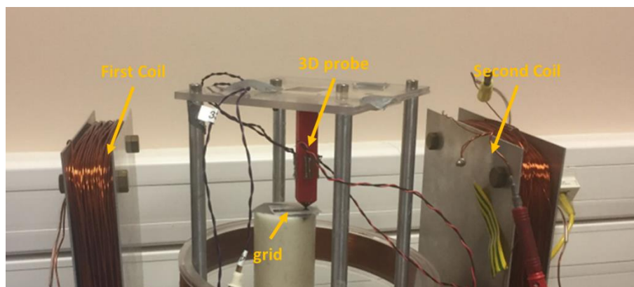
Figure 5.17- Experimental set-up for susceptibility measurement
