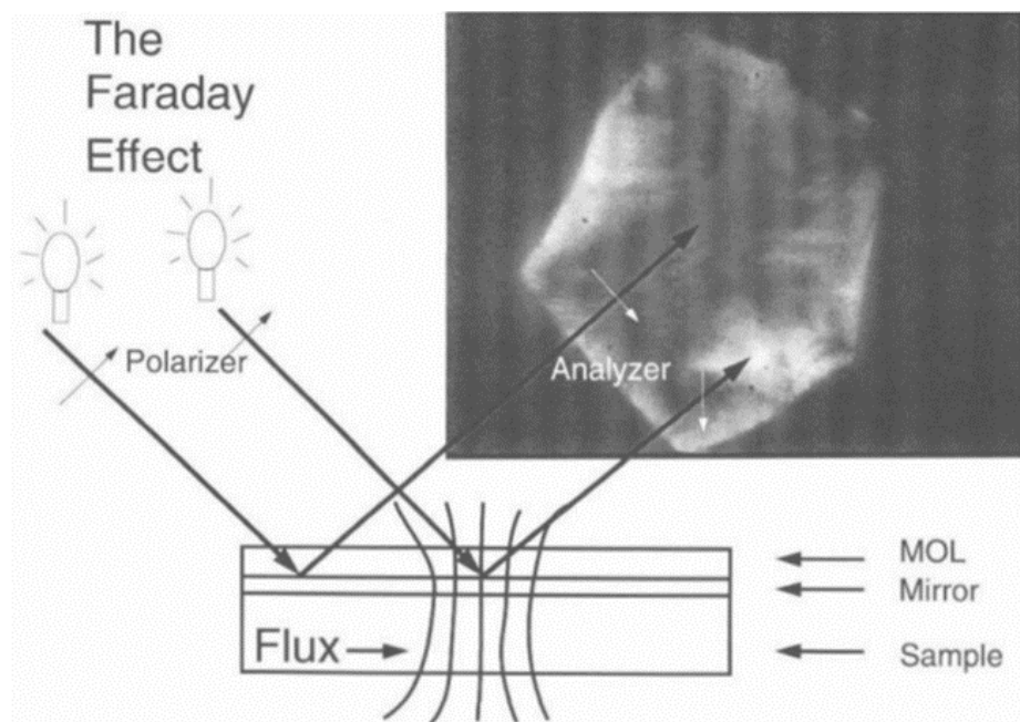
Figure 3.6- Schematic drawing of the Faraday effect. The sample is illuminated by linearly polarized light. Polarizer and analyser are set in crossed position. The light enters the magneto-optically active layer (MOL) and is reflected at the mirror layer. In areas where no flux is present in the sample, no Faraday rotation takes place hence these regions stay dark in the image. In all areas where flux is present, the Faraday rotation changes the polarization plane so that this light is able to pass through the analyser thus leading to bright areas. In the drawing, a reflection angle \theta is shown for clarity whereas in the experiment we have perpendicular incident light. [154]
