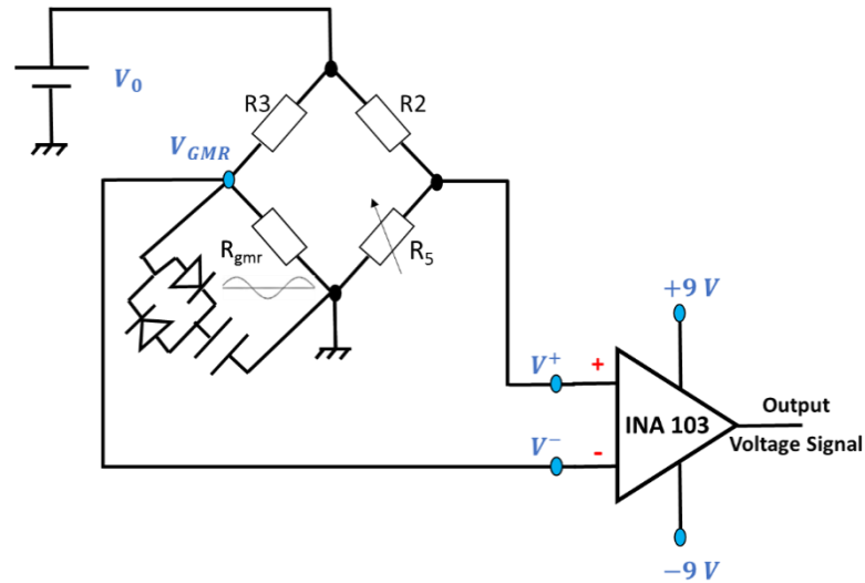
Figure 4.3- Full bridge circuit relied to INA103
