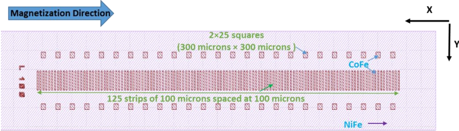
Figure 5.13- The grid composed of magnet strips.
