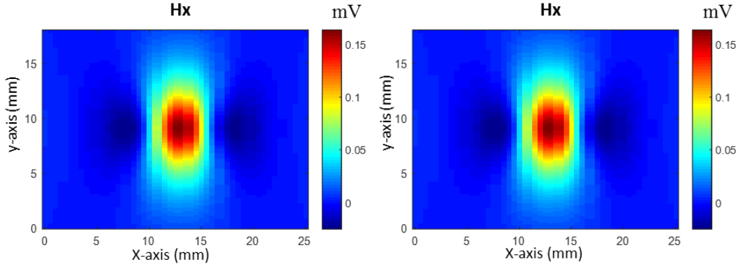
Figure 6.7- CSCAN of the defect in aluminum mock-up obtained with receiver places according to x-axis (left part), reconstruction of H_x component obtained with 3D EC probe (right part).
