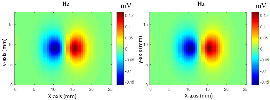
Figure 6.9- CSCAN of the defect in aluminum mock-up obtained with receiver places according to z-axis (left part), reconstruction of H_z component of magnetic field with 3D EC probe (right part)
