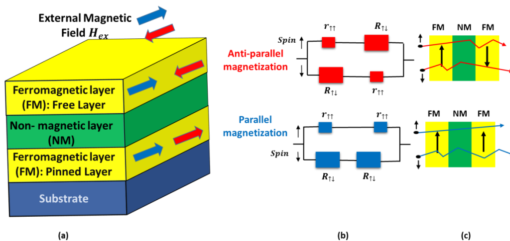
Figure 1.16- GMR structure: (a) Free layer, spacer and pinned layer Illustration of the spin-dependent scattering in ferromagnetic materials (FM). The spacer is non-magnetic (NM); (b) The equivalent electrical circuit with two conducting channels is shown for anti-parallel magnetizations (red) and for parallel magnetizations (blue); (c) The figures at the top illustrate the trajectory of the electrons in antiparallel configuration and illustrate at the bottom the parallel configuration .
