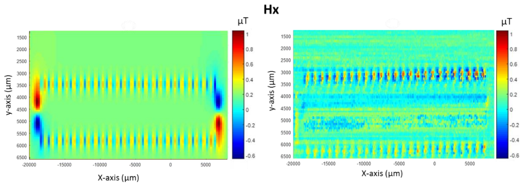
Figure 5.14- Simulation results ( left part ) and experimental results ( right part ) in the case of H_x component analysis
