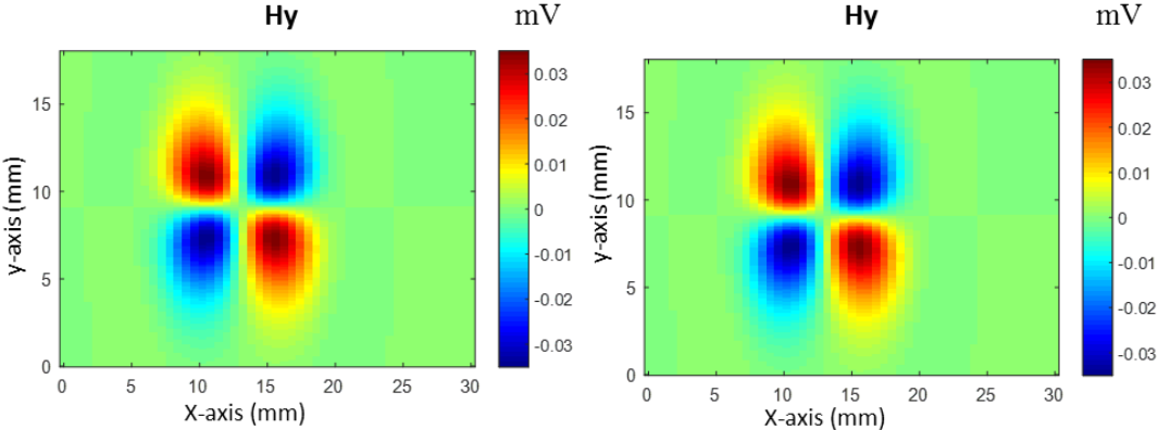
Figure 6.8- CSCAN of the defect in aluminum mock-up obtained with receiver places according to y- axis (left part), reconstruction of H_y component of magnetic field with 3D EC probe (right part).
