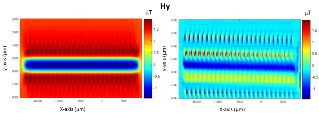
Figure 5.15- Simulation results ( left part ) and experimental results ( right part ) in the case of H_y component analysis. The maximum amplitude is equal to 1.6 \mu T
