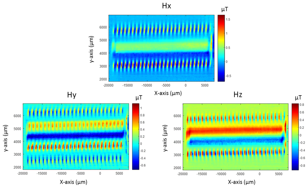
Figure 5.18- The three components of magnetic field in the case of susceptibility measurement. The maximum amplitude values are equal to H_x = 1.5 \mu T , H_y = 1 \mu T , H_z = 0.8 \mu T .
