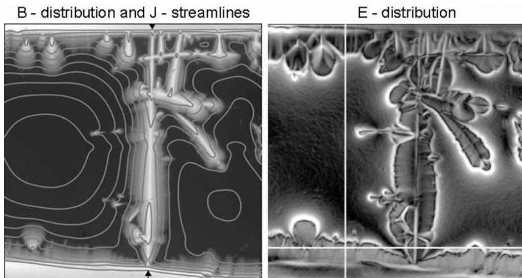
Figure 3.7- Magneto-optical images used to calculate distribution of electric field at 4.2 K in the superconductor. The image shows such distributions for a YBCO film with a grain boundary [161]
