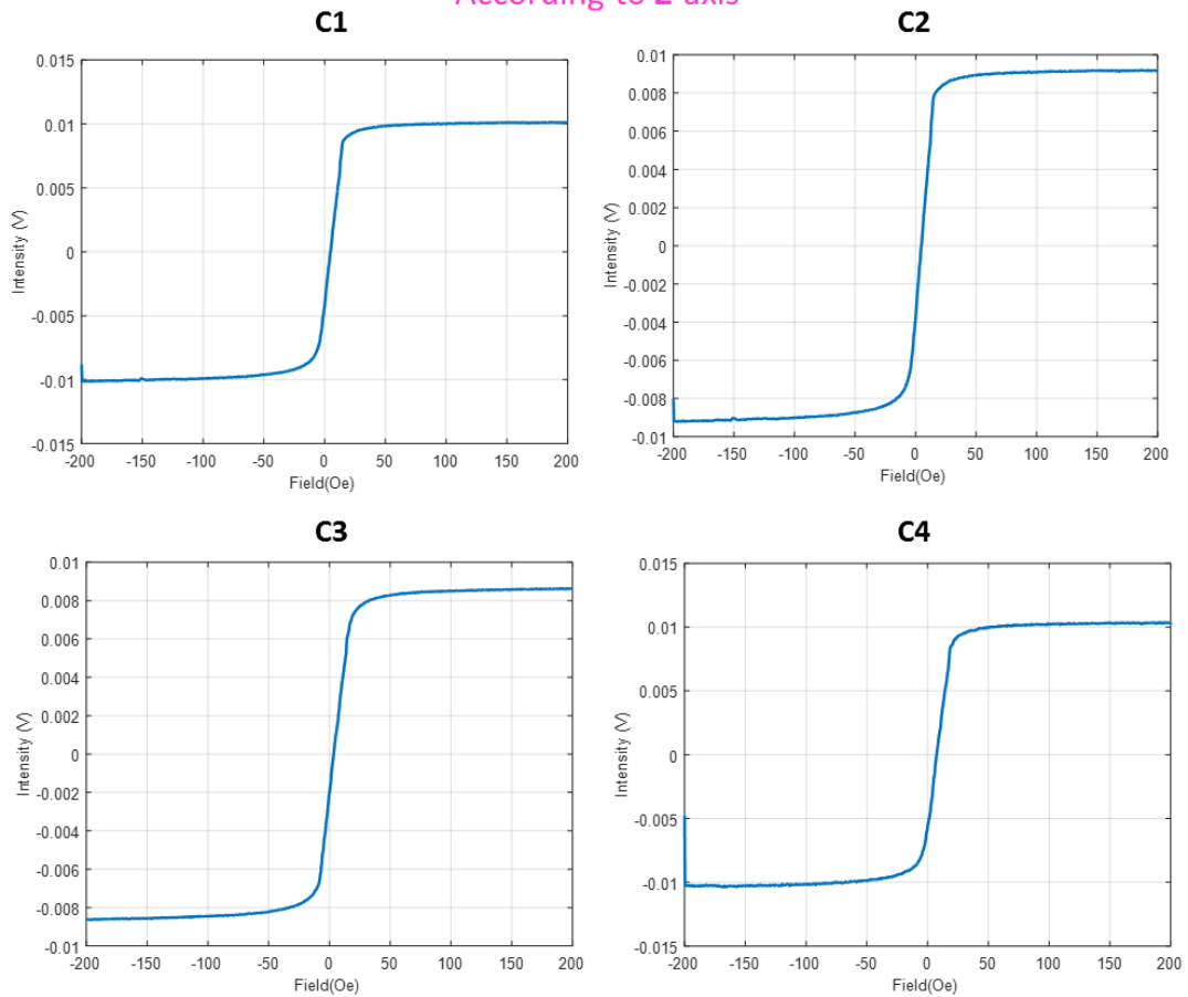
Figure 4.13 – The response of four type I GMR sensors as function of magnetic field applied along their z-axis
