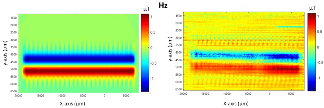
Figure 5.16- Simulation results (left part) and experimental results (right part) in the case of H_z component analysis. The maximum amplitude is equal to 1.2 \mu T
