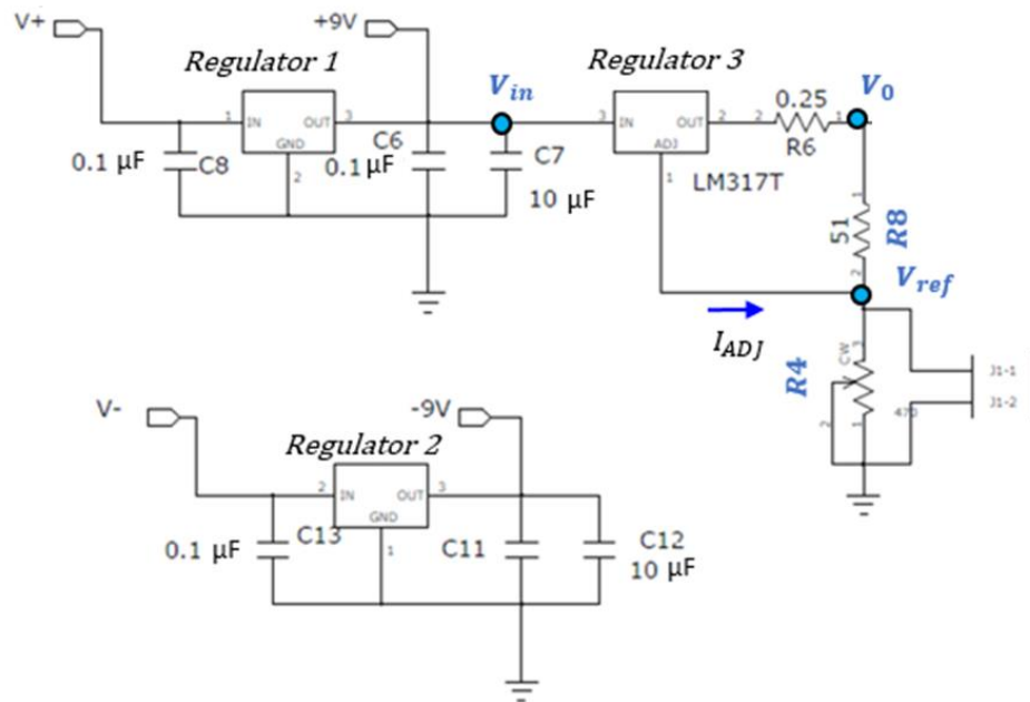
Figure 4.2 Alimentation part of electronic circuit
