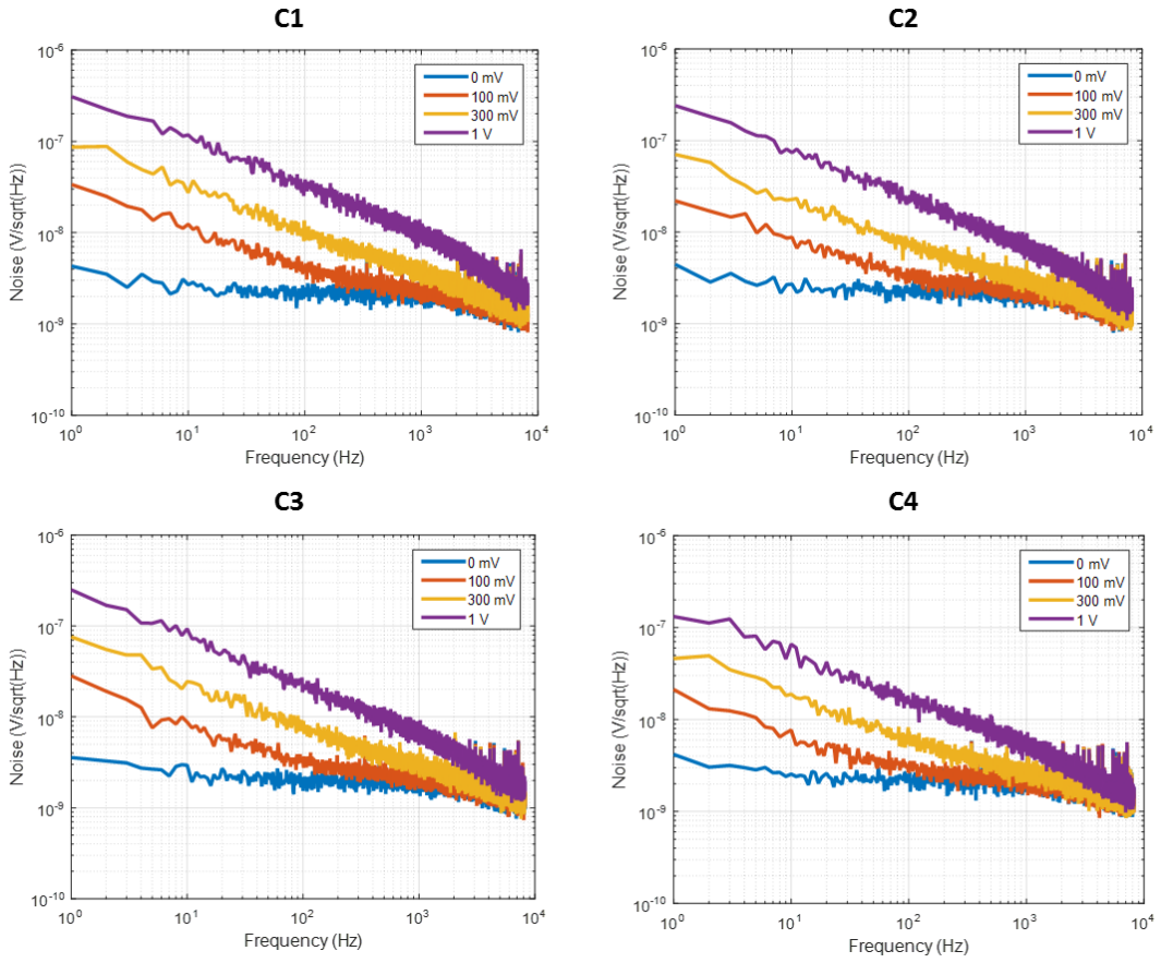
Figure 4.24- Noise spectral density in V/\sqrt{\text{Hz}} of four type 2 sensors with V_{\text{GMR}} = 0 \text{ mV}, 100 \text{ mV}, 300 \text{ mV} and 1 \text{ V}
