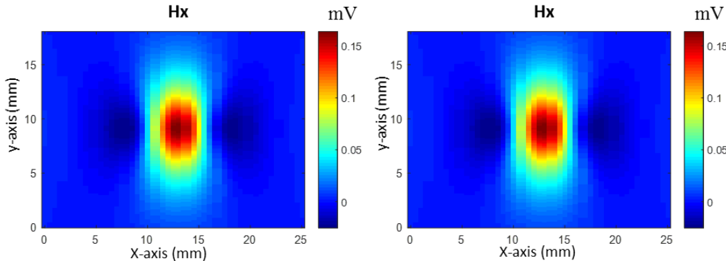
Figure 6.7- CSCAN of the defect in aluminum mock-up obtained with receiver places according to x-axis (left part), reconstruction of H_x component obtained with 3D EC probe (right part).
