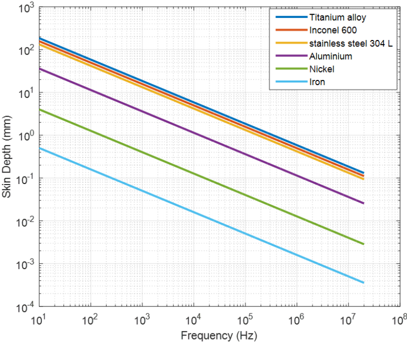
Figure 2.8- Evolution of skin depth against frequency for different materials
