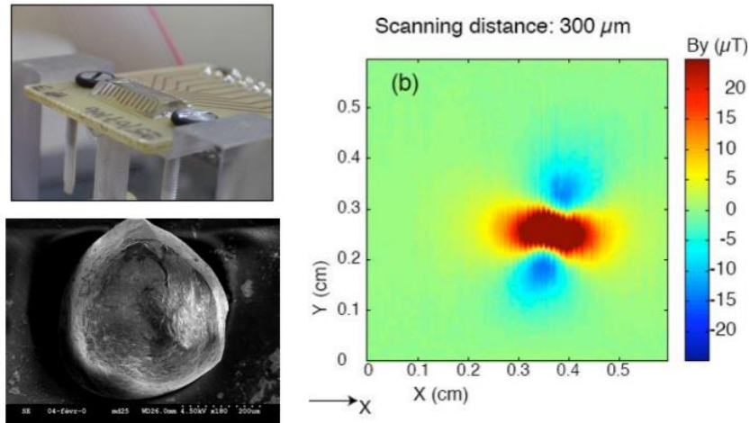
Figure 1.14- Left: GMR scanning element for magnetic field mapping. SEM picture of a 450µm meteorite collected in Antarctica, Right: Magnetic mapping of the meteorite magnetic dipole. Coll. Cerege – Jérôme Gattacceca [66].
