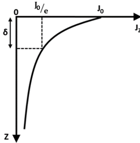
Figure 2.7- Evolution of current density as function of piece depth ( z ) in the case of plane wave excitation [104].
