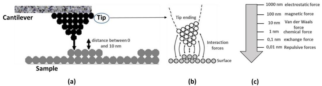
Figure 3.3- Atomic force microscopy principle (a) Tip form (b) Long- and short-range (interatomic) forces dependent of various distance (c) [131, 133]
