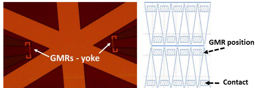
Figure 4.10- GMR sensor in a yoke-shape before cutting
