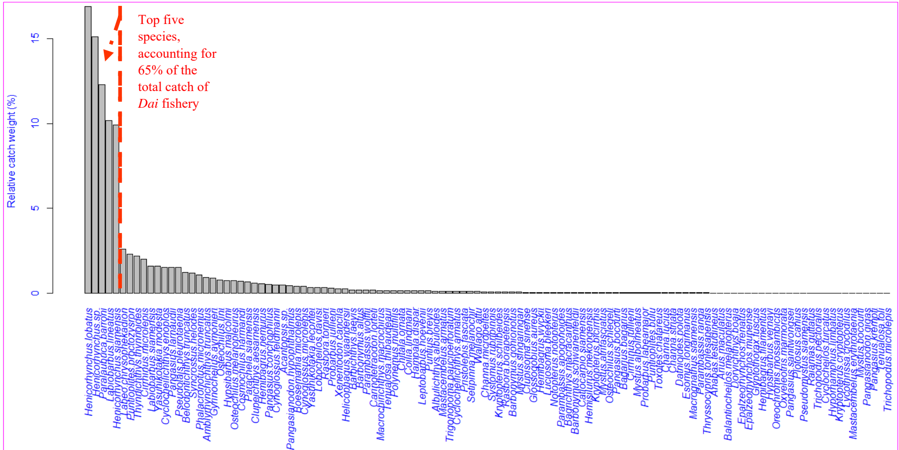
Fig. S4 Relative catch weight (%) of 116 fish species recorded at the Dai fishery between 2001 and 2015
