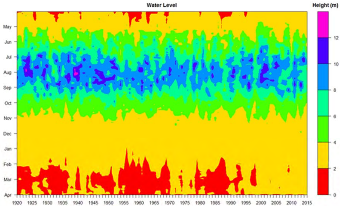
Fig. 6. Temporal raster plot of daily water levels (m) of the Mekong River, Stung Streng Province, 1920-2015.
