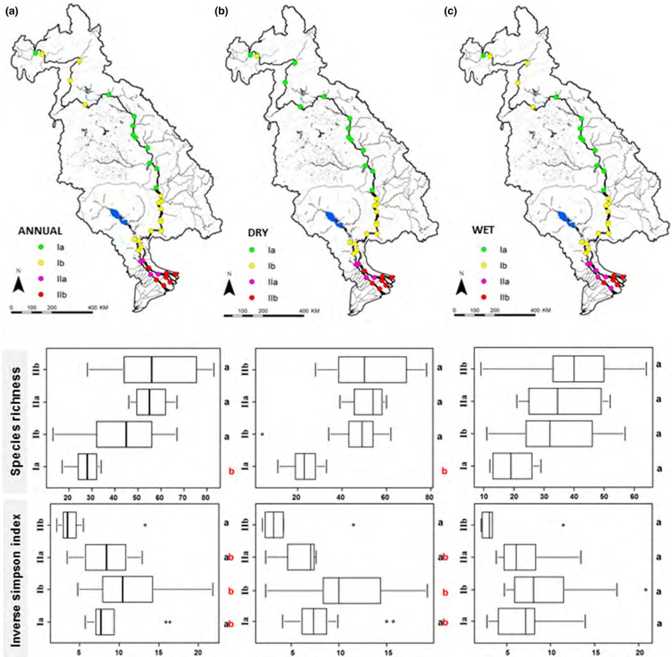
FIGURE 2 Fish distribution and assemblage patterns in Lower Mekong River. Annual (a), dry season (b) and wet season (c) clustering associated with species richness and Inverse Simpson index of each cluster (Ia, Ib, IIa, IIb). For each box plot, the dark line inside the box represents the median value, while the lines below and above indicate the 25 and 75 percentiles respectively. The whisker marks represent the minimum and maximum values. Mean values among clusters with a common letter are not significantly different at p = .05 (Tukey's HSD tests)
