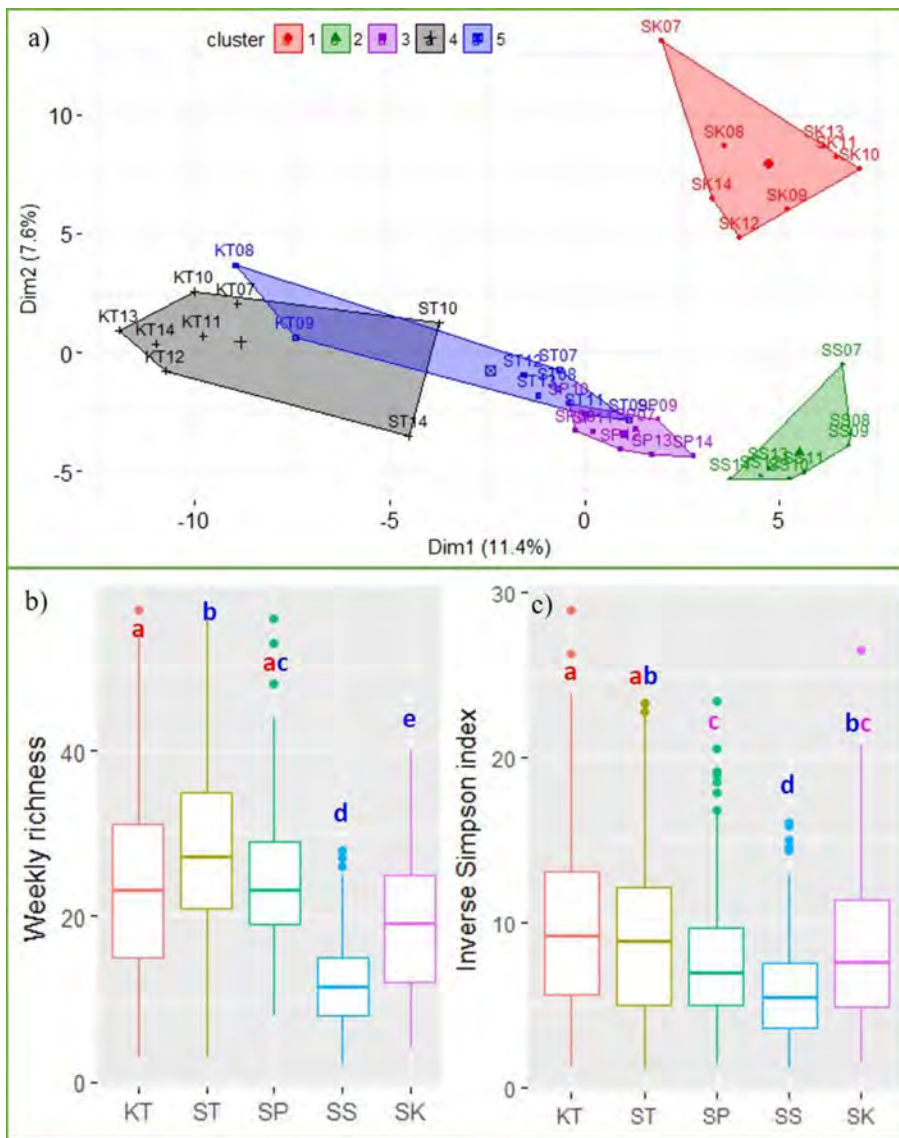
Fig. 3. Fish assemblage patterns in the Mekong-3S system. (a) K-means cluster on PCA plot (k = 5) on Hellinger-transformed yearly assemblage data. Five convex hulls (with different colours) represent each assemblage cluster of the Mekong-3S system. A combination of two letters and two digits denotes the site name and year; for example, KT07 is Kratie in 2007. (b) Boxplots of total weekly richness by site; (c) Boxplots of weekly inverse Simpson diversity index by site. Mean values among sites (Fig. 5b, c) with a common letter are not significantly different at the 0.05 level (Pairwise Wilcoxon Rank Sum Tests). For site names, see Fig. 1.
