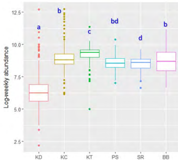
Fig. 15. Spatiotemporal comparison of site fish species abundance in the Tonle Sap River and Lake. Mean values among sites with a common letter are not significantly different at p -value=0.05 (Wilcoxon test). For site names, see Fig. 14.
