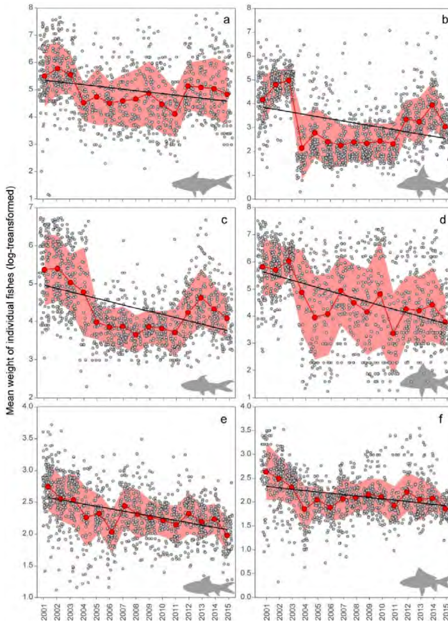
Fig. 4. Linear regressions demonstrate temporal change in log-transformed mean individual weight (g) by season of six common species, composing of large (a: Pangasianodon hypophthalmus ; b: Cyclocheilichthys enoplos ), medium (c: Cirrhinus microlepis ; d: Osteochilus melanopleurus ) and small-sized species (e: Henicorhynchus lobatus ; f: Labiobarbus lineatus ) that possessed either negative (a-d) or positive (e, f) catch changes (expressed as standardized regression coefficients, Table S6) from the fishing season of 2000/01 to 2014/15. See Table S7 for parameter estimates. All slopes were significant ( p -value <0.0001 ). Solid red dots indicate mean body weight and the pink shaded area denotes standard deviation for each survey season across the study period. 2001 represents the fishing season of 2000/2001 and the same for other years.
