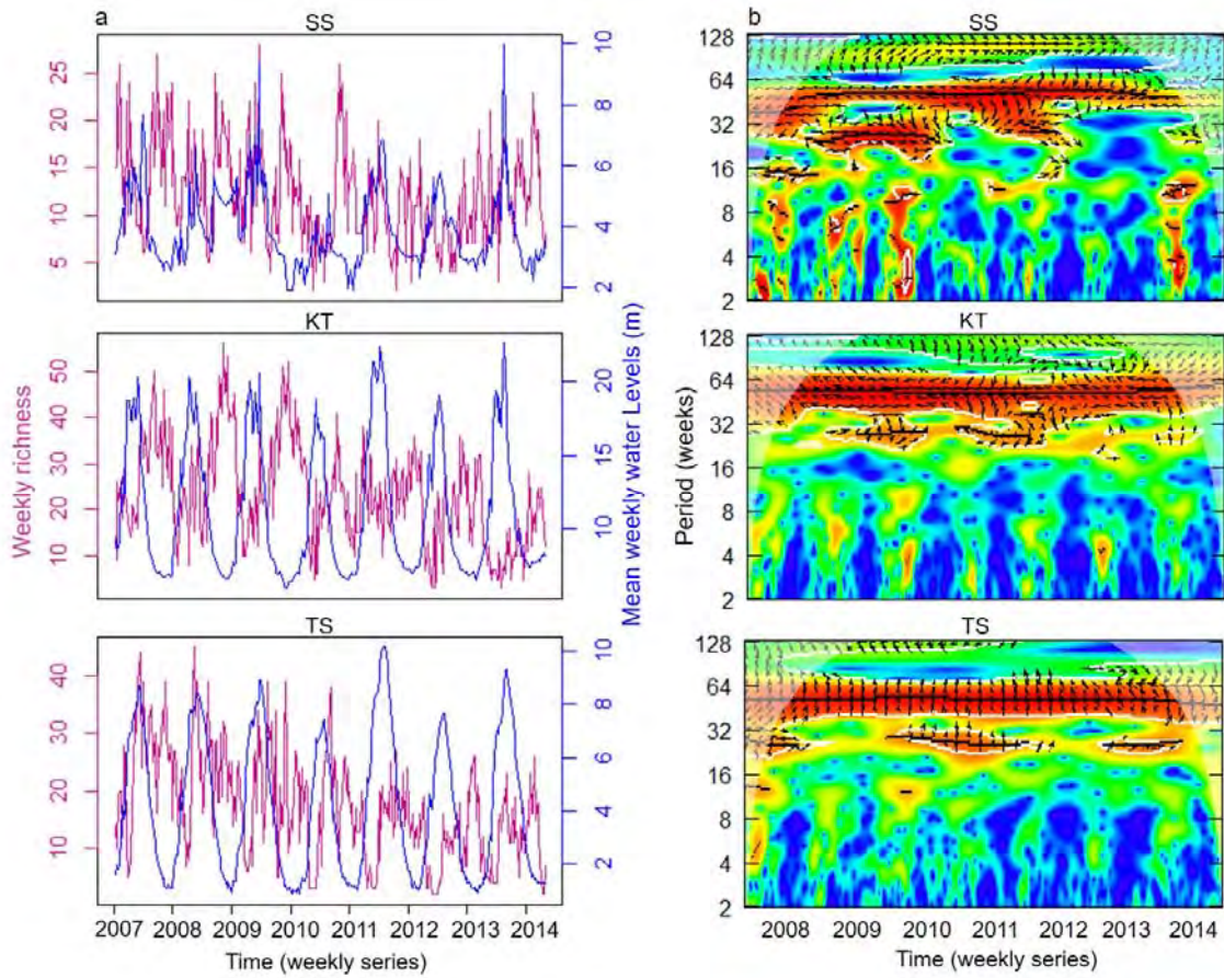
Fig. 33. Temporal variation of total weekly richness (y) and mean weekly water levels (x as predictor). (a) Weekly richness and mean water level data series, covering the period from 1 June 2007 to 31 May 2014. (b) Cross-wavelet power spectrum of weekly richness and water levels. Red color represents stronger cross-wavelet power, and blue weak. Arrows in each plot depict phase-differences. Ridge lines illustrate cross-wavelet power coherence within a band of neighboring periods. Areas in the upper corners, outside the ‘cone of influence’ in each plot indicated the exclusion of areas from edge effects (with weak predictive ability). For site names, see Fig. 32.
