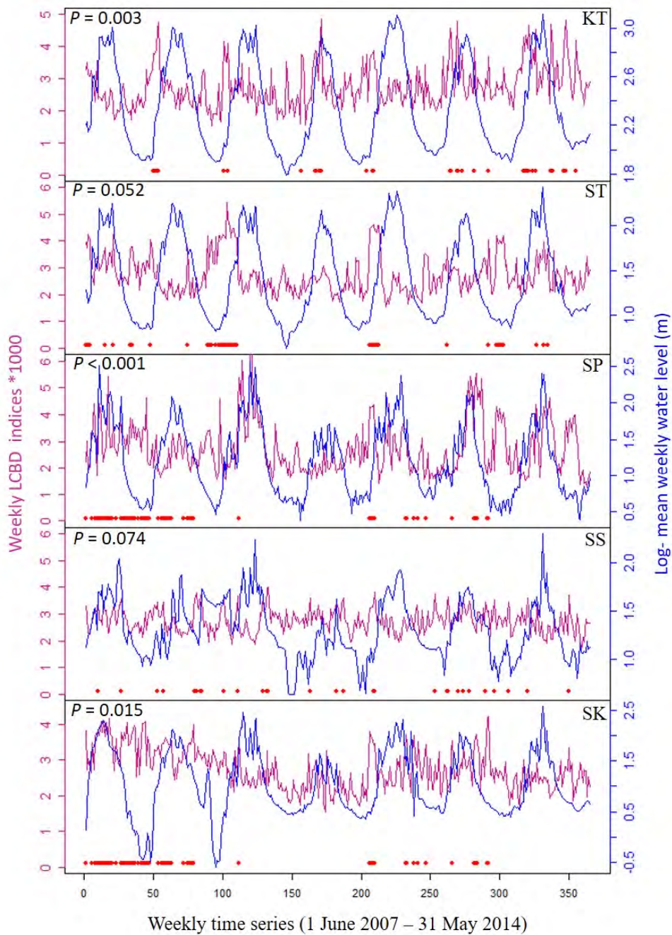
Fig. 31. Temporal changes in LCBD indices (red line) and mean log-transformed weekly water levels (blue line) over 7-year hydrological cycles on the five sites of the Mekong-3S River system. More predictable-seasonal flow patterns are shown in KT and ST, and unpredictable/regulated flows are displayed in SP, SK, and SS. The red dots indicate weeks with significant LCBD indices at the 0.05 level. P denotes the p-value of the pairwise correlation test using the Spearman method. For site names, see Fig. 30.
