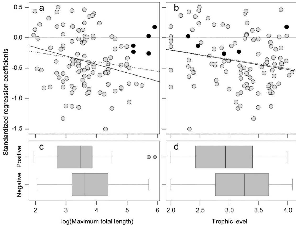
Fig. 23. Relationship between (log+1 transformed) standardized regression coefficients of species composition derived from seasonal catches of 116 fish species recorded at the Dai fishery in the Tonle Sap River from the fishing season of 2000/01 to 2014/15, and (a) their corresponding log-transformed maximum total lengths (maxTL in cm) and (b) trophic levels. Solid points represent endangered (en) and critically endangered (ce) species. Dashed lines show linear regression lines to predict the relationships when all species are considered, and solid lines are linear regression lines when en and ce are excluded from (a) and (b). Model summary (a) when all species are included: slope=-0.08, p-value=0.08, r^2=0.03 ; and when en and ce are excluded: slope=-0.13, p-value=0.006, r^2=0.06 . Model summary (b) when all species are included: slope=-0.15, p-value=0.02, r^2=0.04 ; and when en and ce are excluded: slope=-0.16, p-value=0.02, r^2=0.05 . Boxplots show (c) distribution of maxTL and (d) trophic levels for the positive and negative standardized regression coefficient values of all 116 species. For Fig. 2c, Mann-Whitney rank sum test, p-value=0.02. For Fig. 2d, Mann-Whitney rank sum test, p-value=0.08.
