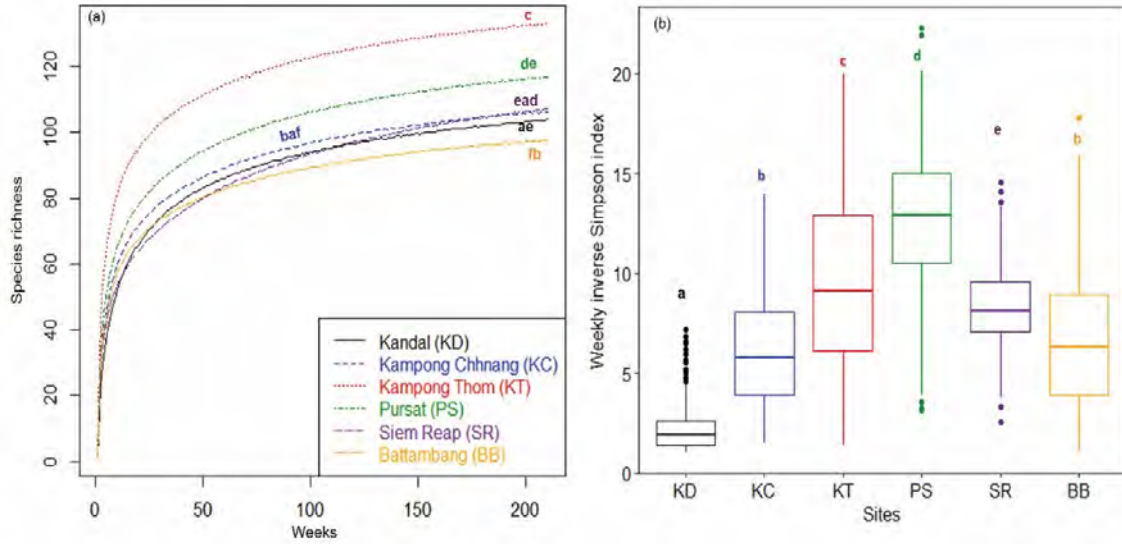
Fig. 14. Spatiotemporal comparison of site fish species richness and diversity in the Tonle Sap River and Lake: (a) site rarefaction curves on species richness; (b) site inverse Simpson index with south-north gradient along the Tonle Sap Rive and Lake. Sites with a common letter are not significantly different at p -value=0.05. For site names: KD=Kandal, KC=Kampong Chhnang, KT=Kampong Thom, PS=Pursat, SR=Siem Reap and BB=Battambang.
