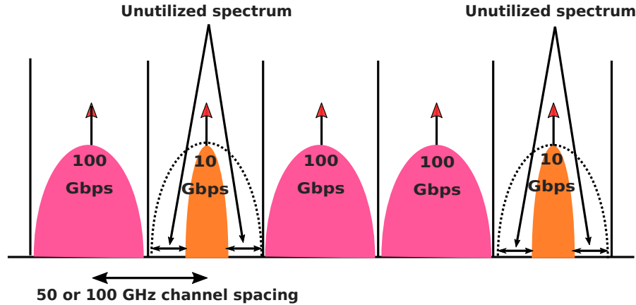
Figure 1.1: IUT-T fixed-grid [16].
