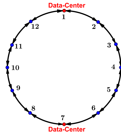
(a) Ring (12 nodes and 12 bidirectional fiber links).
