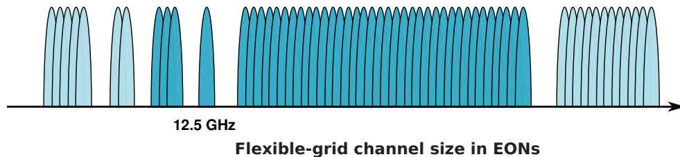
Figure 1.2: Flexible-grid in EONs [16].
