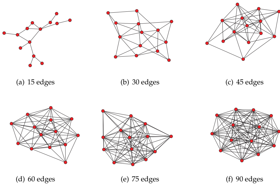
Figure 3.10: Six random graphs with 14 vertices and 15-90 edges.
