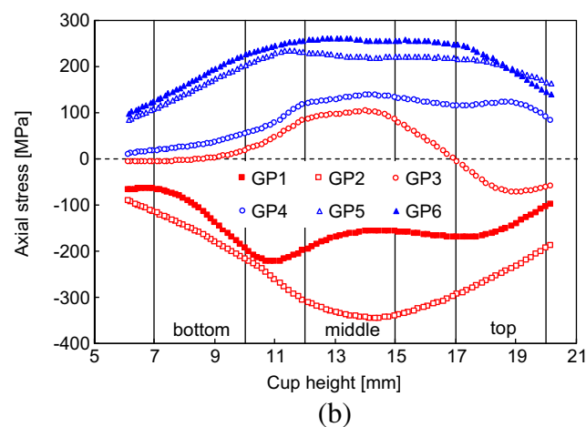
Fig. 8 Axial stress distributions along the cup wall at the end of the cup forming and unloading stage: (a) Lower gap; (b) Higher gap
