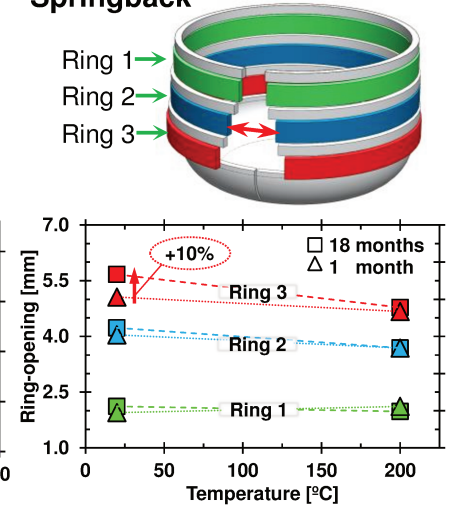
Springback
