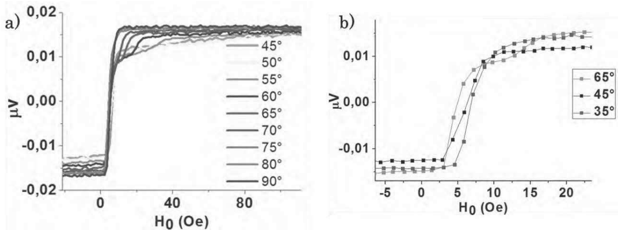
Figure 4.19: a) Evolution of the LMOKE component for sample N°1 at different angle \alpha . The field is swept from negative to positive fields. We clearly observe some “plateau” for angles between 50^\circ and 70^\circ . However, in b) the “plateaus” are absent for angles below 45^\circ .
