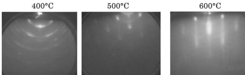
Figure 4.1: RHEED patterns of CMS at different deposition temperatures.
