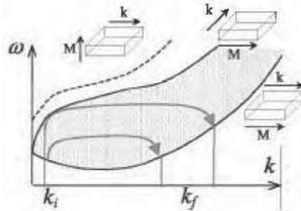
Figure 2.17: spin wave dispersion curves as a function of wave vector in the case of thin films. The gray region represents the case of tangentially magnetized thin film while the dashed line represents the case of a perpendicularly magnetized film [53 Bailleul].
