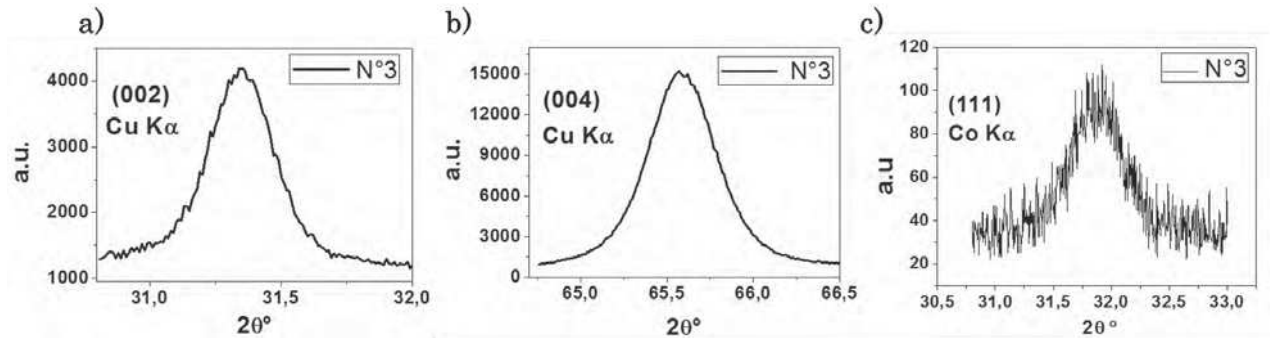
Figure 4.10: (002) and (004) diffraction peaks for sample N°3 measured with Cu K \alpha source in a) and b) respectively. c), (111) diffraction peak measured with the Co K \alpha_{1,2} source diffractometer.
