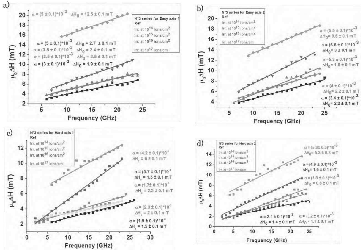
Figure 5.28: Evolution of damping coefficient and extrinsic linewidth contribution \Delta H_0 as a function of irradiation dose from \Delta H vs. f_{res} measurements for N°3 series along the two easy and two hard axes.
