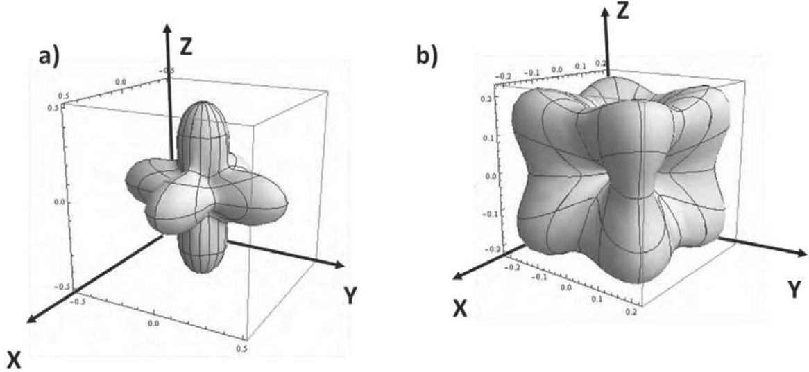
Figure 2.7: 3D presentation of the cubic anisotropy for a) K_{c1} < 0 and b) K_{c1} > 0 .
