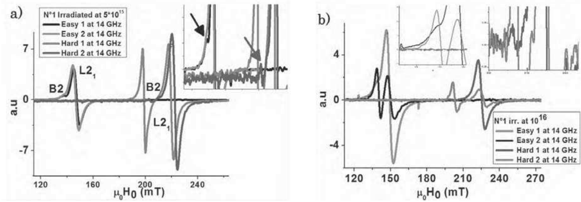
Figure 5.15: FMR absorption spectra obtained for the four easy and hard axes directions for a) N°1 irradiated at 5 \times 10^{15} and b) N°1 irradiated for 10^{16} ions/cm 2 fluence.
