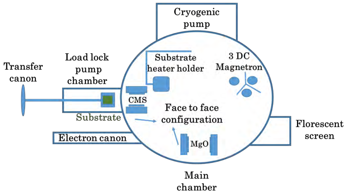
Figure 3.4: graphical representation of PLASSYS sputtering at CEMES.
