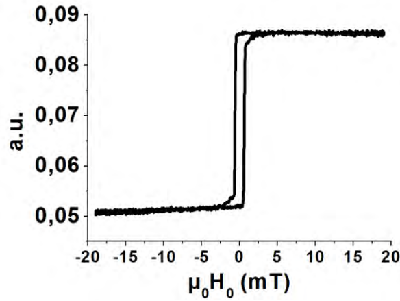
Figure 3.22: An example of Hysterises loop for LMOKE measurements.
