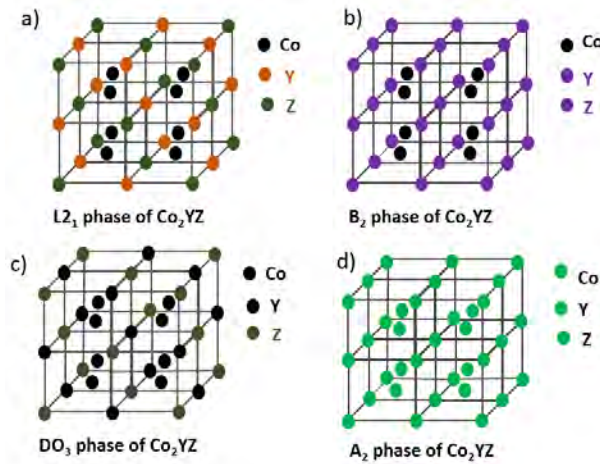
Figure 1.1: schematic presentation of \text{Co}_2\text{YZ} crystalline structure: a) \text{L}_{21} , b) \text{B}_2 , c) \text{D}_{03} and \text{A}_2 phases.
