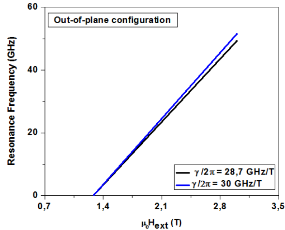
Figure 2.12: Resonance frequency as a function of an external magnetic field for out-of-plane configuration ( \theta=0^\circ ). The blue line is corresponds to \frac{\gamma}{2\pi} = 30 \text{ GHz/T} , while the black line corresponds to \frac{\gamma}{2\pi} = 28.7 \text{ GHz/T} .
