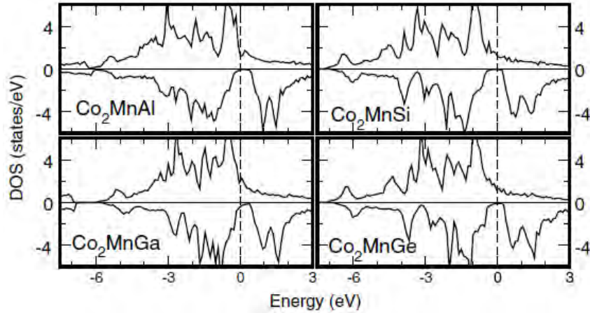
Figure 1.4: Spin resolved DOS for \text{Co}_2\text{MnZ} compounds with Z=\text{Al}, \text{Ga}, \text{Si} and \text{Ge} . Taken from [25 Galanakis].
