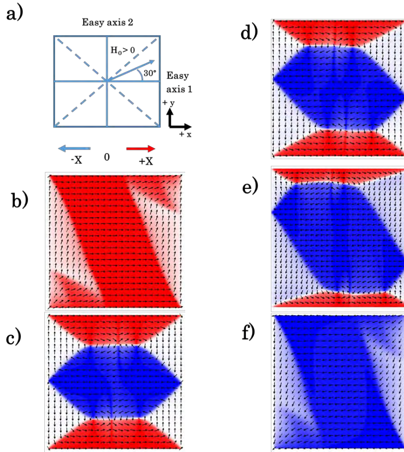
Figure 4.24: simulated switching mechanisms for fields applied at 30° from the easy axis 1. Switching from positive b) to negative f) applied field occurs through the growing of the central magnetic domain pointing in the -X direction as shown in c), d) and e).
