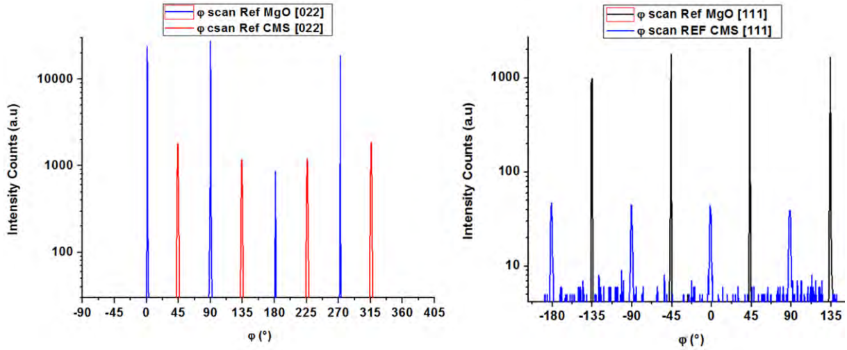
Figure 4.5: \phi scan of the CMS with respect to the MgO substrate along the [022] and [111] directions clearly shows the 45^\circ orientation.
