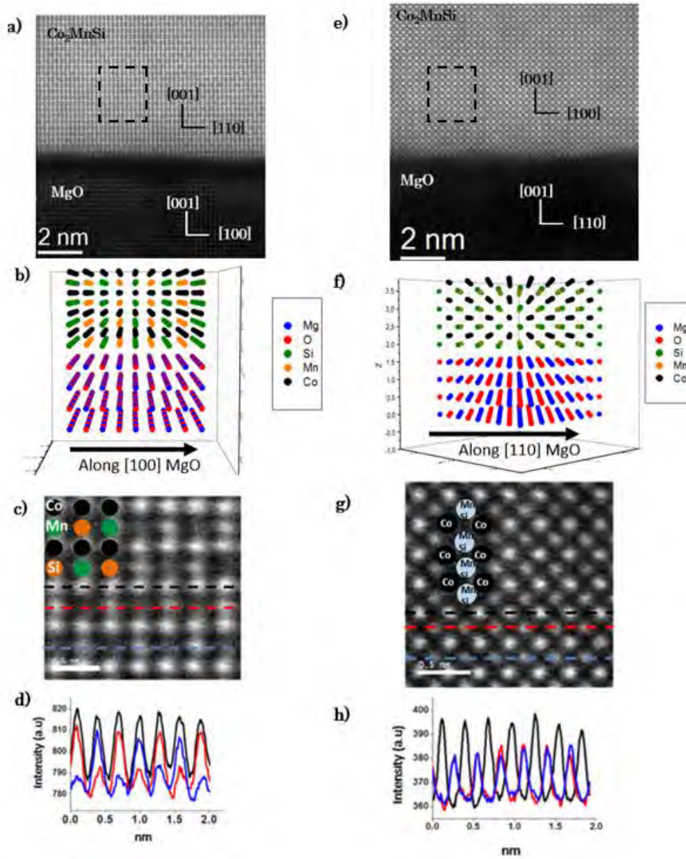
Figure 4.12: a) and e) are examples of HAADF-STEM of the reference sample N°3. b) and f) Sketched of the atomic arrangement in the different zone axis, considering the perfect \text{L2}_1 structure. c) and g) Zoom corresponding to the black boxes in a) and e) showing the Co, Mn and Si positions. d) and h) Intensity profile for the dotted lines in c) and g).
