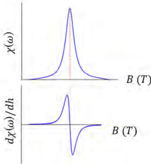
Figure 3.26: Microwave absorption and FMR derivative signal as a function of the applied external field.
