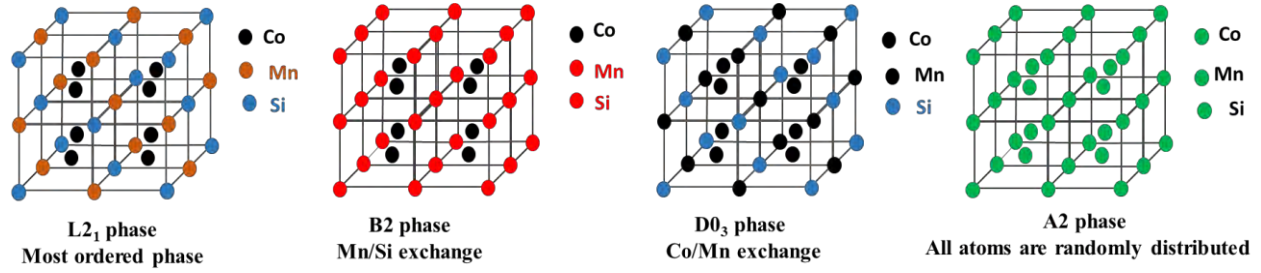
Figure 1.10: schematic presentation of Co 2 MnSi crystalline structure: a) L 21 , b) B2, c) D0 3 and A2 phases.
