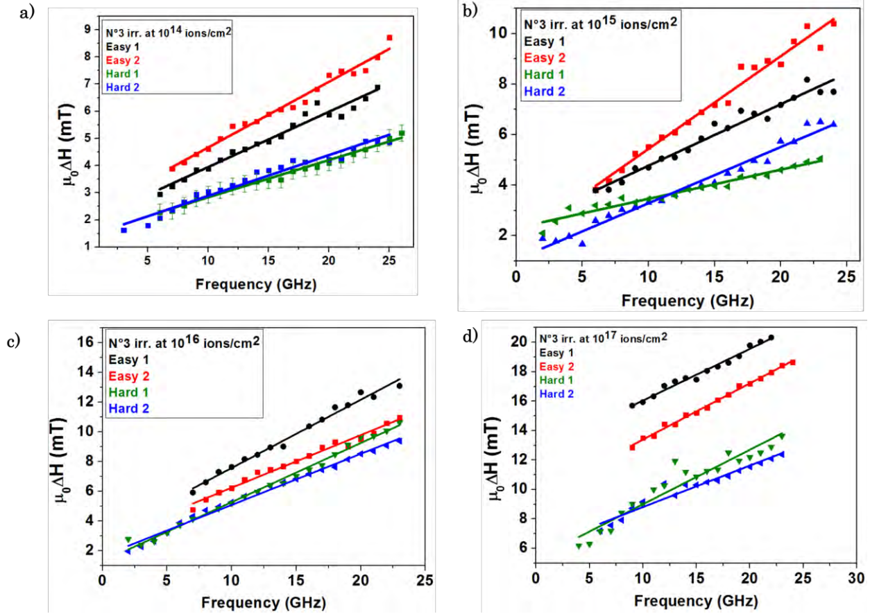
Figure 5.27: \Delta H vs. f_{res} measurements of N°3 series irradiated samples from 10^{14} to 10^{17} ions/cm 2 along the 4 axes directions shows clearly that the easy axes have higher \Delta H than hard axes.
