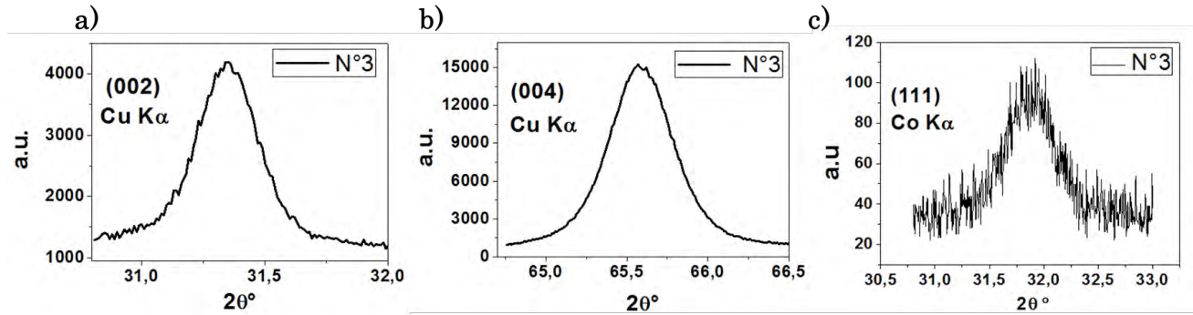
Figure 4.10: (002) and (004) diffraction peaks for sample N°3 measured with Cu K \alpha_1 source in a) and b) respectively. c), (111) diffraction peak measured with the Co K \alpha_{1,2} source diffractometer.
