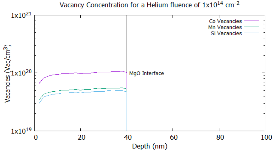
Figure 5.3: Vacancy concentration as depth or Vacancy concentration of Co,Mn and Si for 10^{14} ions/cm 2 at the Mgo/CMS interface.
