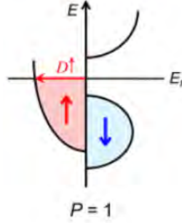
Figure 1.3: schematic presentation of the DOS of half metallic ferromagnetic, P=1 from electron's spin polarization at the Fermi level. Adapted from [24]
