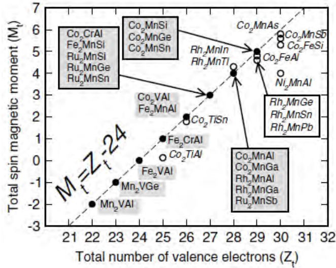
Figure 1.7: Calculated total spin moments for Heusler alloys, the dashed line represents the Slater-Pauling behavior. The open circles are deviated from the curve. Adapted from [26 Galanakis].
