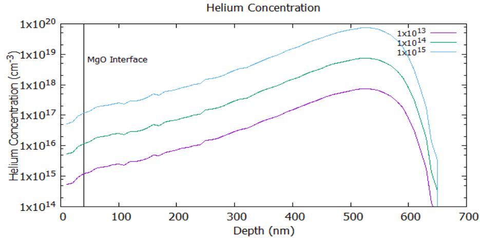
Figure 5.2: distribution of different concentration doses of \text{He}^+ ions at 150 KeV as a function of CMS layer depth.
