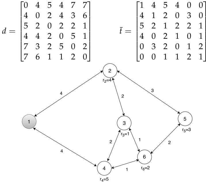
Figure 1.1 – Directed (symmetric) graph describing an instance with 6 stations, data rates r = (0, 4, 1, 5, 3, 2) , time matrix \bar{t} and distance matrix d .
