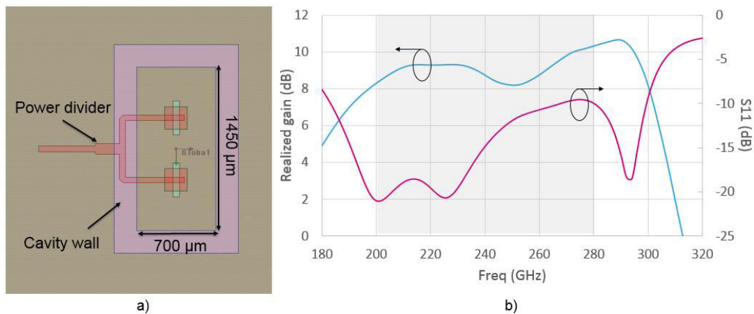
Figure III.20. (a) Final design of the divider, and (b) corresponding |S_{11}| and simulated broadside gain of the 2x1 array of patches fed by the divider.
