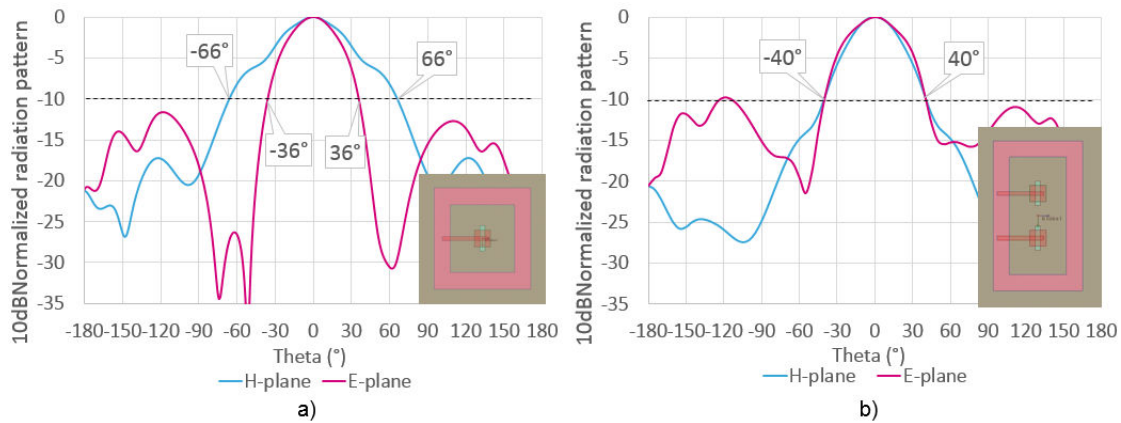
Figure III.19. (a) E-plane and H-plane normalized radiation patterns at 240 GHz with one patch, and (b) with two patches in the E-plane at 280 GHz.
