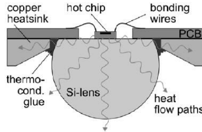
Figure III.5. Lens-packaged Tx/Rx module from [III.8].
