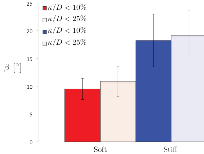
Figure 1.31: Out-centering effect. Histogram of the mean angle \pm the standard deviation, at high flow strength : for soft capsules with an off-centering lower than 10% (in dark red, n=40 ), for all soft capsules (in light red, n=51 ); for stiff capsules with an off-centering lower than 10% (in dark blue, n=12 ), for all stiff capsules (in light blue, n=33 ).
