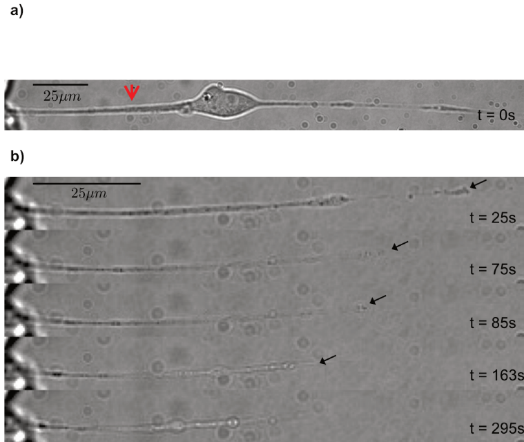
Figure 5.23: Retraction of the filament. Fluid flows from left to right. The cell is attached on VWF at the surface of a beam. (a) Picture of the cell in flow before ablation, the cell elongates with a velocity of 0.17\ \mu\text{m}/\text{s} (b) We follow the total length of the filament and noticed several ruptures of the filament. The red arrow in picture (a) shows the point of ablation. Black arrows in picture (b) indicate the points of successive ruptures. Ablation occurs after 15 seconds acquisition.
