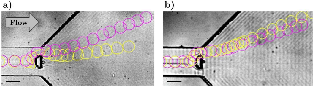
Fig. 5. Trajectory of capsules in the diverging flow chamber. Capsules were flowed at low (pink) and high (yellow) flow strengths. (a) Capsules prepared at pH 5.9. (b) Capsules prepared at pH 8. The scale bars correspond to 100 \mu m. (For interpretation of the references to color in this figure legend, the reader is referred to the web version of this article).
