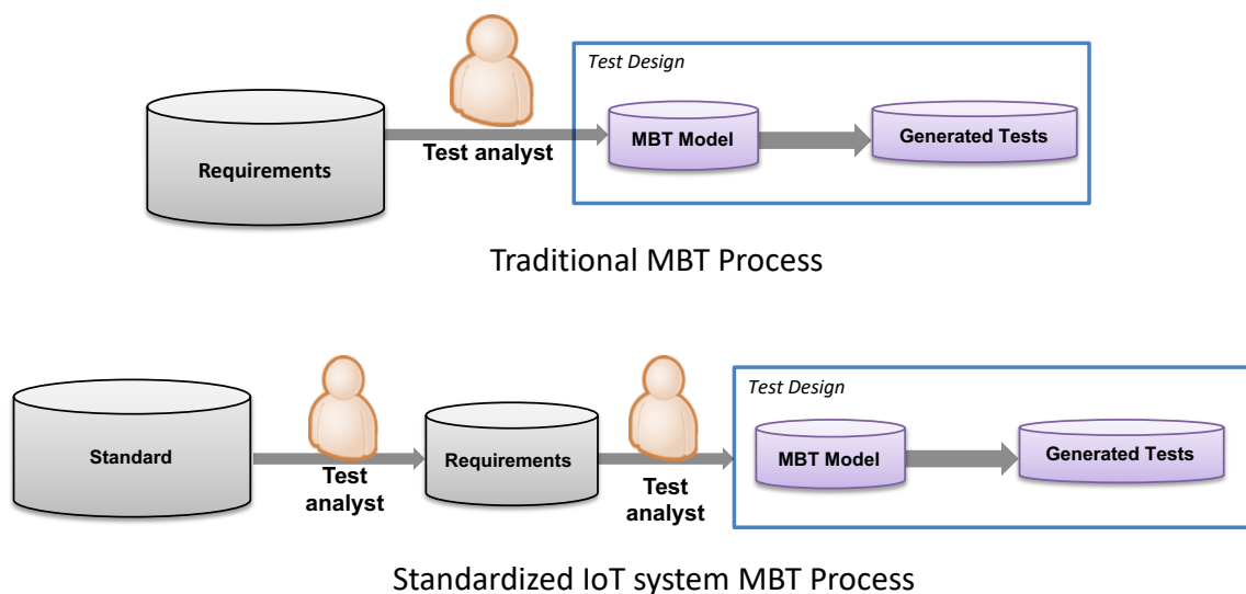
Figure 6.1: Traditional vs Standardized MBT Process
