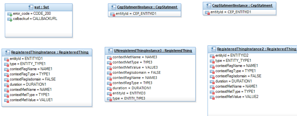
Figure 10.2: Excerpt of the Data handling object diagram
