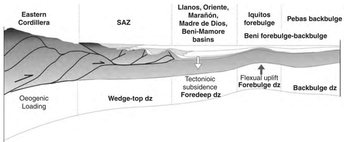
Figure 1.5. Schematic cross-section illustrating the Foreland Basin System concept sensu DeCelles & Gilles (1996) applied to subandean basins (from Roddaz et al., 2010).
