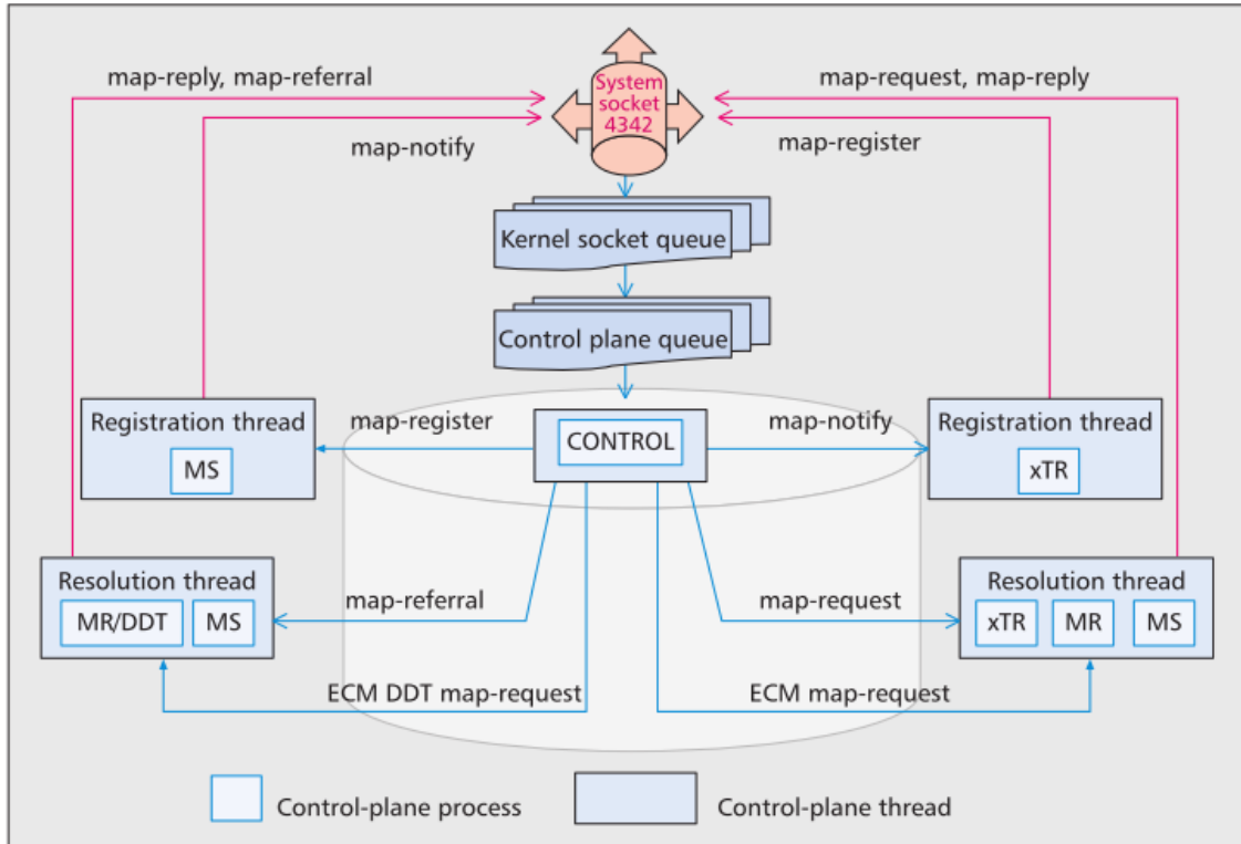
Figure 2.4: System-level OpenLISP control plane multi-thread architecture.
