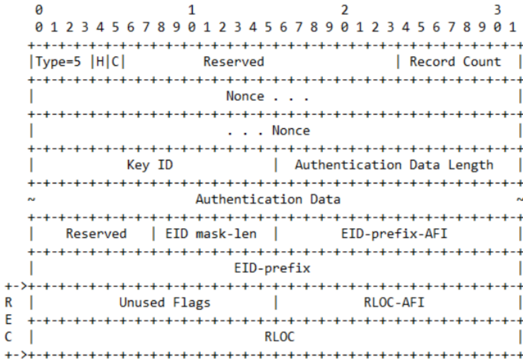
Figure 3.2: CHANGE PRIORITY message format.
