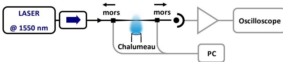
FIGURE 3.5 – Banc de fusion-étirage.
