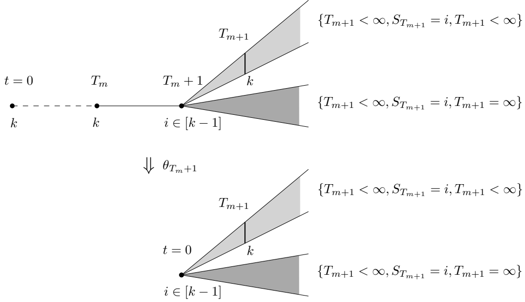
Figure 5.4 – The upper figure: The event \{S_{T_{m+1}} = i, T_m < \infty\} consists of the plays that at time T_m visit state k for the m th time without ever visiting the states > k before, and at time T_m + 1 they visit state i , where i < k . These plays are partitioned into two sets. The set \{T_{m+1} < \infty, S_{T_{m+1}} = i, T_m < \infty\} of plays that will visit k for the (m + 1) th time and the set \{T_{m+1} = \infty, S_{T_{m+1}} = i, T_m < \infty\} of the plays for which the m th visit in k was the last one. The lower figure : The shift mapping \theta_{T_{m+1}} “forgets” all the history prior to the time T_m + 1 .
