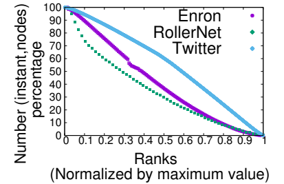
Figure 3.10: Inverse cumulative distribution of ranks attributed by Temporal Closeness during temporary inactive moments.
