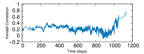
Figure 3.8: Evolution of the Kendall tau correlation between Temporal Closeness and Coverage over time on Enron dataset.
