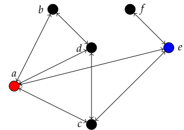
Figure 1.1: A toy example of a graph.
