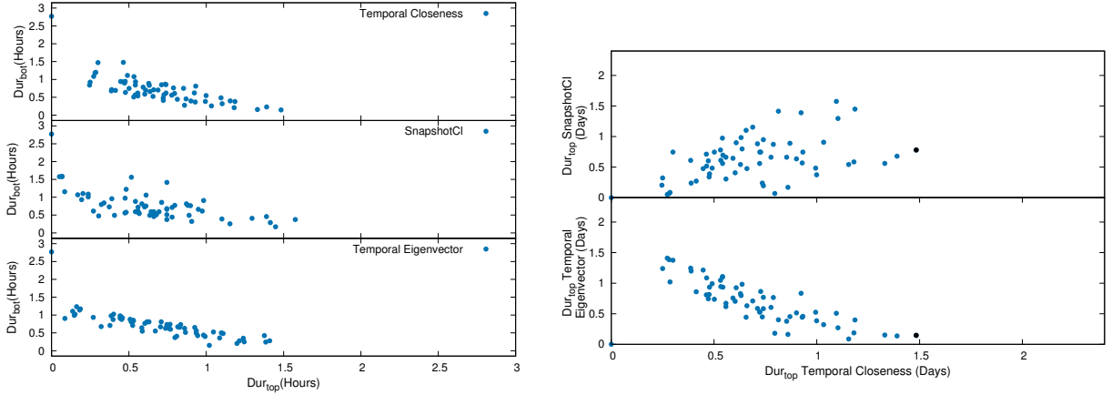
Figure 3.13: Left: For each node, the Dur_{top} and dur_{bot} values attributed by each method on the RollerNet dataset. Right: For each node the Dur_{top} value attributed by Temporal Closeness versus the Dur_{top} attributed by the other methods on the RollerNet dataset.
