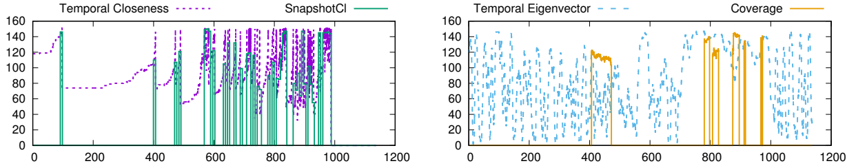
Figure 3.11: Evolution of ranks attributed by the four methods over time for a randomly selected node.
