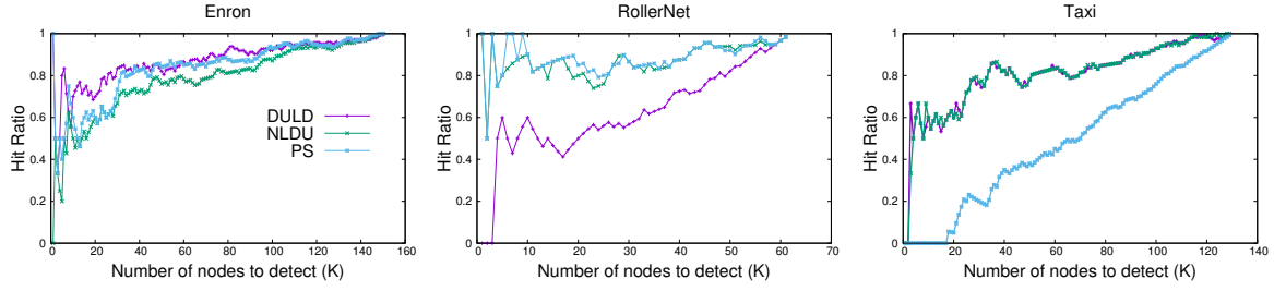
Figure 4.6: Evolution of the \text{hitratio} as a function of k for 3 datasets: Enron; RollerNet; Taxi.
