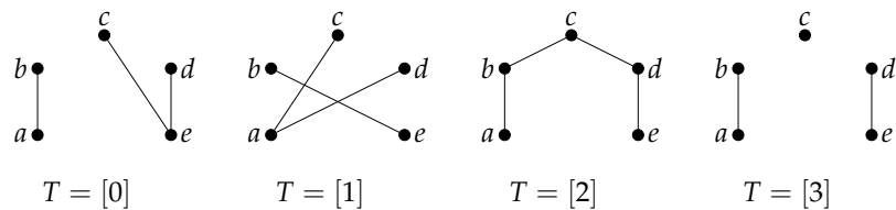
Figure 1.4: A representation of a dynamic graph in the form of 4 snapshots representing each 1 instant.
