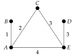
Figure 3.1: A toy example of a dynamic graph. The labels on the links indicate the instant in which the link occurs.
