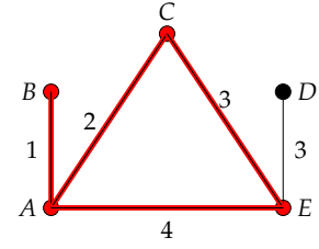
Figure 5.1: A toy example of a dynamic graph. The labels on the links indicate the instant in which the link occurs. In bold red the subgraph induced by the node A as an ego node.
