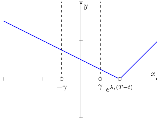
Figure 3.2 – Graph of function y = |e^{\lambda_i(T-t)} - x| when \gamma < e^{\lambda_i(T-t)} .
