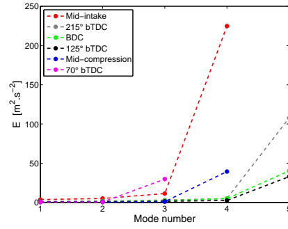
Figure 6.38: Energy contents as function of the EMD mode for the 6 instantaneous velocity fields.
