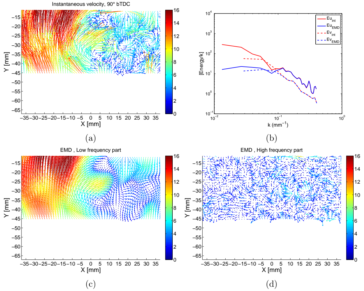
Figure 6.43: Results of EMD analysis, Mid-compression stroke, Cycle 10 (1400 rpm), Slow transient condition.
