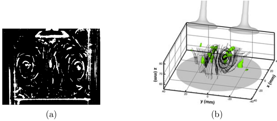
Figure 1.3: Two mean ring-vortices generated under inlet valves; (a) by hydraulic analogues in a IC engine, from Ekhian & Hoult (1979) [45], (b) by Stereoscopic PIV in a DISI engine, from Bücker et al. (2012) [20].
