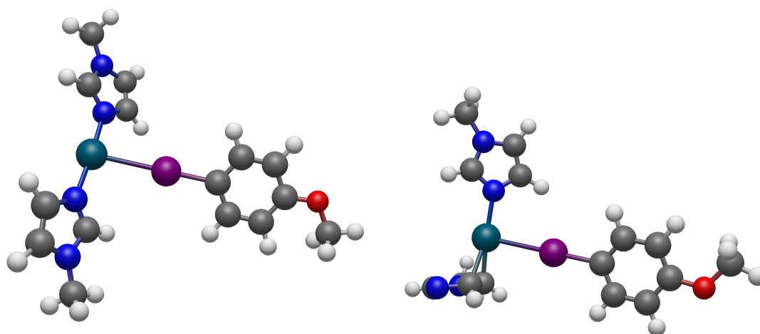
FIGURE II.28 – Structures des complexes (4-OMe-C 6 H 4 -I)-Pd(κ 1 -mim) 2 et (4-OMe-C 6 H 4 -I)-Pd(κ 1 -mim)(η 2 -mim).
