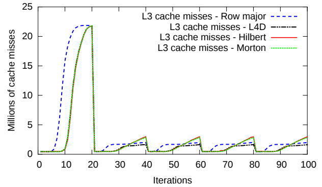
Figure 2.9: Millions of cache misses per iteration for the cache level 3 during the update-velocities and accumulate loops. Architecture: Haswell
