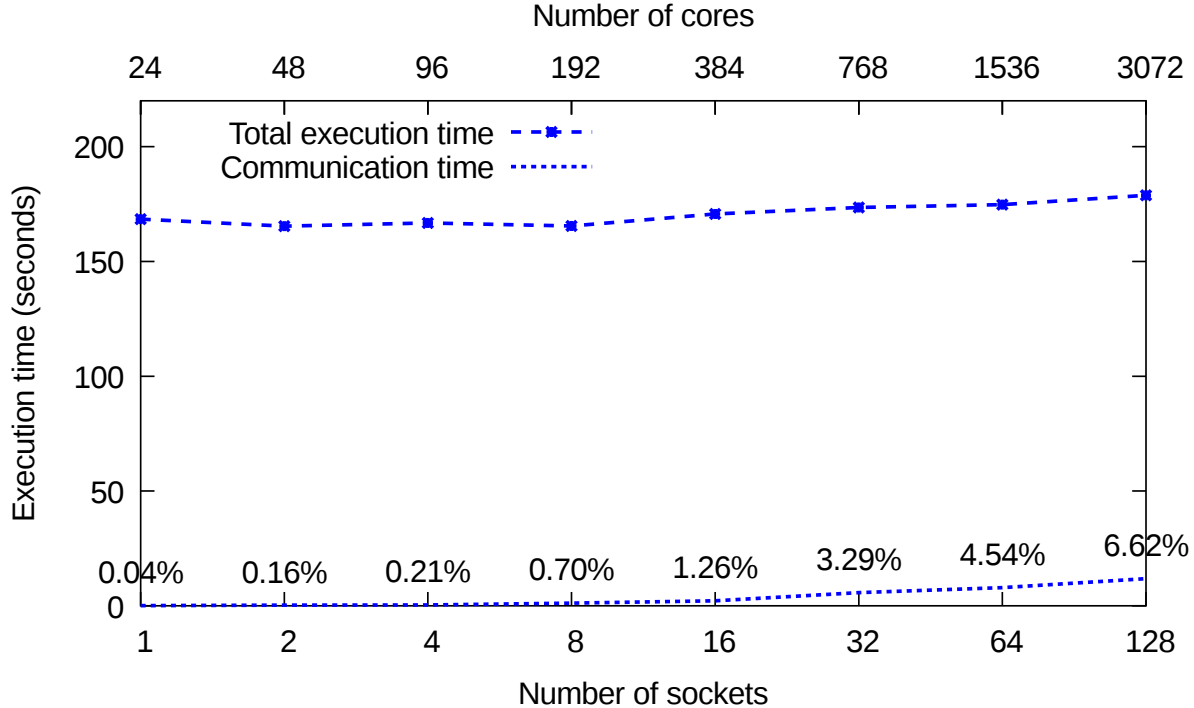
Test case: 64 \times 64 \times 64 grid, 1 billion particles per socket, 100 iterations simulation (sorting every 10 iterations). Architecture: Skylake. Communication time is shown as percentage of the execution time.
