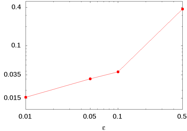
Figure 2.1: The global relative error at time t = 5 (in the L^2 norm) of the density of the Vlasov–Poisson solution of (2.3) with respect to the guiding center solution of (2.4), as function of \varepsilon .
