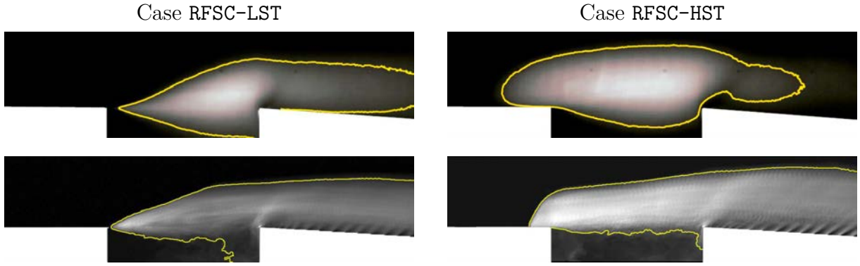
Figure 7.21 – Comparison with experimental data: flame luminosity adapted from Micka [116] (top) and average heat release rate (bottom)
