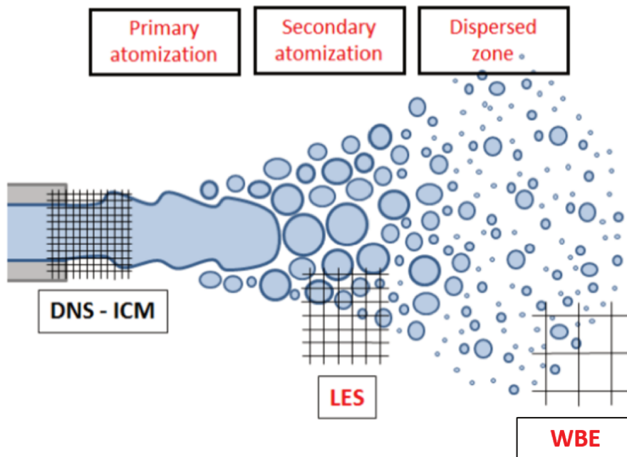
Figure 2.3: Atomization zones.
