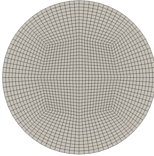
Figure 3.19: Discretized liquid inlet patch. [18].
