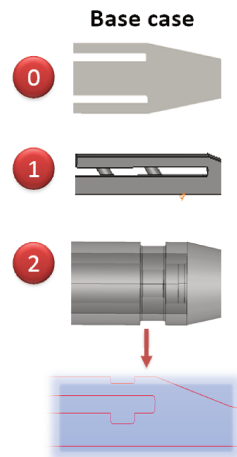
Figure 5.13: Proposal modifications within the premixing zone.
