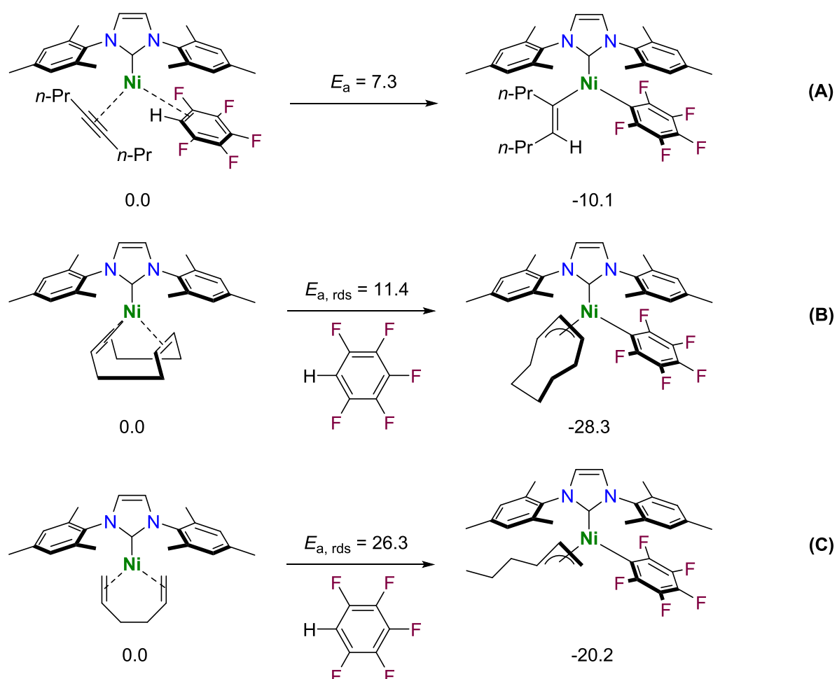
Scheme 16. DFT computed products from the reaction of [Ni 0 (NHC-Mes 2 )(L)] (L = 4-octyne ( A ), 1,5-cyclooctadiene ( B ), 1,5-hexadiene ( C )) complexes and C 6 F 5 H. Values correspond to Gibbs free energy, E_a corresponds to the Gibbs energy connecting transition state, E_{a, rds} corresponds to the Gibbs energy of the rate-determining step, all energies presented in kcal mol -1 .
