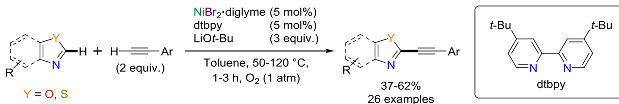
Scheme 56. Ni-catalyzed C–H/C–H oxidative coupling of benzoxazoles and terminal alkynes under an oxygen atmosphere.
