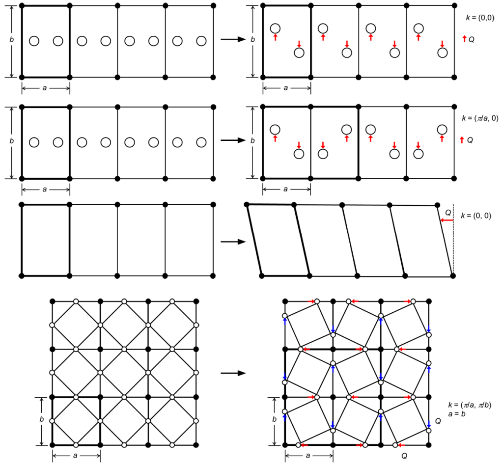
Figure 2-4 Examples of order parameter Q (on 2D lattice); k is the propagation vector of high symmetry phase. (81)
