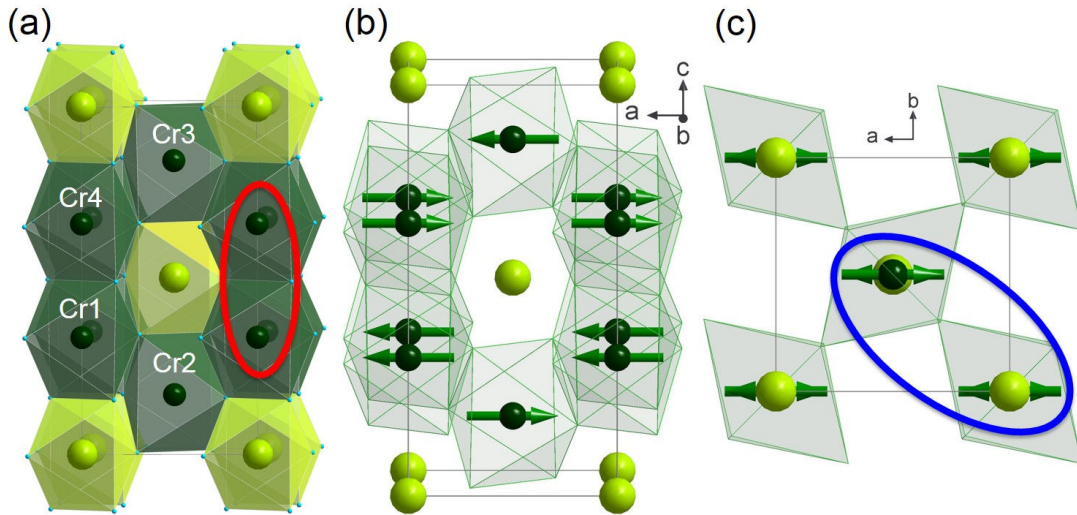
Figure 4-6 (a) Structure of Cr_2TeO_6 with the labels corresponding to the four (symmetrically equivalent) Cr-sites. The red ellipse shows the magnetic bi-unit made of two edge-sharing octahedra, while the blue ellipse shows corner sharing octahedra. Magnetic structure of Cr_2TeO_6 ( I_9 with \psi_1 ) projected along (b) [010] and (c) [001]
