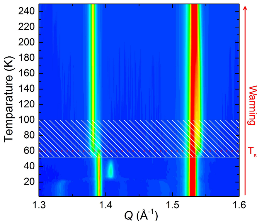
Figure 3-37 Temperature evolution of the NPD patterns of \text{Mn}_2\text{TeO}_6 (S2 sample), in a selected Q range, from 1.5 to 250 K upon warming (WISH@ISIS). The dashed area corresponds to the two-phase temperature range. The horizontal red dot line indicates T_s .
