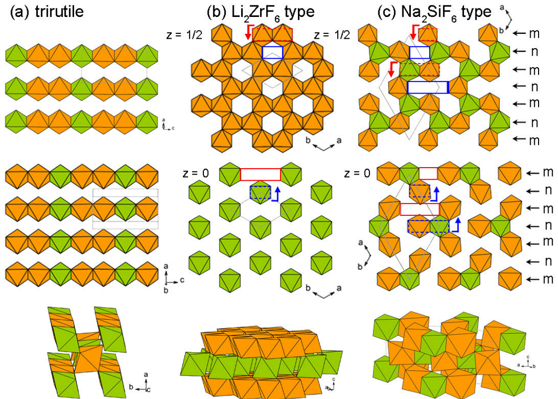
Figure 5-3 Drawing of the structures (lower panel) and showing each time only one octahedral layer (higher and middle panels) (a) inverse trirutile ( P4_2/mnm ), (b) honeycomb with P31m and (c) honeycomb with P321 from (157). In (b) and (c), red and blue arrows show cation shifts layer to layer ( z = 0 \leftrightarrow z = 1/2 ) to highlight the relationship between structures. Cations move from dot rectangles to solid rectangles.
