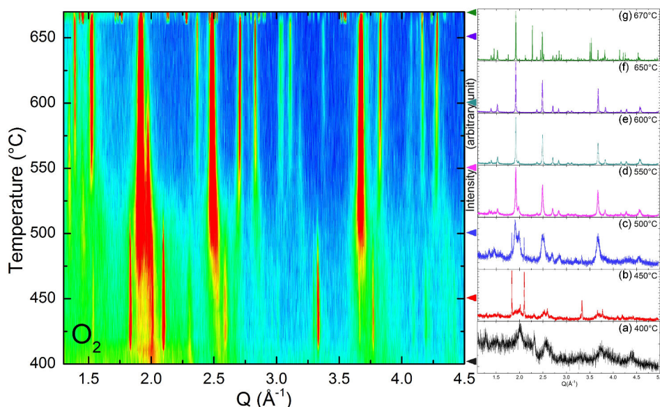
Figure 3-2 In-situ XRPD patterns of the Mn, Te, O system as a function of temperature in O 2 , from 400 to 670°C. Selected diffraction patterns are presented on the right side.
