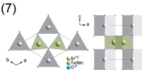
Figure 1-5 Polyhedral representation of known structures in the \text{ABTeO}_6 family
