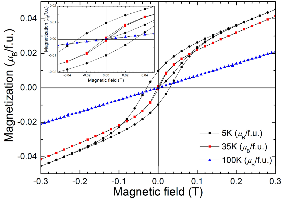
Figure 4-16 Magnetic field dependence of the magnetization of \text{Cr}_{0.025}\text{Mn}_{1.975}\text{TeO}_6 recorded at 5, 35, and 100 K. Hysteresis features are seen in the MH curve at 5 and 35 K. The inset shows the enlargement of the selected range.
