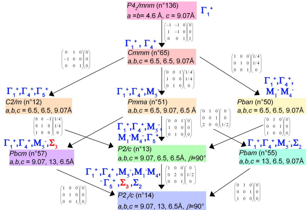
Figure 3-15 Symmetry relations for the transformation from P4_2/mnm to P2_1/c via five possible subgroup paths. The irrep labels (blue) indicate the active irrep components of each subgroup. \Sigma_3 is highlighted in red. Numbers in brackets denote SG numbers according to the international tables for crystallography. Corresponding cell parameters and transformation matrixes, which relate the coordinate system of the subgroup to that of the super-group, are also given.
