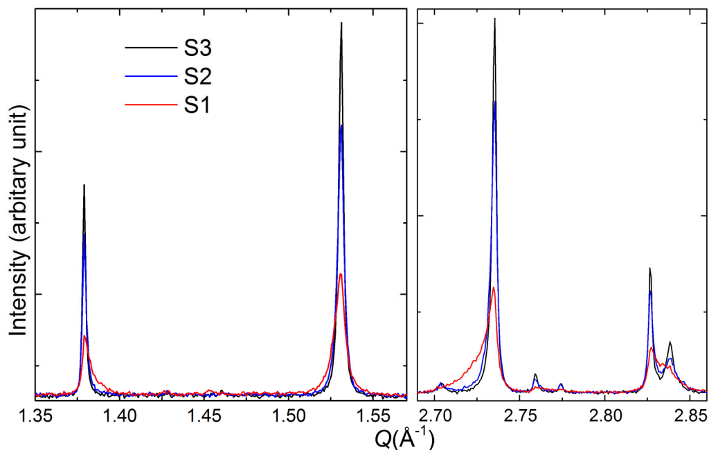
Figure 3-6 SXRPD patterns (in selected Q -ranges) of the three \text{Mn}_2\text{TeO}_6 samples
