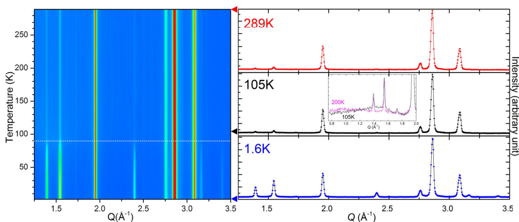
Figure 4-4 (left) Temperature evolution of the NPD (G4.1@LLB) patterns of Cr 2 TeO 6 , in the 1.25\text{--}3.5 \text{\AA}^{-1} selected Q range (from 1.6 to 289 K). The horizontal white dot line indicates the magnetic transition at 90K. (right) NPD data of Cr 2 TeO 6 at 289, 105 and 1.6K, the inset on the pattern at 105K emphasizes the diffuse scattering signal observed at this temperature.
