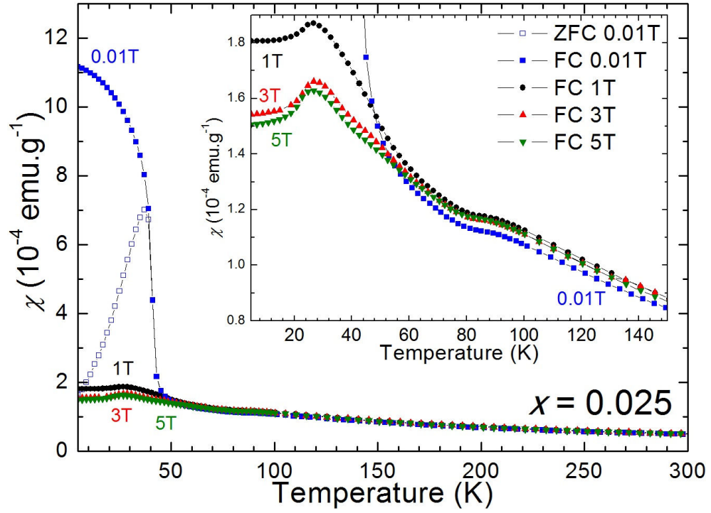
Figure 4-15 Temperature dependence of the magnetization curves (zfc, fc) of \text{Cr}_{0.025}\text{Mn}_{1.975}\text{TeO}_6 in an applied field of 0.01, 1, 3 and 5 T.
