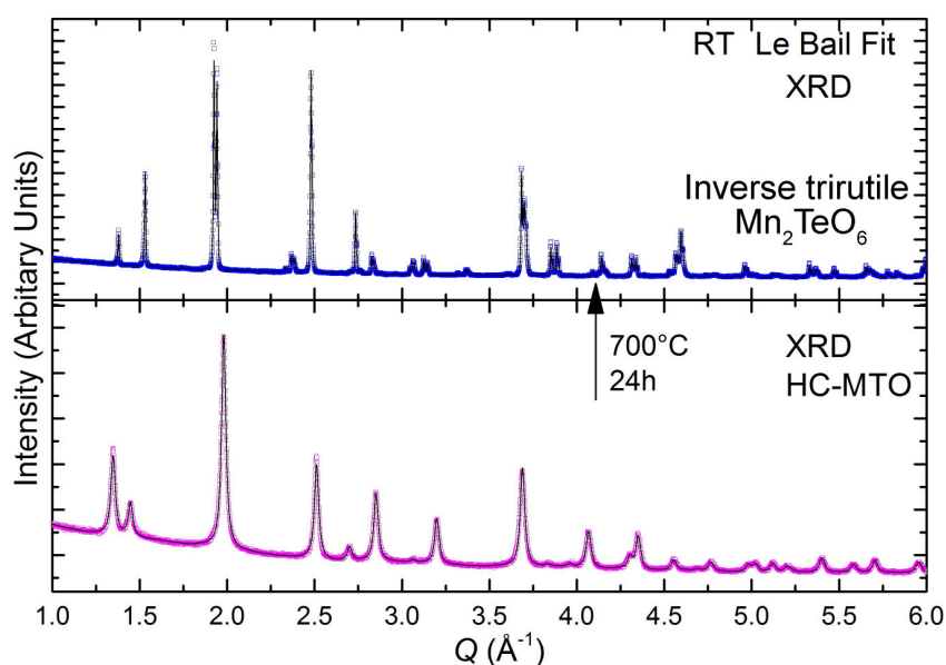
Figure 5-2 Le Bail fits of the XRPD patterns of the HC-MTO phase and the inverse trirutile \text{Mn}_2\text{TeO}_6 recorded at RT. The HC-MTO pattern is indexed in the trigonal structure (SG: P\bar{3}1m with a \cong 5.00 \text{ \AA} , c \cong 4.65 \text{ \AA} and \gamma = 120^\circ ), while the inverse trirutile \text{Mn}_2\text{TeO}_6 pattern is indexed in the RTM structure (SG: P2_1/c with a \cong 9.10 \text{ \AA} , b \cong 13.05 \text{ \AA} , c \cong 6.47 \text{ \AA} and \beta \cong 90.07^\circ )
