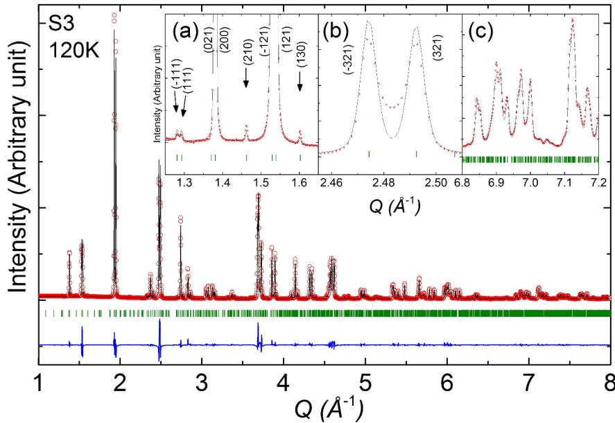
Figure 3-33 Rietveld refinement of the SXRPD data of \text{Mn}_2\text{TeO}_6 (S3 sample) at 120K in P2_1/c with a = 9.101 \text{ \AA} , b = 13.035 \text{ \AA} , c = 6.453 \text{ \AA} and \beta = 90.64^\circ . The insets show chosen Q ranges to highlight (a) small peaks corresponding to the doubling along b (compared with the HTT phase), (b) Bragg peaks characteristic of the monoclinic distortion, (c) the quality of the fit at high angles.
