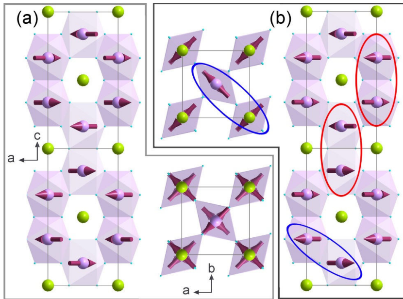
Figure 3-41: Views along b and c -axis of the magnetic model for the tetragonal \text{Mn}_2\text{TeO}_6 ; as proposed by Fruchart (7) in (a) and derived from the \Gamma_3 representation in (b) The red ellipses show the magnetic bi-unit made of two edge-sharing octahedra, while the blue ellipse show corner sharing octahedra.
