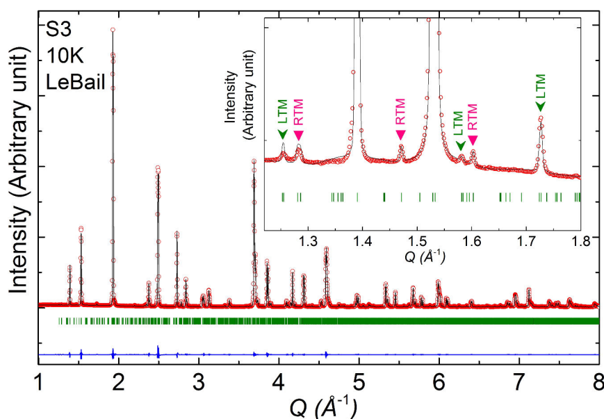
Figure 3-36 Le Bail fit of the SXRPD data of \text{Mn}_2\text{TeO}_6 at 10K. The inset shows a Q -range chosen to show the small peaks (pink arrows: RTM-like b doubling, green arrows: LTM), indexed in the monoclinic structure ( P2_1/c , a = 9.0386 (1) Å, b = 13.0498 (1) Å, c = 6.5048 (1) Å, \beta = 90.285 (1) °) with \mathbf{k} = (1/2 \ 0 \ 1/4) .
