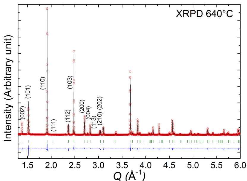
Figure 3-9 Rietveld refinement of the Mn_2TeO_6 structure from XRPD data recorded at 640^\circ\text{C} using P4_2/mnm : experimental data (open red circles); calculated pattern (black line); allowed Bragg reflections (green vertical marks). The difference between the experimental and calculated profiles is displayed at the bottom of the graph as a blue line. In following sections, unless otherwise mentioned, Rietveld refinements of powder diffraction patterns will be described in this manner.
