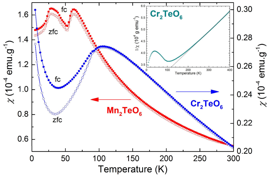
Figure 4-3 Magnetic susceptibility vs. temperature curves (zfc and fc) for (left axis) Mn_2TeO_6 in 100Oe and (right axis) Cr_2TeO_6 in 3000Oe. The inset shows the corresponding \chi^{-1}(T) curve of Cr_2TeO_6 . The black dot line is for the Curie-Weiss fitting.
