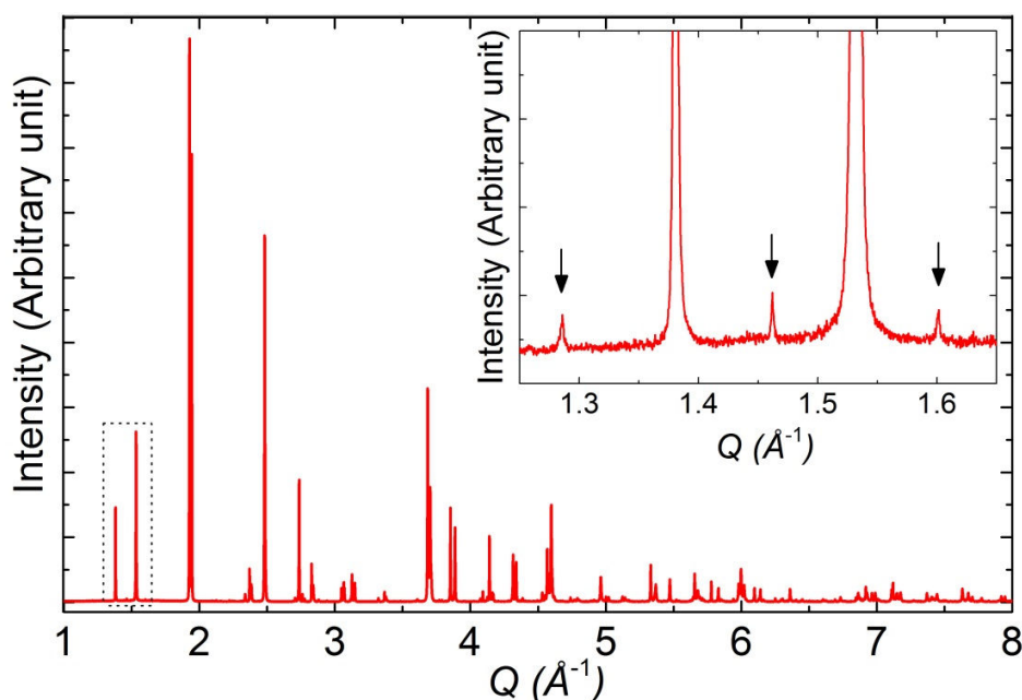
Figure 3-14 SXRPD data (CRISTAL, SOLEIL) of \text{Mn}_2\text{TeO}_6 at RT. The inset shows an enlarged view of extra peaks induced by the doubling of the b parameter (with respect to the HTT form).
