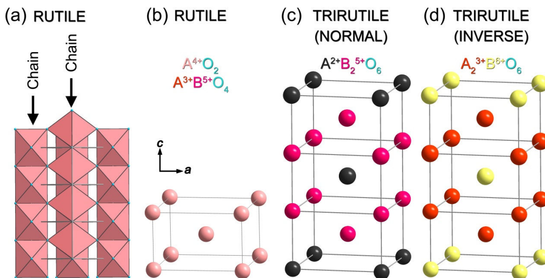
Figure 1-1 Dra wing of rutile-type structures (only cations are shown) and O_6 octahedra for the (a) panel.
