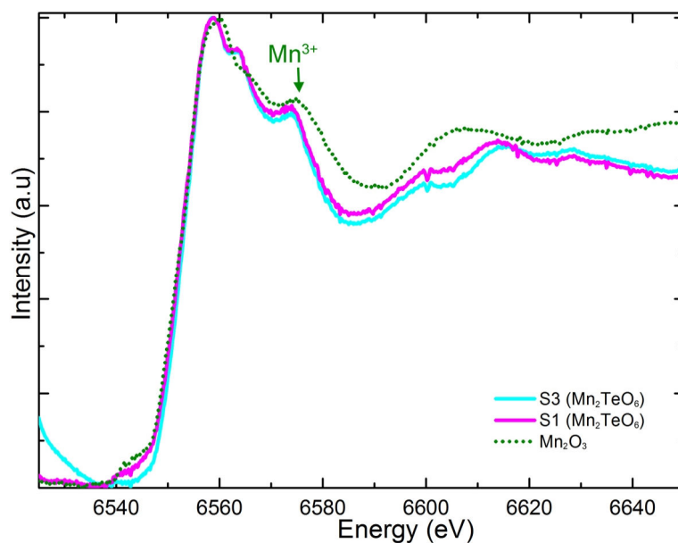
Figure 3-25 Mn K-edge XANES spectra of \text{Mn}_2\text{TeO}_6 (S3 and S1) and \text{Mn}_2\text{O}_3 as a reference sample for \text{Mn}^{3+} at RT. The highest absorbance of each spectrum was normalized to unity.
