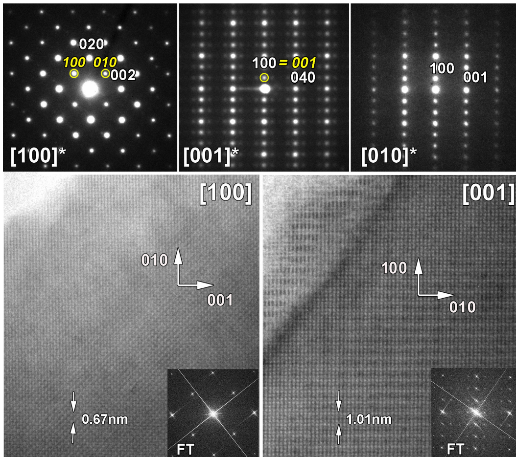
Figure 3-20 SAED patterns along the main zone axes [100] , [001] , and [010] and corresponding [100] and [001] HRTEM images and associated FT patterns. The indexing corresponds to the RTM (white) and HTT (italic yellow) structures.
