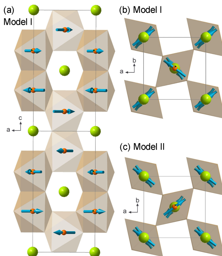
Figure 4-14 Models of magnetic structures for \text{Cr}_{0.2}\text{Mn}_{1.8}\text{TeO}_6 projected along (a) [010] and (b) [001] .
