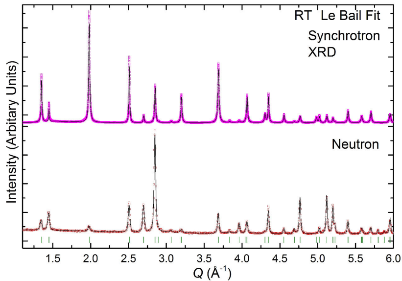
Figure 5-1 Le Bail fitting of the SXRPD (CRISTAL@Soleil) and NPD (D2B@ILL) data of HC-MTO phase recorded at RT. Both patterns are indexed in a trigonal structure (SG: P\text{-}31m with a \cong 5.00\text{\AA} , c \cong 4.65\text{\AA} and \gamma = 120^\circ )
