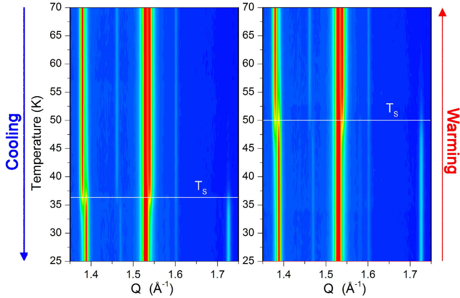
Figure 3-31 Temperature evolution of the SXRPD data of \text{Mn}_2\text{TeO}_6 (S3 sample) recorded from 70 to 25K (cooling) and from 25 to 70K (warming) in temperature sweeping mode.
