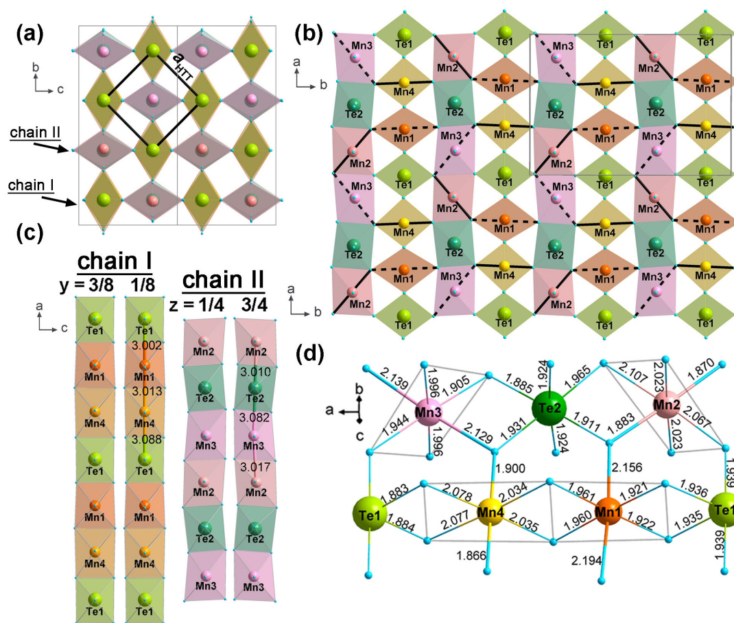
Figure 3-19 Representation of the P2_1/c distorted inverse trirutile structure of \text{Mn}_2\text{TeO}_6 at RT projected (a) along [100] , (b) along [001] and (c) along [010] and [001] . The parent HTT cell is shown in (a) as a black line. In (b) both types of chains are represented, and the full/dotted black lines highlight the compressed/elongated Mn–O distances of the \text{MnO}_6 octahedra. For clarity, only one type of chain is shown in each projection in (c). (d) Mn–O and Te–O interatomic distances (Å) are given for each of in the six octahedra building \text{Mn}_2\text{TeO}_6 .
