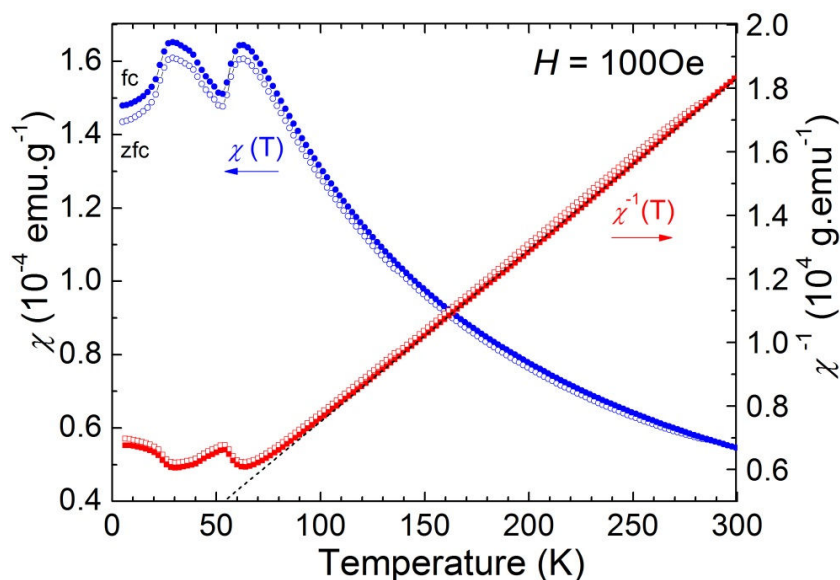
Figure 3-26 Zero field-cooling warming (zfcw) and field-cooling warming (fcw) \chi(T) curves (left axis) of \text{Mn}_2\text{TeO}_6 (S2 sample) and \chi^{-1}(T) (right axis) in 100 Oe. The dotted black line show the linear fit to a Curie-Weiss regime.
