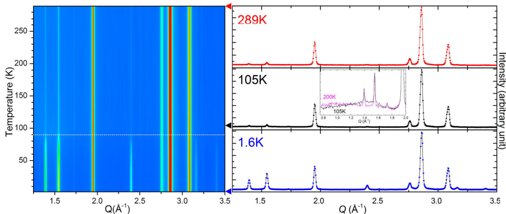
Figure 4-4 (left) Temperature evolution of the NPD (G4.1@LLB) patterns of \text{Cr}_2\text{TeO}_6 , in the 1.25\text{--}3.5\text{ \AA}^{-1} selected Q range (from 1.6 to 289 K). The horizontal white dot line indicates the magnetic transition at 90K. (right) NPD data of \text{Cr}_2\text{TeO}_6 at 289, 105 and 1.6K, the inset on the pattern at 105K emphasizes the diffuse scattering signal observed at this temperature.
