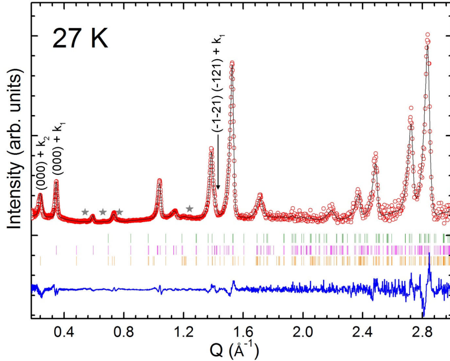
Figure 3-39 Le Bail fitting of the LT crystal structure of \text{Mn}_2\text{TeO}_6 at 27 K (WISH): P2_1/c with a = 9.0354 \text{ (2) \AA} , b = 13.0478 \text{ (3) \AA} , c = 6.5039 \text{ (1) \AA} , \beta = 90.2302 \text{ (2) }^\circ and the magnetic peaks indexed with \mathbf{k}_1 = (1/2 \ 0 \ 0) and \mathbf{k}_2 = (0 \ 1/2 \ 0) . Weak additional magnetic peaks are outlined by grey stars.
