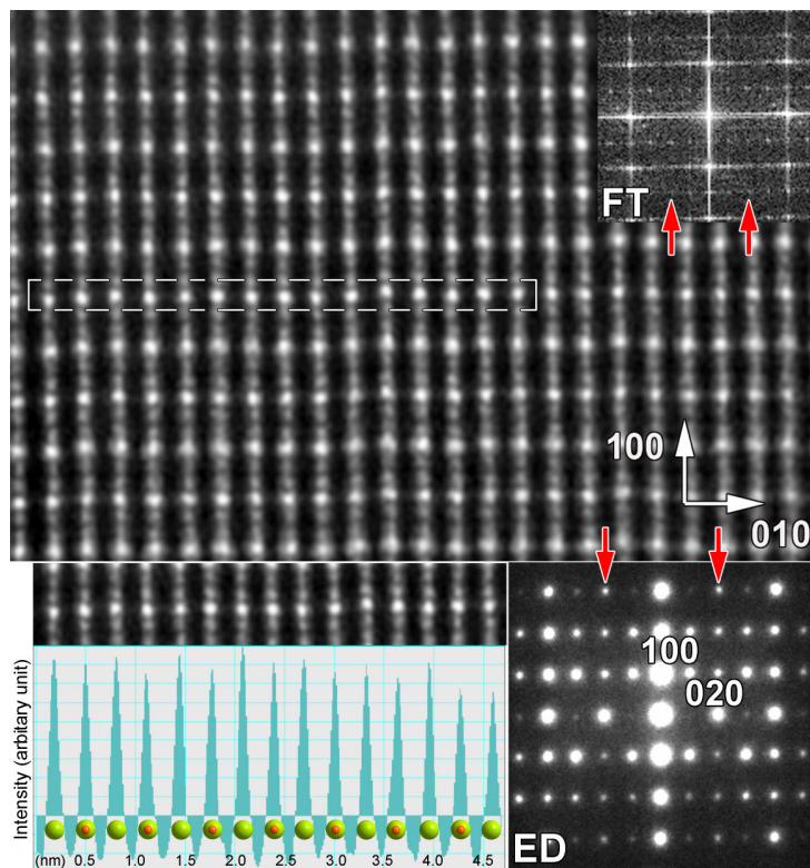
Figure 3-22 [001] HAADF-STEM image highlighting the area corresponding to the 020 spots in the FT and ED patterns (red arrow). The intensity plot profile along the Te row of the selected area (white rectangle) is also given in insert.
