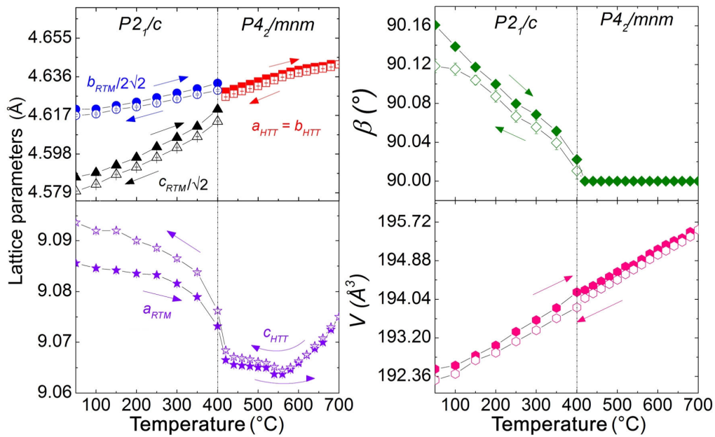
Figure 3-24 Temperature evolution between RT and 700°C of the lattice parameters and cell volume of \text{Mn}_2\text{TeO}_6 , from NPD data upon heating (full symbols) and cooling (open symbols).
