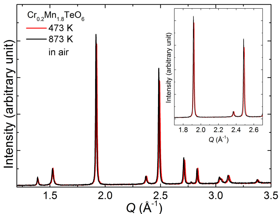
Figure 4-8 Laboratory XRPD patterns of \text{Cr}_{0.2}\text{Mn}_{1.8}\text{TeO}_6 at 473K (red line) and 873K (black line) in air.
