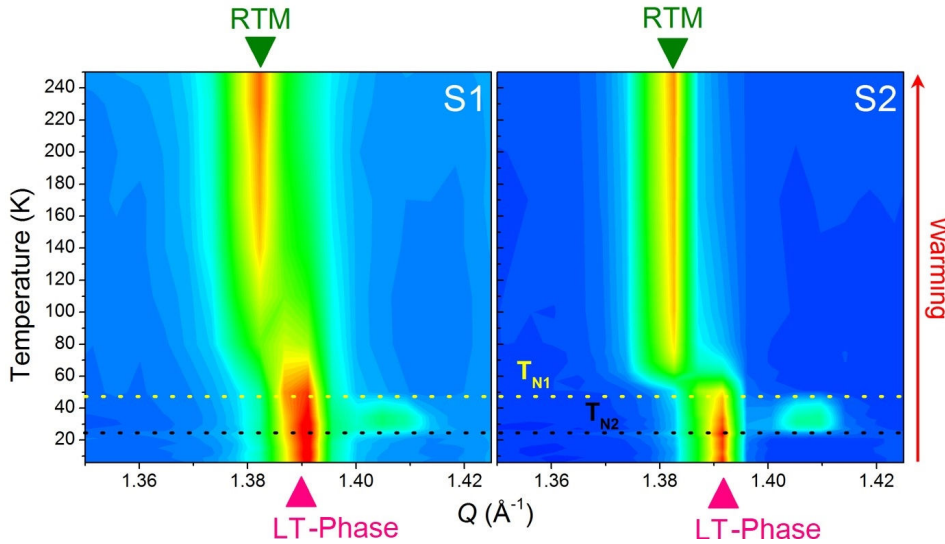
Figure 3-45 Temperature evolution (from 6 to 250K) of the NPD patterns (selected Bragg peaks) of \text{Mn}_2\text{TeO}_6 (Left: S1, Right: S2 sample) recorded upon warming. Green triangles (top of figure) and pink triangles (bottom of figure) point out Bragg peaks belonging to RTM and LT phase, respectively. The horizontal yellow and black dotted lines indicate the T_{N1} and T_{N2} magnetic transition, respectively.
