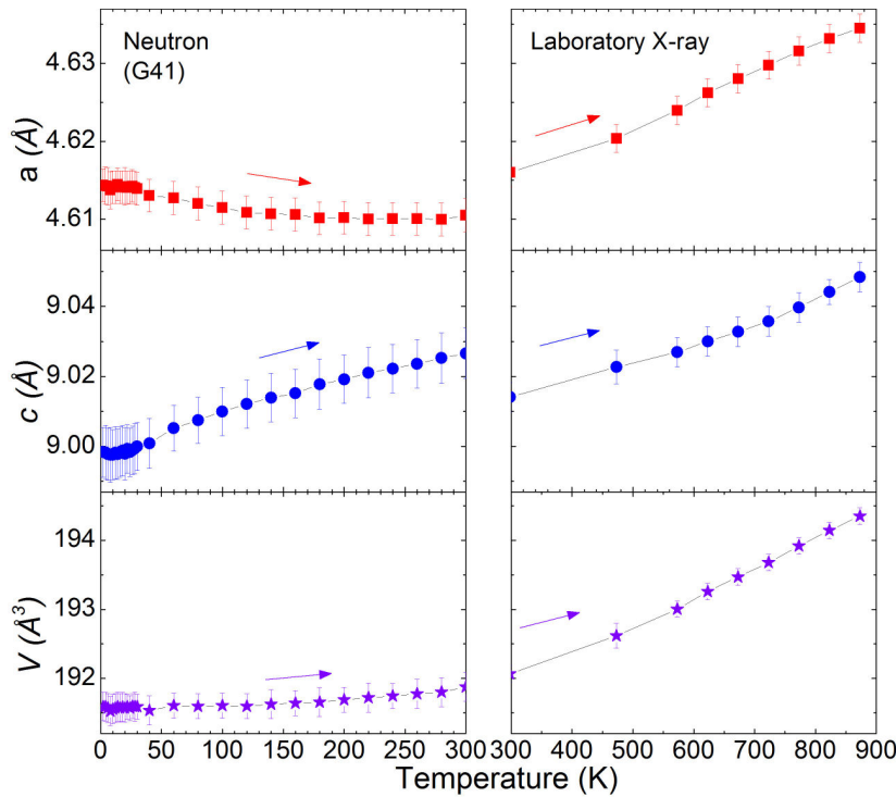
Figure 4-11 Temperature evolution of the lattice parameters and cell volume of Cr_{0.2}Mn_{1.8}TeO_6 obtained from Le Bail fitting of laboratory XRPD data recorded in air (right, from 300 to 873K) and NPD (G4.1@LLB) data (left, 2K to 300K) upon warming. Characterized samples and measurement conditions are not same, explaining the discrepancy at 300K between the two plots.
