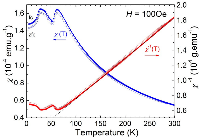
Figure 3-26 Zero field-cooling warming (zfcw) and field-cooling warming (fcw) \chi(T) curves (left axis) of Mn_2TeO_6 (S2 sample) and \chi^{-1}(T) (right axis) in 100 Oe. The dotted black line show the linear fit to a Curie-Weiss regime.
