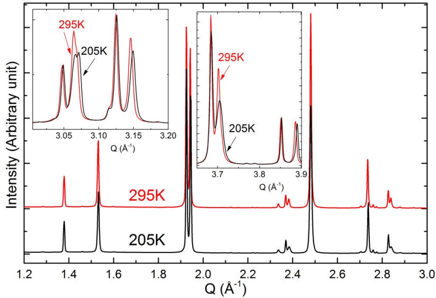
Figure 3-30 SXRPD data of Mn_2TeO_6 (S3 sample) at 295 and 205K in the 1.2 - 3.0 \text{ \AA}^{-1} Q range and in insets selected Bragg peaks at higher- Q ranges.
