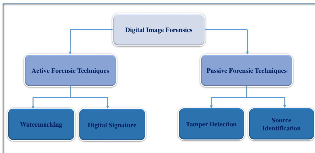
FIGURE 1.1: Hierarchy of digital image forensics.
