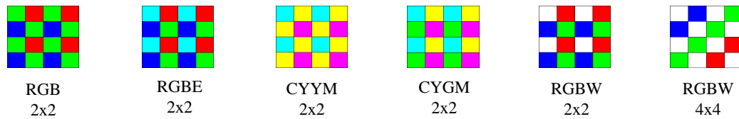
FIGURE 2.10: Color filter array patterns
