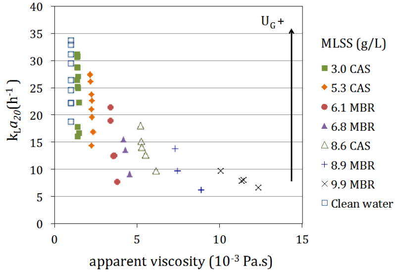
Figure VI.3. Coefficient k_L a_{20} vs. calculated apparent viscosity in the bubble column for different MLSS concentrations and two types of activated sludge - Fine bubble (FB) diffuser .
