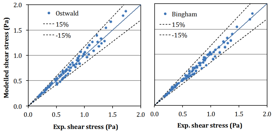
Figure IV.13. Comparison between experimental and predicted values of shear stress using the rheological models of Ostwald-de Waele and Bingham for the two sets of experimental rheograms, (i) and (ii), (using Equations IV.1 to IV.8 presented in Table IV.10).
