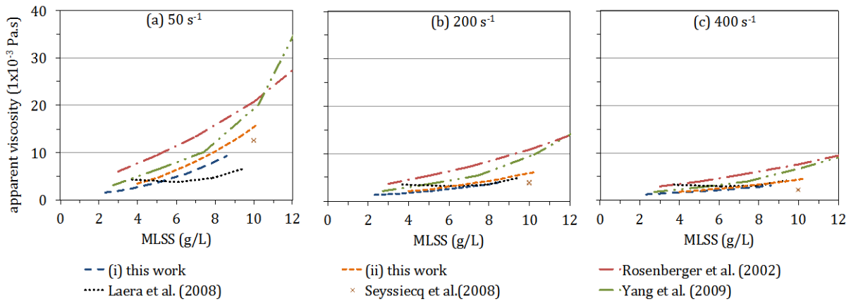
Figure IV.14. Apparent viscosity as a function of MLSS concentration at different shear rates (a) 50 s -1 , (b) 200 s -1 and (c) 400 s -1 for best fit in this work ((i) Eqs. IV.5 and IV.7; (ii) Eqs. IV.6 and IV.8) and other studies.
