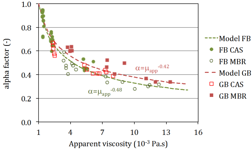
Figure VI.14. Alpha factor as a function of the apparent viscosity. Results and correlations obtained on site (CAS and MBR plants) and the fine and coarse bubbles diffusers.
