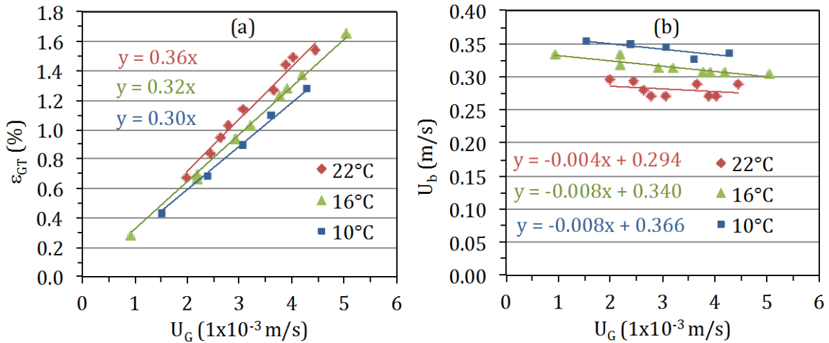
Figure V.1. (a) Overall gas hold-up and (b) average bubble rise velocity ( U_b ) obtained at a temperature of 10, 16 and 22°C in clean water in the bubble column at different superficial gas velocities ( U_G ) - FB diffuser.
