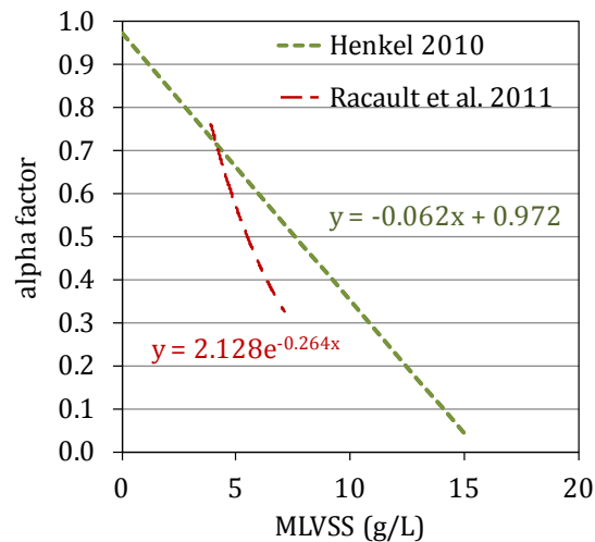
Figure I.8. Decrease of alpha factor with the increase of the MLVSS concentration according to two different models: Henkel (2010) and Racault et al. (2011).
