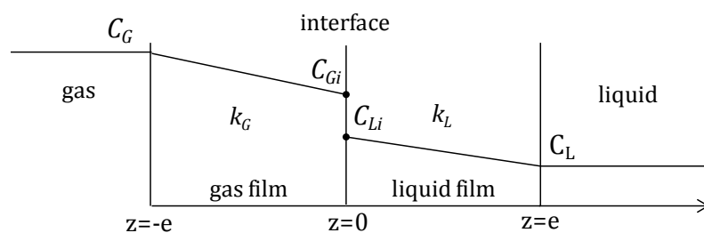
Figure I.2. Double film model (adapted from Roustan, 2003)
