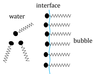
Figure I.9. Schematic of surfactants arrangement at a water-bubble interface.
