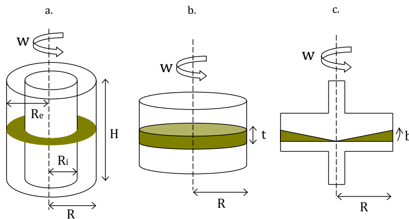
Figure I.15. Geometries of rotational rheometers: a. Concentric cylinder, b. Plate-plate, c. Cone-plate.
