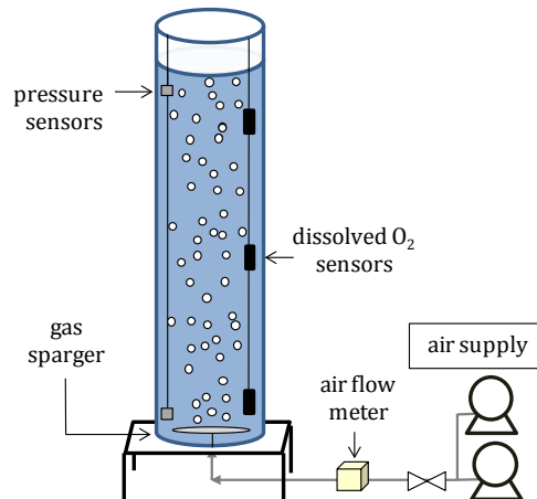
Figure II.1. Schematic of the bubble column used to measure the oxygen transfer in clean water and with activated sludge.
