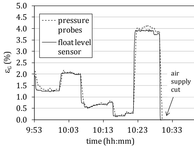
Figure II.8. Comparison of the gas hold-up ( \epsilon_G ) measured with the float level sensor and pressure probes.
