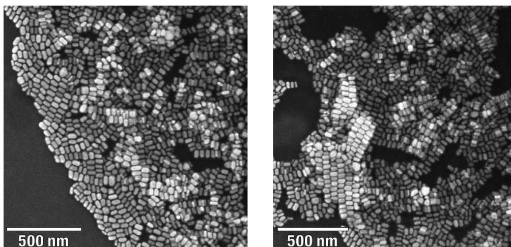
Figure 92. SEM micrographs of CTAB-stabilised AuNRs drop-casted on Si substrates from a water dispersion.
