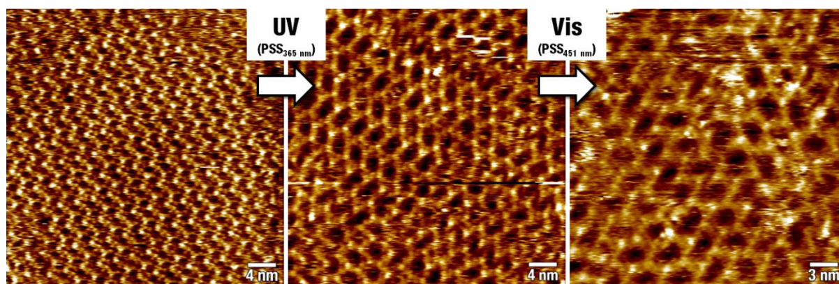
Figure 63. STM images of 1 recorded at the interface between an HOPG substrate and a 10 \mu M solution of 1 in 1-heptanoic acid. Left , no light irradiation (average tunnelling current ( I_T ) = 30 pA, tip bias voltage ( V_T ) = +800 mV). Centre , in-situ UV ( \lambda_{\max} = 365 nm) light irradiation ( I_T = 30 pA, V_T = +800 mV). Right , subsequent in-situ Vis ( \lambda_{\max} = 451 nm) light irradiation ( I_T = 20 pA, V_T = +800 mV).
