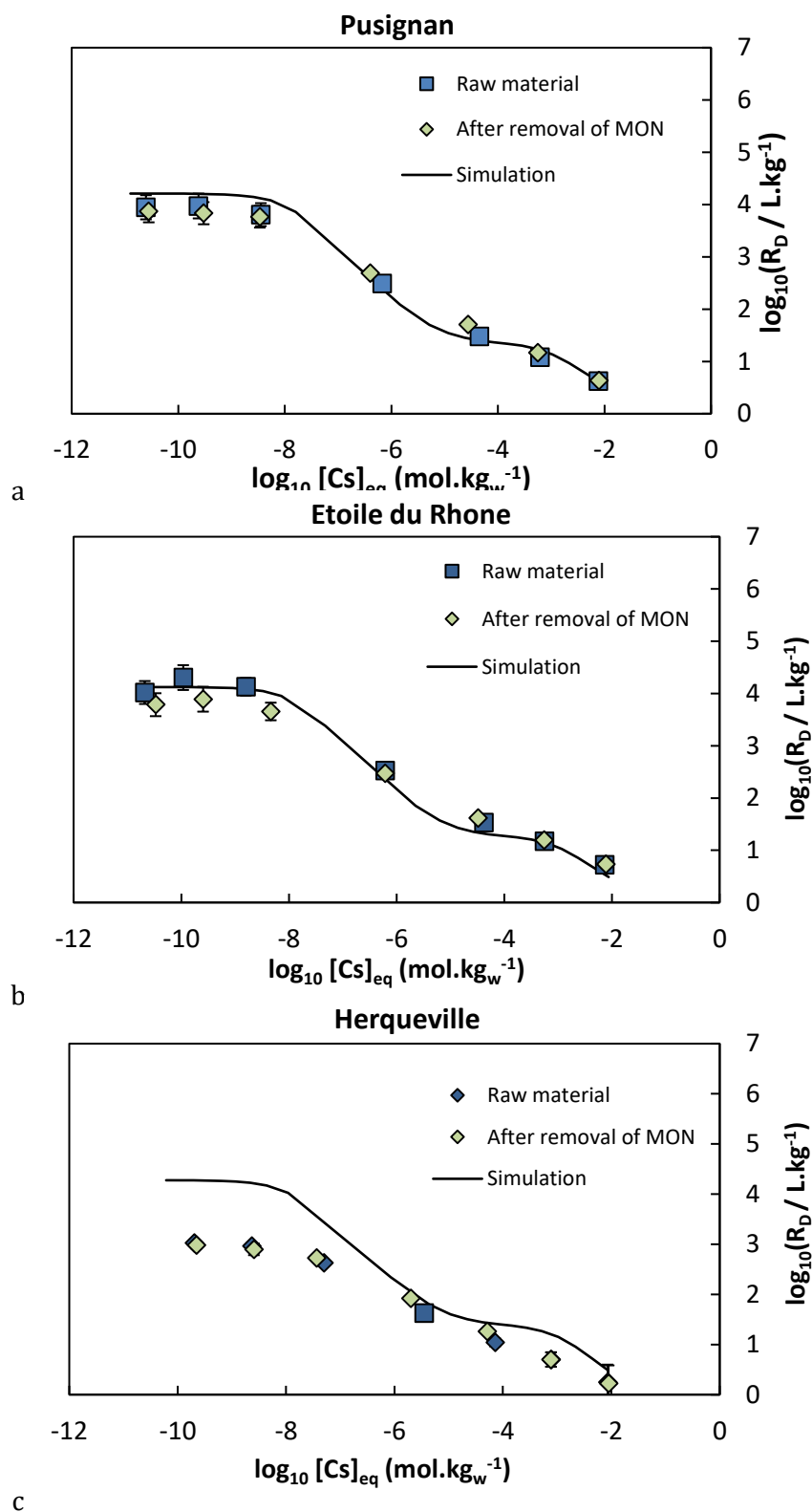
Figure IV. 6. Adsorption isotherms of Cs onto raw soil samples (squares) and after the removal of NOM (diamonds) at \text{pH}_{\text{water}}=6.5, 6.8 and 5.2 for Pusignan (a), Etoile-sur-Rhône (b), and Herqueville (c), respectively S/L = 0.05 \text{ kg.L}^{-1} and I = 0.1 \text{ mol.kg}_w^{-1} ( \text{CaCl}_2 ).
