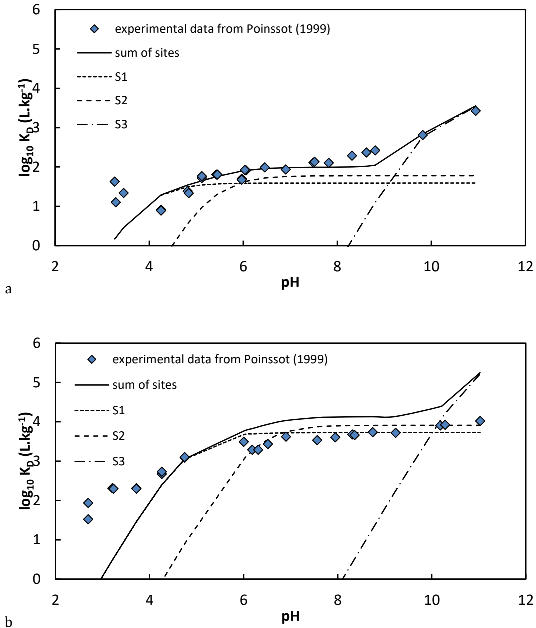
Figure III. 4. Adsorption isotherm in pH of Sr onto a Na-illite at [Sr]_i < 10^{-9} \text{ mol.kg}_w^{-1}t , a) I = 0.1 \text{ mol.kg}_w^{-1} and S/L \text{ ratio} = 1.78 \text{ g.L}^{-1} , and b) I = 0.01 \text{ mol.kg}_w^{-1} (NaClO 4 ), and S/L \text{ ratio} = 1.53 \text{ g.L}^{-1} and modelling with the multi-site ion-exchanger formalism.
