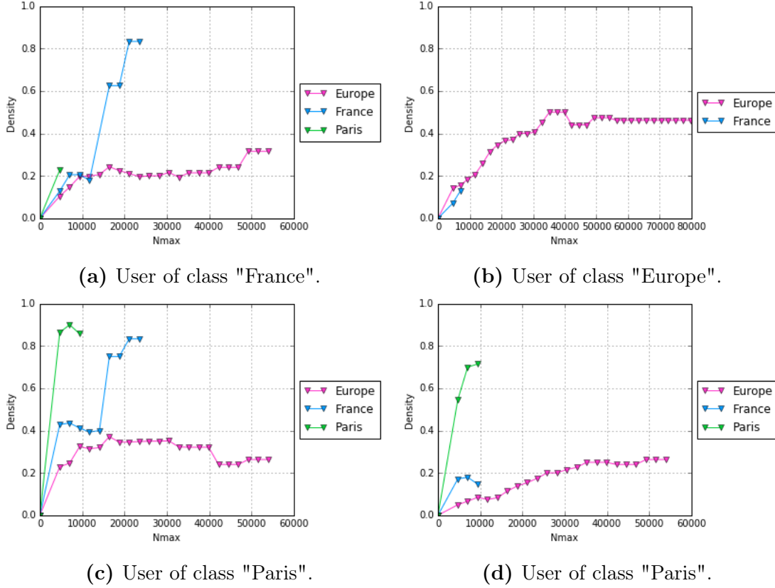
Figure 5.2: We represent the evolution of the density of the dataset for different users and for different values of N_{max} and three different geographical areas: Europe, France and Paris. We observe that each user has a peak of density depending on an optimal N_{max} which characterizes the class of the user.
