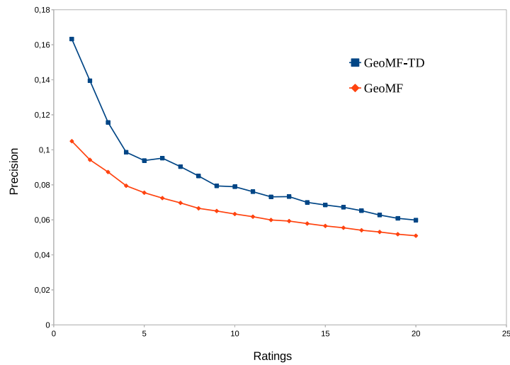
Figure 3.2: Precision comparison between GeoMF and GeoMF-TD
