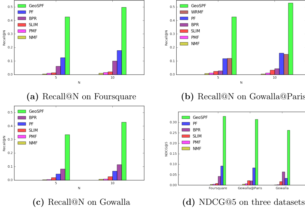
Figure 4.7: Performance comparison w.r.t. state-of-the-art approaches for three datasets: Foursquare, Gowalla@Paris and Gowalla. We plot Recall@N for N=5 and N=10 on Figures A.4a, A.4b and A.4c. We plot NDCG@5 on figure A.4d. We observe that GeoSPF outperforms significantly baselines on the three datasets for the three performance measures.
