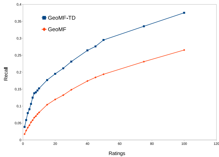
Figure 3.3: Recall comparison between GeoMF and GeoMF-TD
