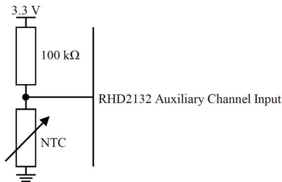
Fig. 7. Temperature measurement circuit diagram
