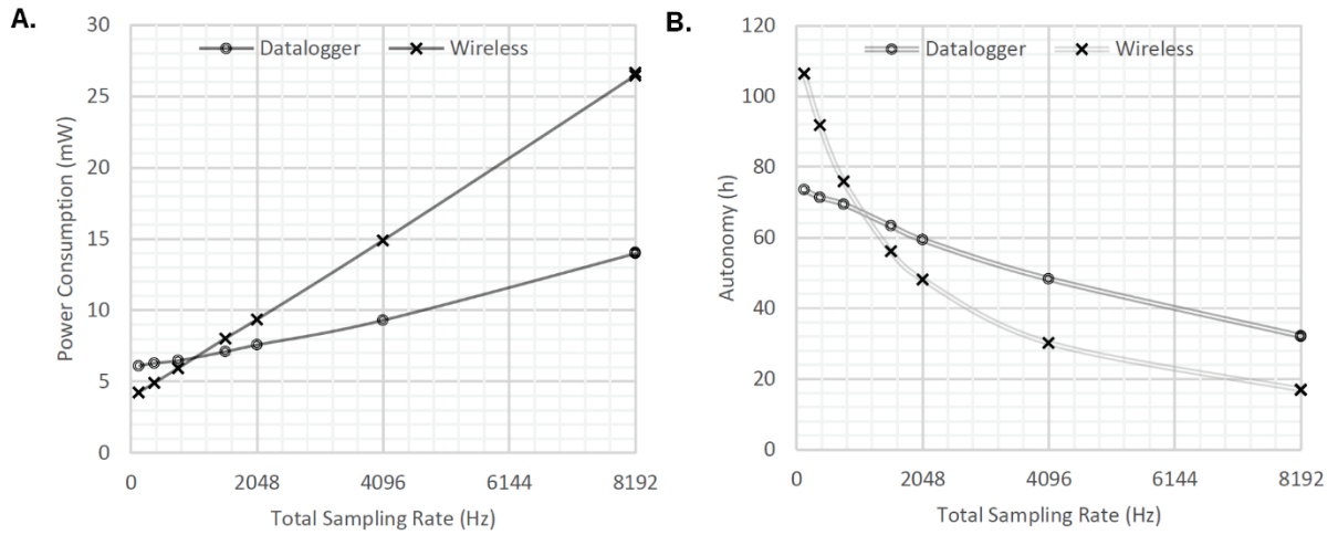
Fig. 8. Power consumption of the system with a 3V supply voltage and expected autonomy with a 150mAh primary battery.
