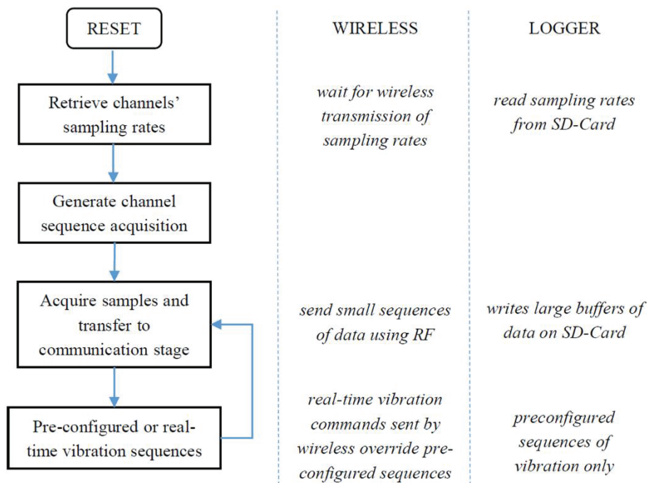
Fig. 5. Flowchart of the embedded software on the microcontroller unit
