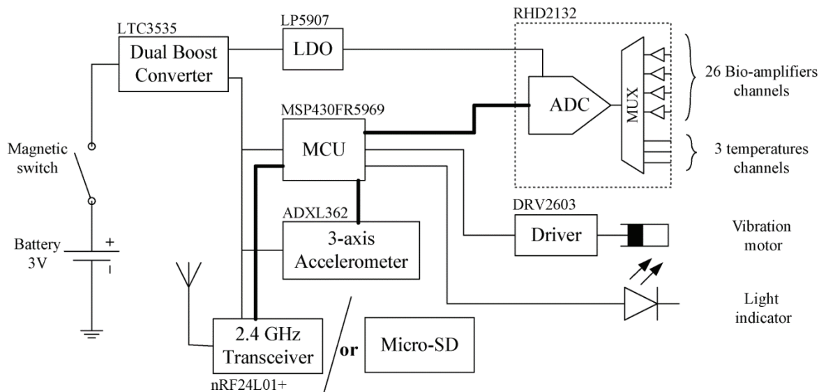
Fig. 4. Functional diagram of the complete instrumentation
