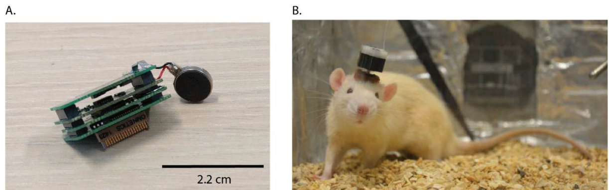
Fig. 2. A. Picture of the device showing the stack of boards with circular vibrating motor connected. B. Picture of a rat with the enclosed wireless device on its head.
