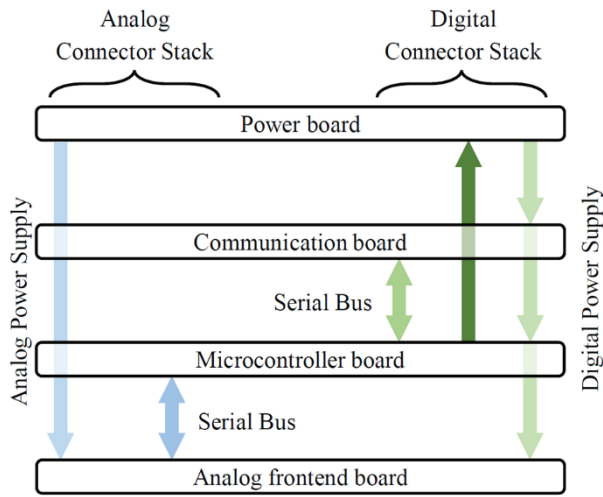
Fig. 3. Diagram of the interconnection between hardware modules
